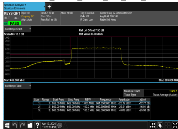
B2_N71(10M)_DFT-s- OFDM_QPSK_Outer_Full_Low_CH
