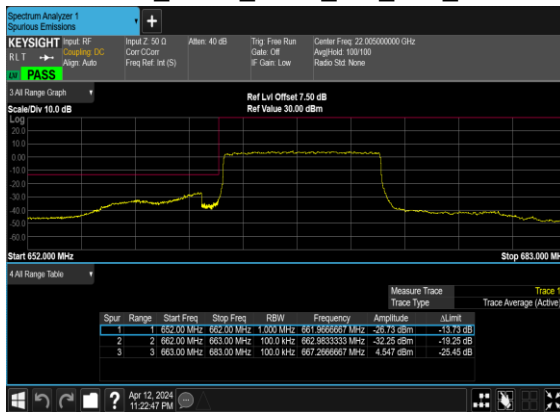
B2_N71(10M)_DFT-s- OFDM_BPSK_Outer_Full_Low_CH
