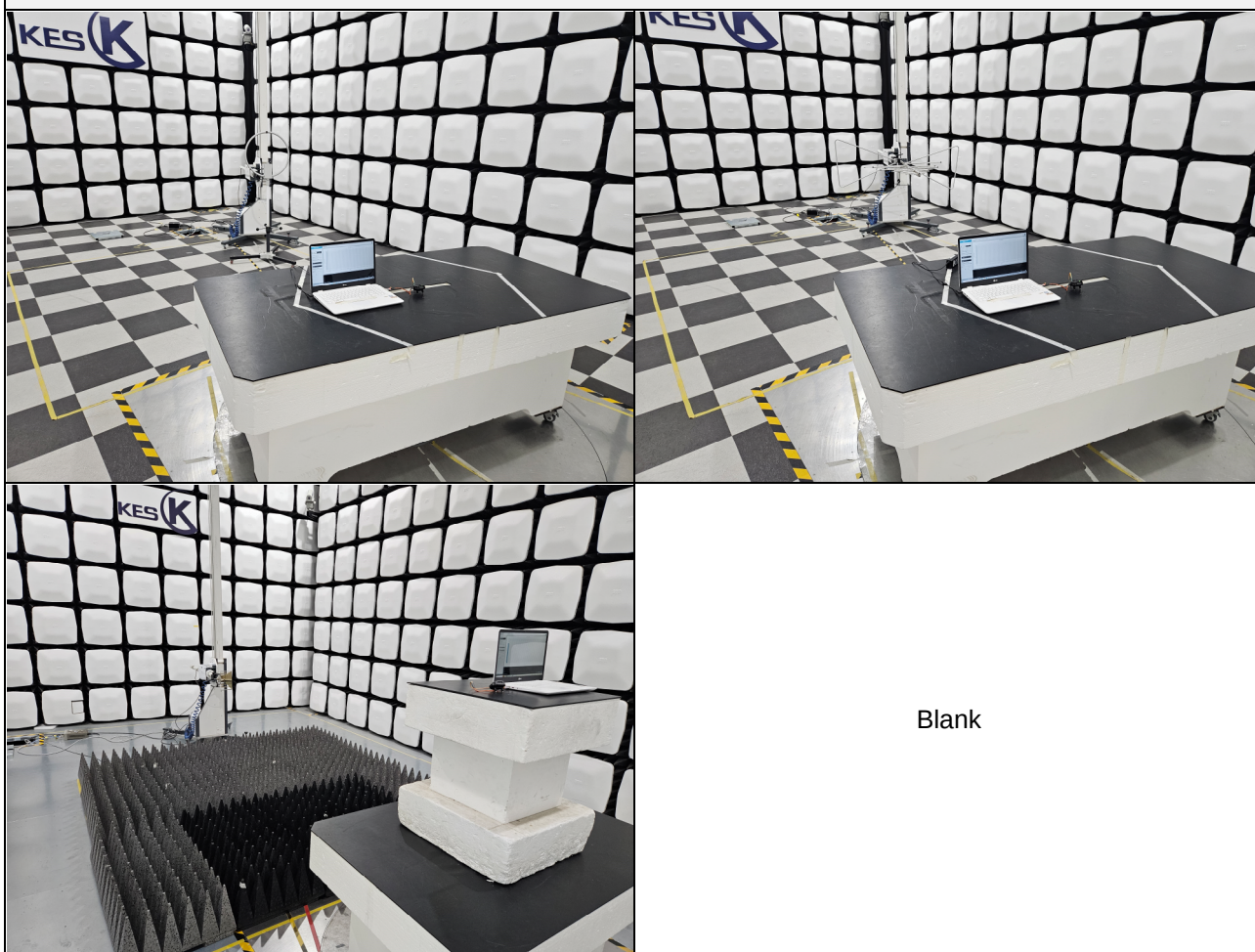
Radiated test
