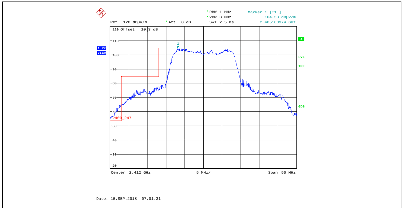
Plot 5.4.4.1.4.39. Band-Edge RF Radiated Emissions at 3 m, Vertical Polarization, Peak 18 Mbps QPSK, Power Setting 21, Channel 1, 2412 MHz
