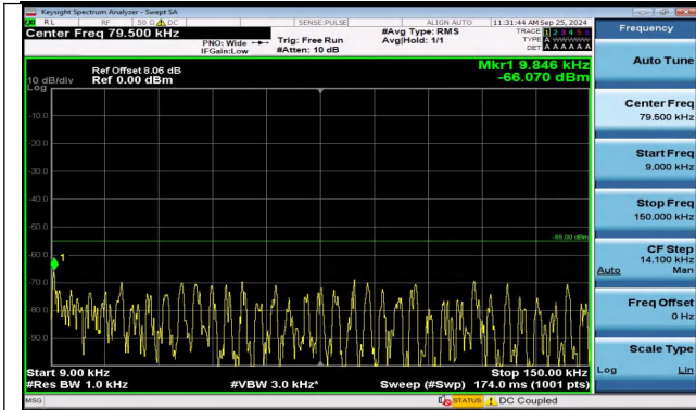
Band38_10MHz_QPSK_38200_1RB#0_0.009~0.15_0.009 ~0.15
