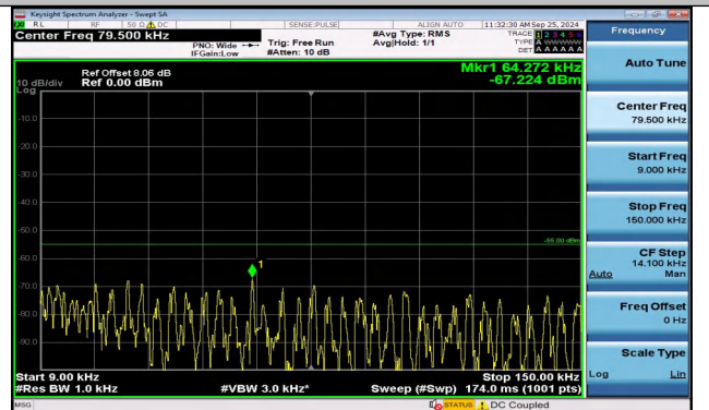
Band38_10MHz_16QAM_38200_1RB#0_0.009~0.15_0.00 9~0.15
