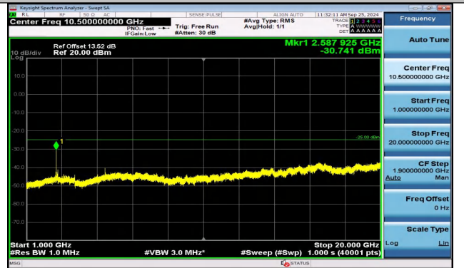
Band38_10MHz_QPSK_38200_1RB#0_1000~20000_100 0~20000
