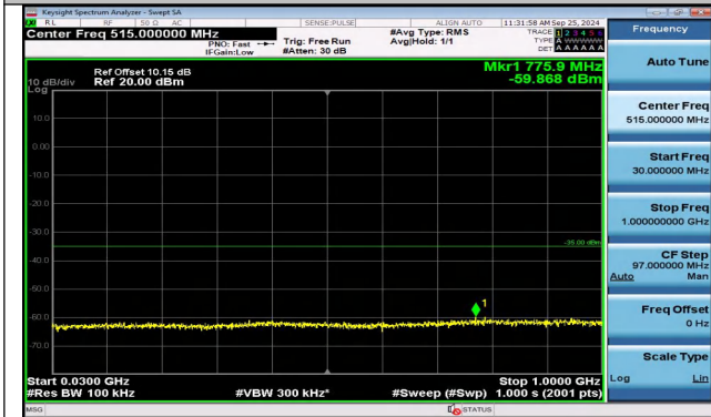
Band38_10MHz_QPSK_38200_1RB#0_30~1000_30~100 0
