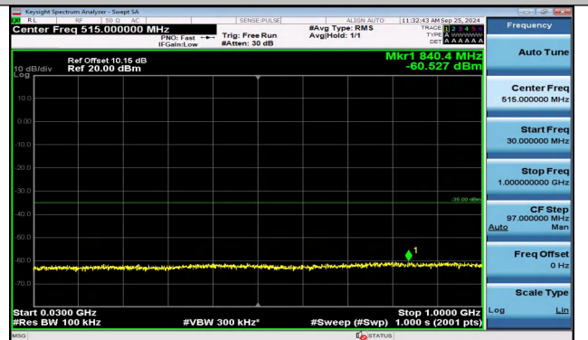
Band38_10MHz_16QAM_38200_1RB#0_30~1000_30~10 00
