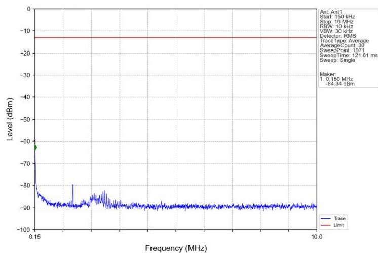
Band66_5MHz_QPSK_HCH_1777.5MHz_RB_1_0_NTV
