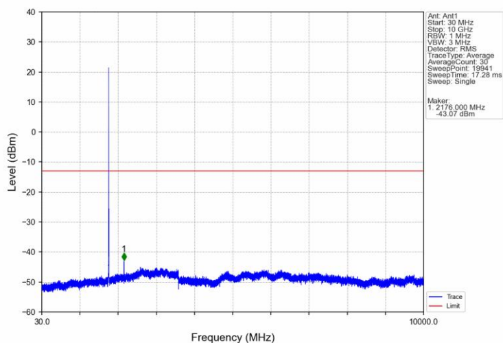
Band66 5MHz 16QAM HCH 1777.5MHz RB 1 0 NTVN
