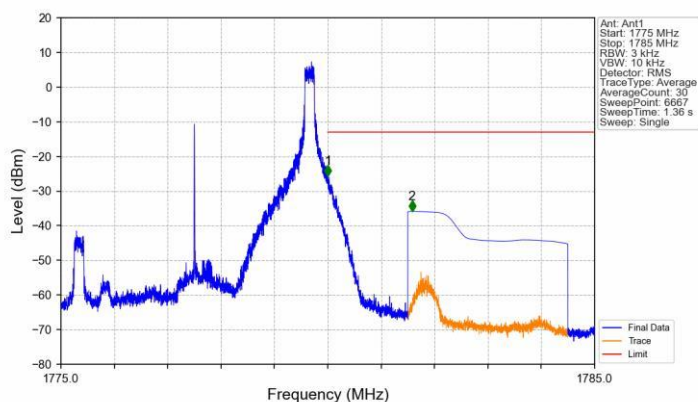
Band66 5MHz 16QAM HCH 1777.5MHz RB 1 24 NTN
