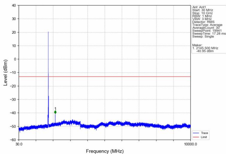
Band66 10MHz 16QAM MCH 1745MHz RB 1 0 NTV
