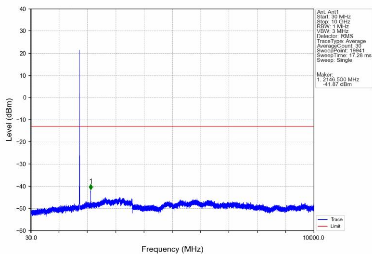
Band66 5MHz 16QAM MCH 1745MHz RB 1 0 NTNV
