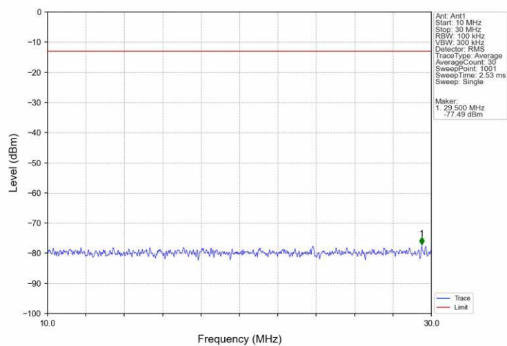
Band66_5MHz_QPSK_HCH_1777.5MHz_RB_1_0_NTV
