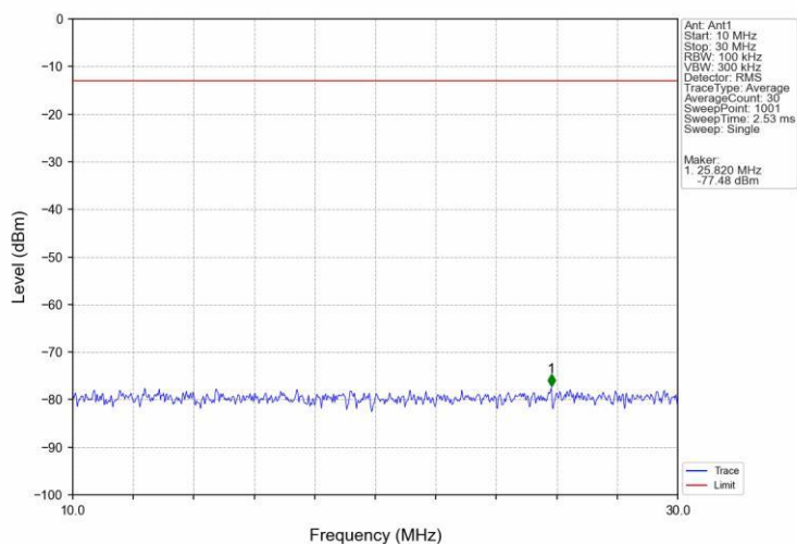
Band66 15MHz QPSK HCH 1772.5MHz RB 1 0 NTNV
