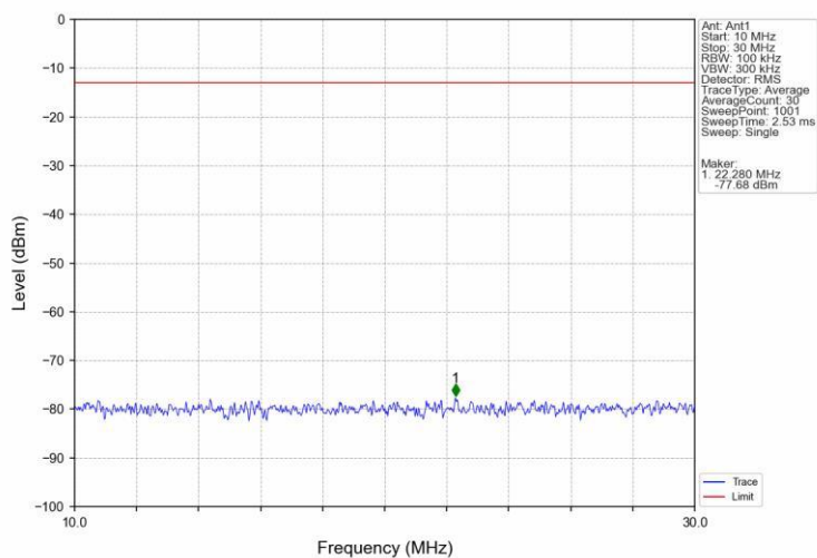
Band66 10MHz 16QAM HCH 1775MHz RB 1 0 NTV
