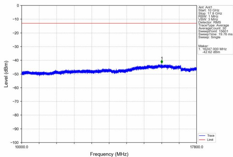
Band66 10MHz QPSK MCH 1745MHz RB 1 0 NTNV
