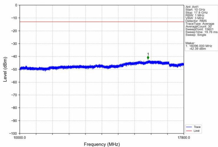
Band66 5MHz 16QAM HCH 1777.5MHz RB 1 0 NTVN
