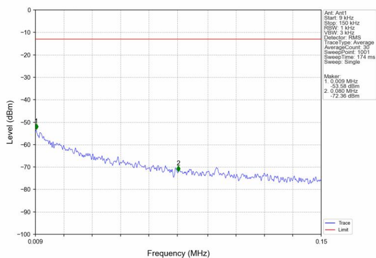
Band66 10MHz 16QAM HCH 1775MHz RB 1 0 NTNV
