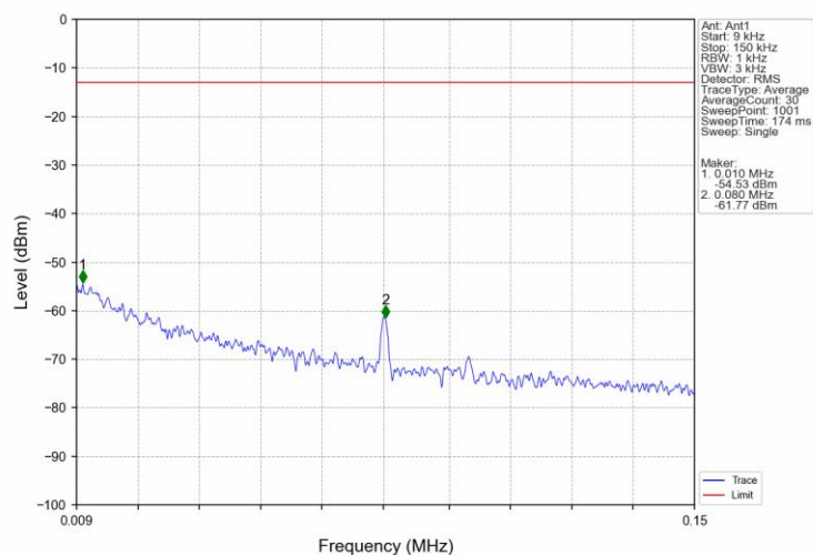
Band66 5MHz 16QAM LCH 1712.5MHz RB 1 0 NTNV
