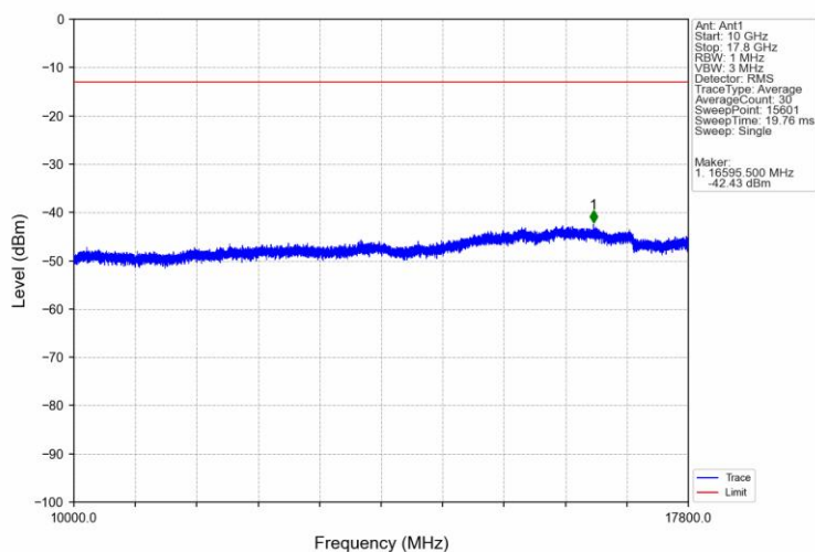
Band66 15MHz QPSK HCH 1772.5MHz RB 1 74 NTNV
