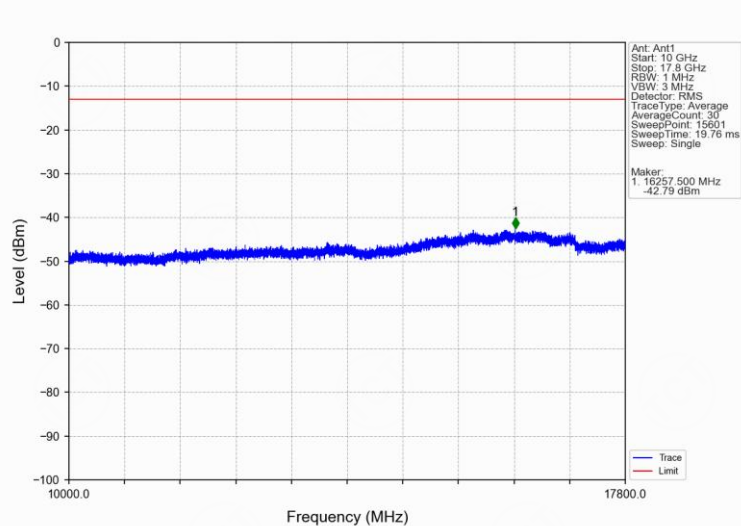
Band66 5MHz QPSK MCH 1745MHz RB 1 0 NTNV
