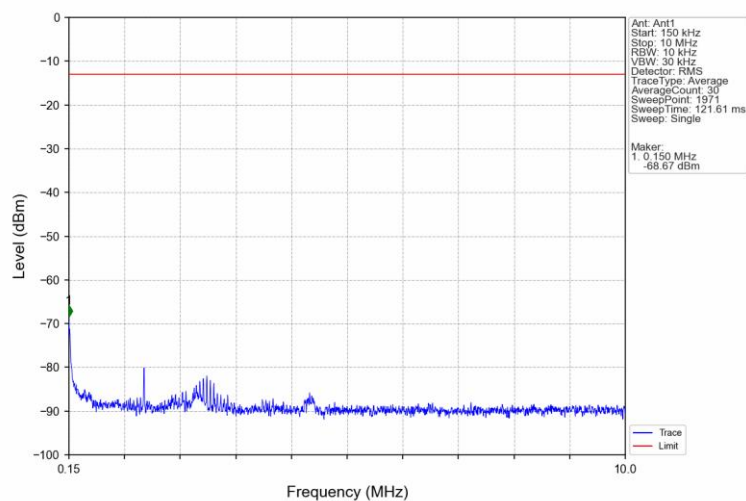
Band66 10MHz 16QAM MCH 1745MHz RB 1 0 NTV
