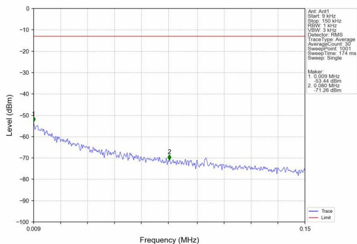
Band66 10MHz 16QAM MCH 1745MHz RB 1 0 NTV
