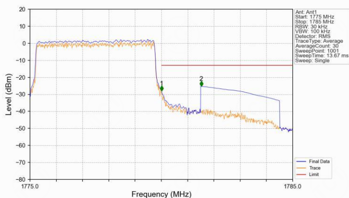
Band66 5MHz 16QAM HCH 1777.5MHz RB 25 0 NTN
