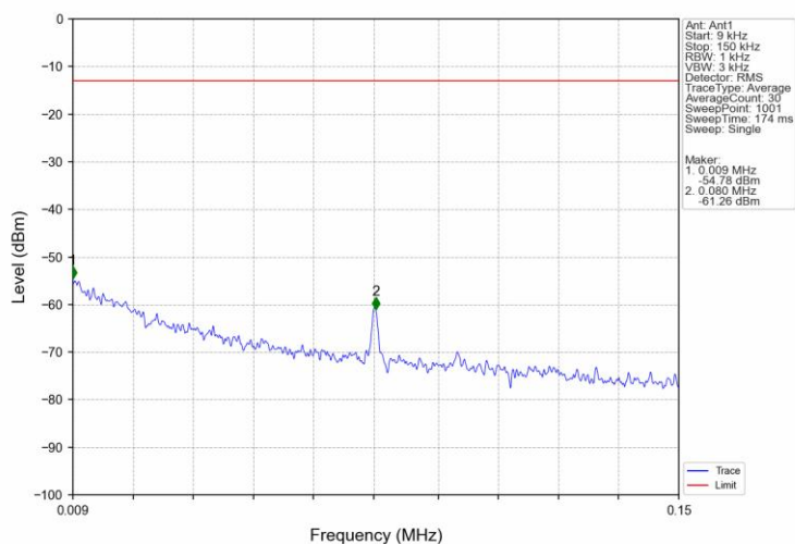
Band66 15MHz QPSK HCH 1772.5MHz RB 1 0 NTNV
