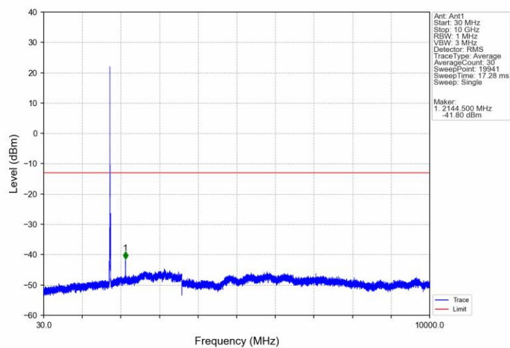
Band66 10MHz QPSK MCH 1745MHz RB 1 0 NTNV
