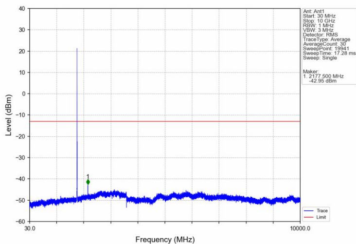
Band66_5MHz_QPSK_HCH_1777.5MHz_RB_1_0_NTV
