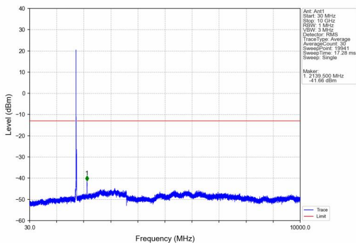
Band66 15MHz 16QAM MCH 1745MHz RB 1 0 NTV
