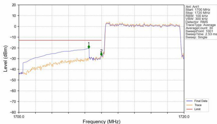
Band66 10MHz 16QAM LCH 1715MHz RB 50 0 NTV
