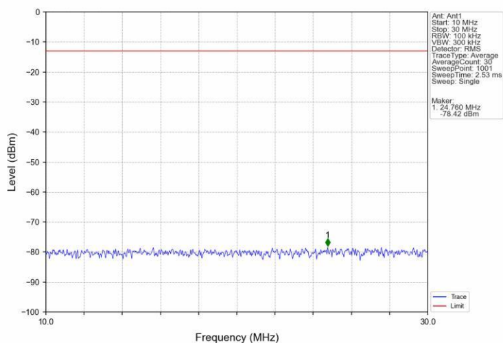
Band66 15MHz 16QAM MCH 1745MHz RB 1 0 NTV
