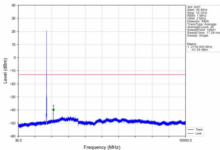
Band66 10MHz 16QAM LCH 1715MHz RB 1 0 NTV
