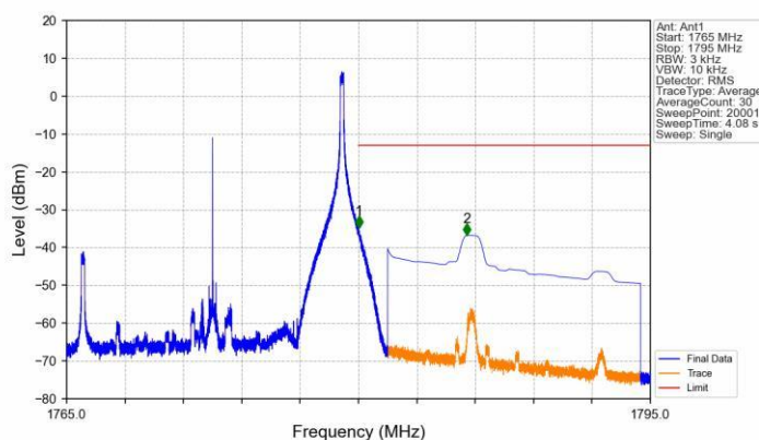
Band66 15MHz QPSK HCH 1772.5MHz RB 1 74 NTNV
