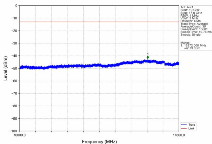
Band66 10MHz 16QAM HCH 1775MHz RB 1 0 NTNV
