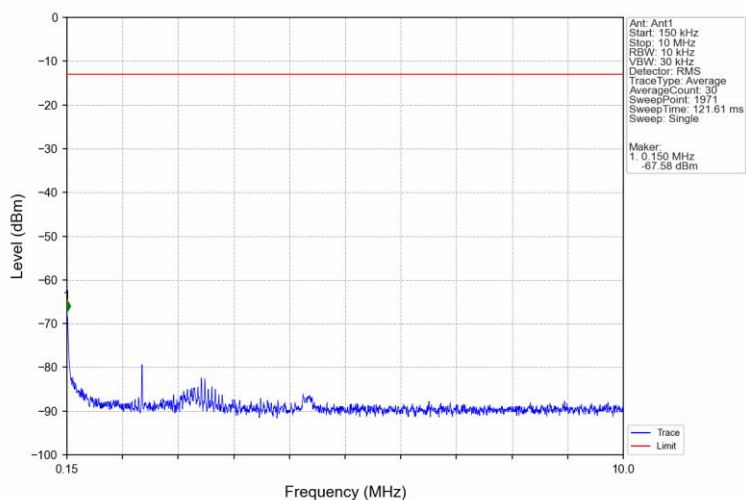
Band66 10MHz 16QAM HCH 1775MHz RB 1 0 NTV
