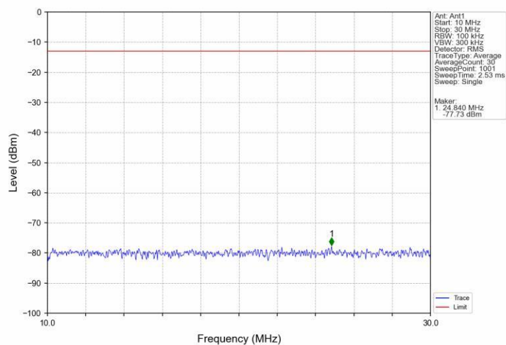
Band66 5MHz 16QAM HCH 1777.5MHz RB 1 0 NTV
