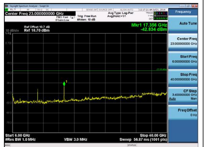
CUE-802.11a-5785M-chain2(6GHz-40GHz)
