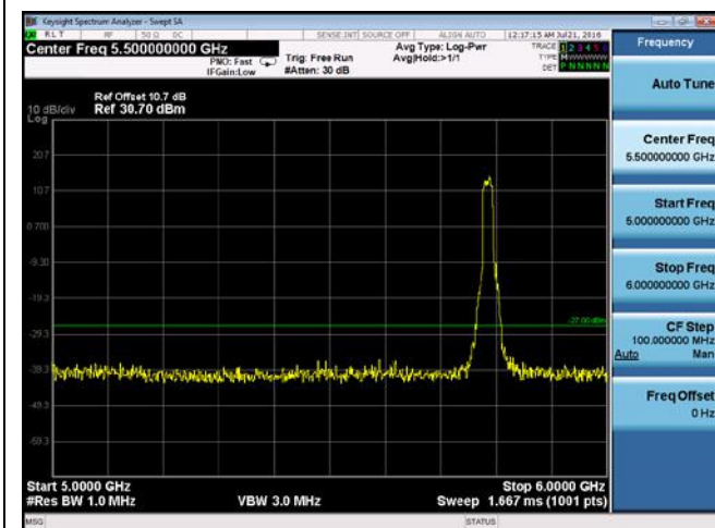
CUE-802.11a-5785M-chain2(5GHz-6GHz)
