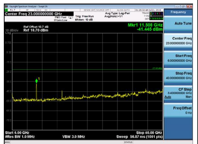
CUE-802.11n-40-5755M -chain3(6GHz-40GHz)
