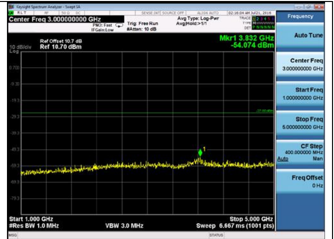
CUE-802.11n-40-5755M-chain4(1GHz-5GHz)
