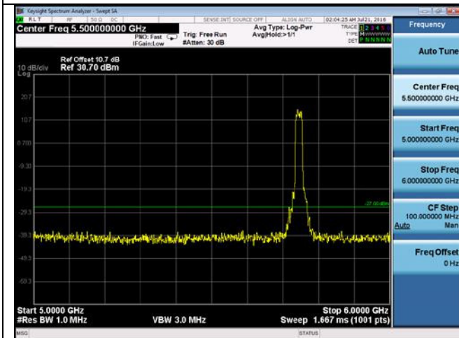
CUE-802.11n-20-5745M-chain4(5GHz-6GHz)
