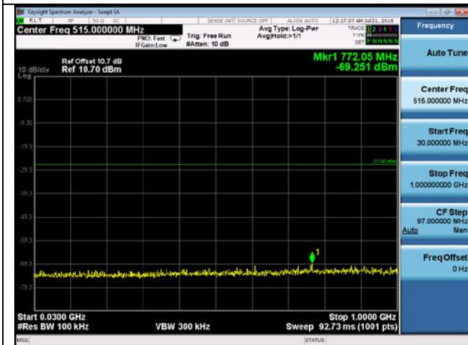
CUE-802.11a-5785M-chain2(30MHz-1GHz)
