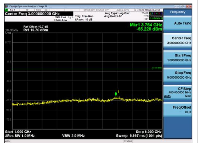
CUE-802.11n-20-5785M-chain1(1GHz-5GHz)
