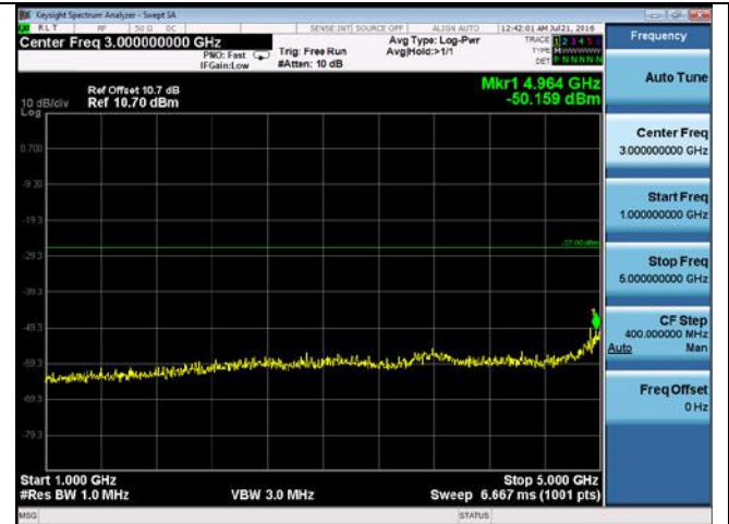
CUE-802.11ac-80-5210M -chain 2(1GHz-5GHz)
