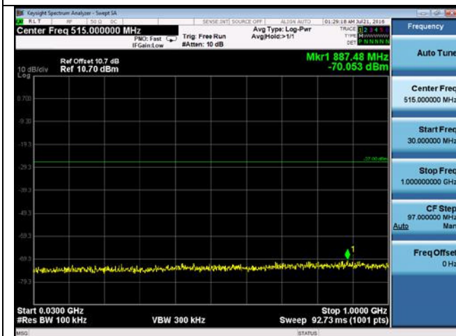
CUE-802.11n-40-5755M -chain3(30MHz-1GHz)
