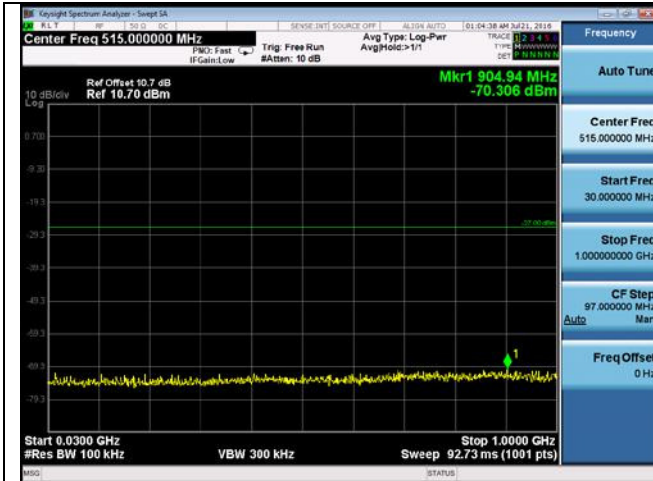
CUE-802.11a-5785M-chain3(30MHz-1GHz)
