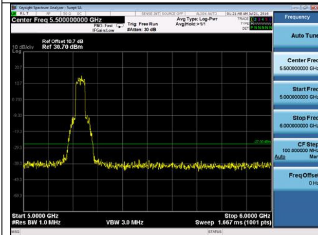
CUE-802.11n-40-5230M chain3(5GHz-6GHz)
