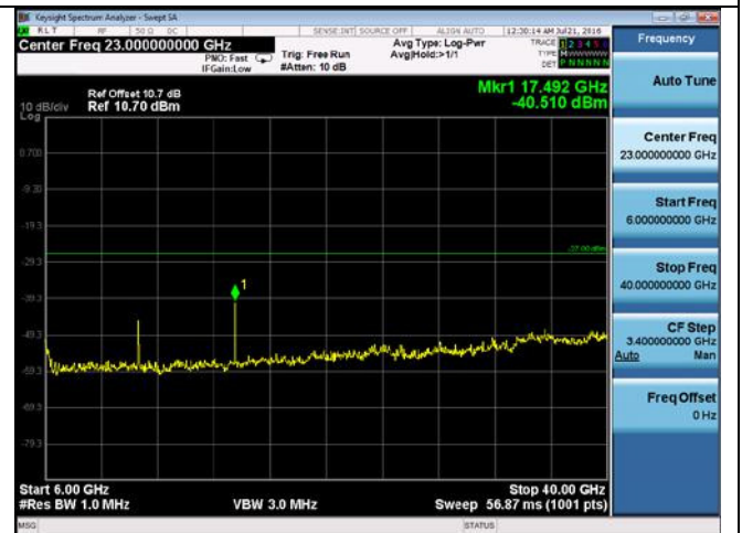
CUE-802.11n-20-5825M chain 2(6GHz-40GHz)
