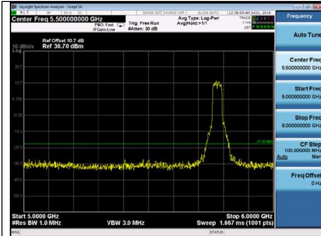
CUE-802.11n-40-5755M -chain2(5GHz-6GHz)
