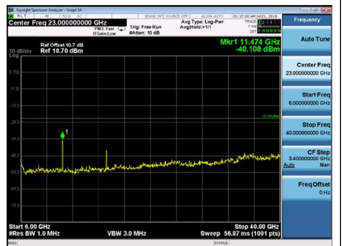
CUE-802.11n-20-5745M chain3(6GHz-40GHz)
