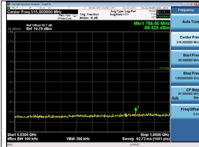
CUE-802.11n-40-5230M -chain3(30MHz-1GHz)
