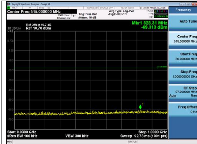
CUE-802.11a-5745M-chain1(30MHz-1GHz)
