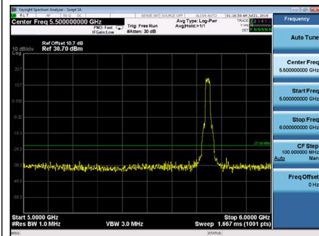
CUE-802.11n-20-5745M -chain3(5GHz-6GHz)
