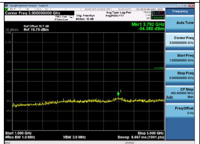
CUE-802.11n-40-5755M -chain3(1GHz-5GHz)
