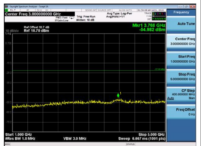
CUE-802.11a-5785M-chain4(1GHz-5GHz)
