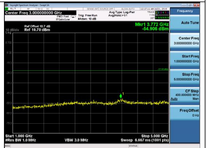
CUE-802.11a-5785M-chain2(1GHz-5GHz)
