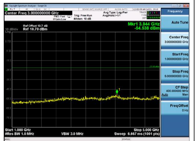
CUE-802.11n-40-5795M-chain1(1GHz-5GHz)
