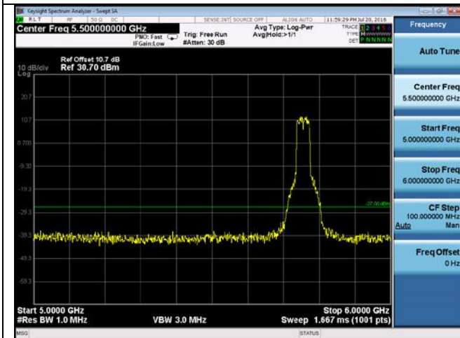
CUE-802.11n-40-5755M-chain1(5GHz-6GHz)
