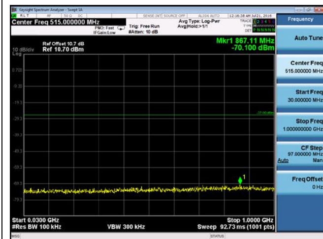
CUE-802.11a-5745M-chain2(30MHz-1GHz)
