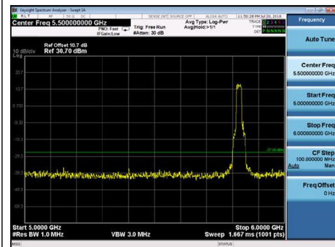
CUE-802.11n-20-5825M -chain 1(5GHz-6GHz)
