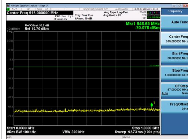
CUE-802.11n-40-5795M-chain1(30MHz-1GHz)
