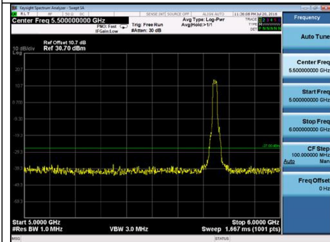
CUE-802.11a-5745M-chain1(5GHz-6GHz)
