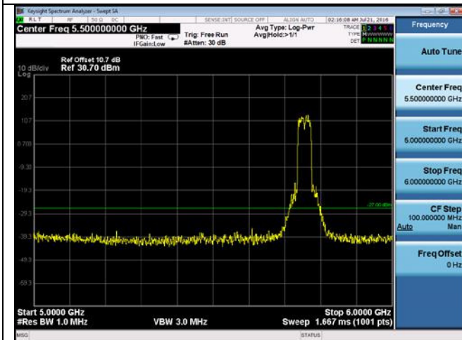
CUE-802.11n-40-5755M-chain4(5GHz-6GHz)
