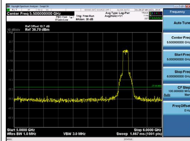
CUE-802.11n-40-5755M -chain3(5GHz-6GHz)
