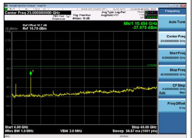
CUE-802.11n-40-5230M -chain2(6GHz-40GHz)
