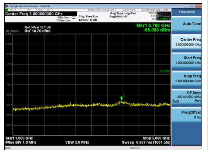
CUE-802.11a-5745M-chain2(1GHz-5GHz)
