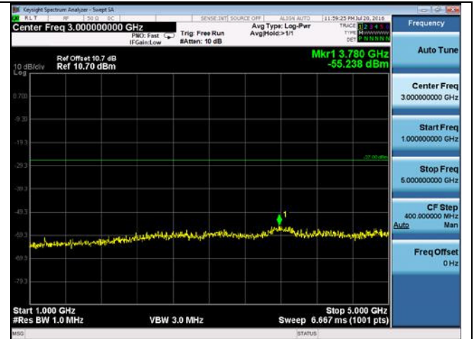
CUE-802.11n-40-5755M-chain1(1GHz-5GHz)
