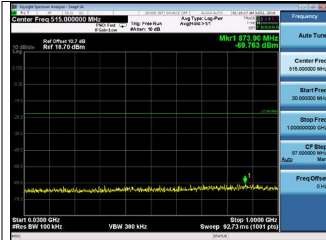
CUE-802.11n-20-5785M chain3(30MHz-1GHz)
