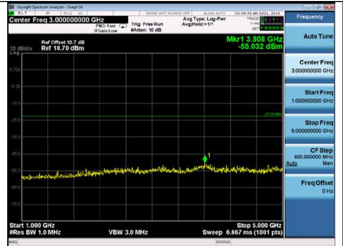
CUE-802.11a-5785M-chain3(1GHz-5GHz)
