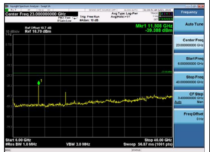
CUE-802.11a-5745M-chain3(6GHz-40GHz)
