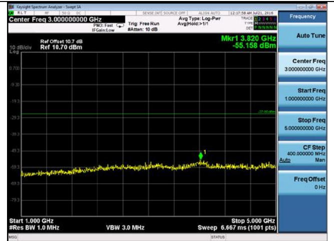
CUE-802.11a-5825M -chain 2(1GHz-5GHz)
