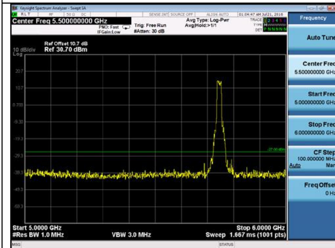
CUE-802.11a-5785M-chain3(5GHz-6GHz)
