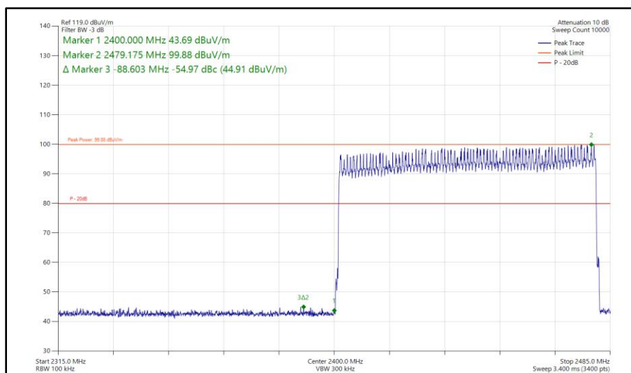
Figure 38 - Bluetooth 2-DH5, SISO, Core 0 - Hopping Band Edge Frequency 2400 MHz
