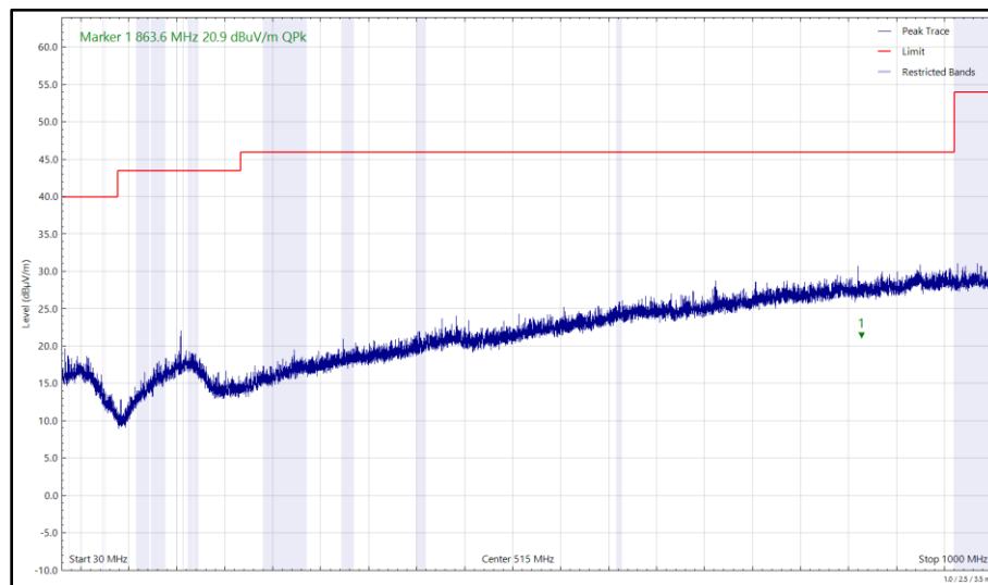
Figure 43 - 2441 MHz (CH39), DH5, iPA, Core 0, 30 MHz to 1 GHz, Horizontal (Peak)
