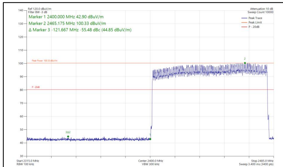
Figure 39 - Bluetooth 3-DH5, SISO, Core 0 - Hopping Band Edge Frequency 2400 MHz
