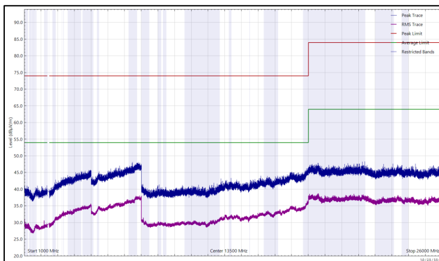
Figure 41 - 2402 MHz (CH0), DH5, iPA, Core 0, 1 GHz to 26 GHz, Horizontal
