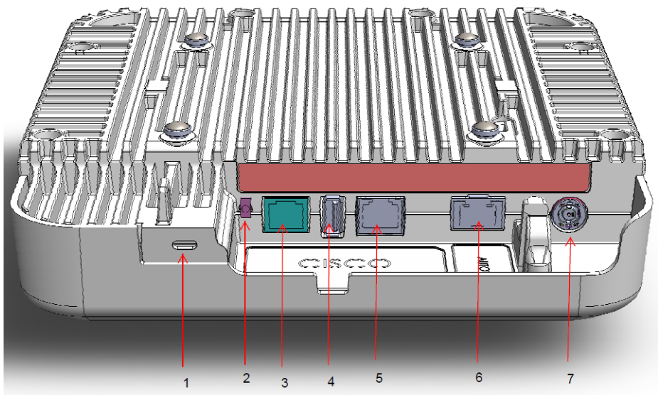
Figure 3 Access Point Ports and Connections on the Head - 2802E and 2802I Models
