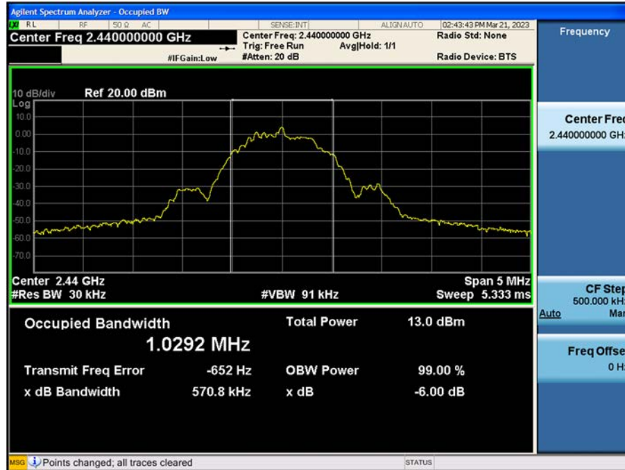
99 % & 6 dB Bandwidth plot (Mid-CH 19)
