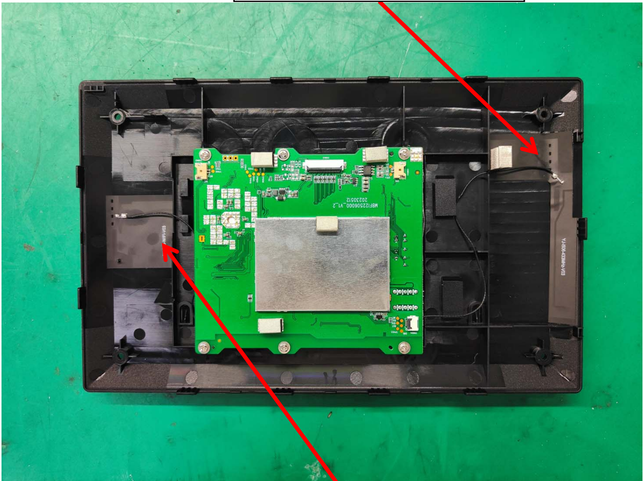
433MHz Antenna
