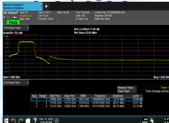
B2 1.4M 16QAM 6@0 CH 19193
