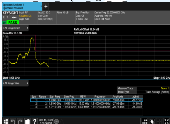
B2 1.4M 16QAM 1@5 CH 19193
