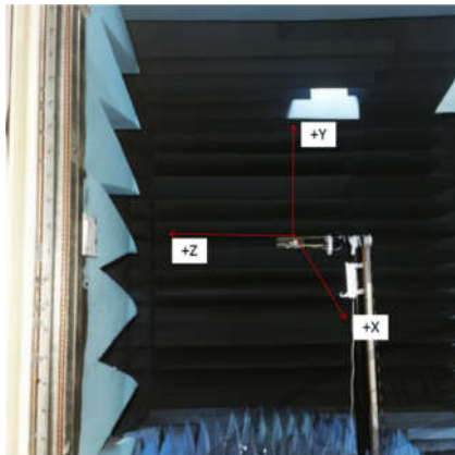
DUT photo in chamber
