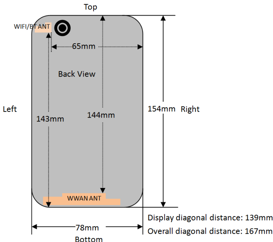
Fig.14.1 EUT Antenna Locations
