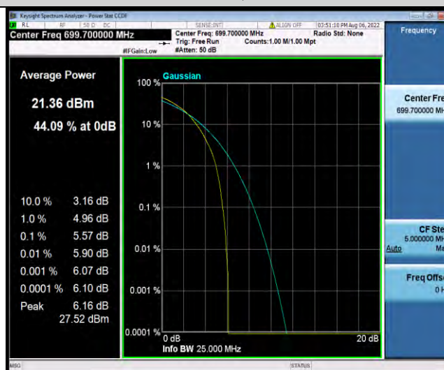
Band12-1.4MHz-64QAM-23095-1RB#0
