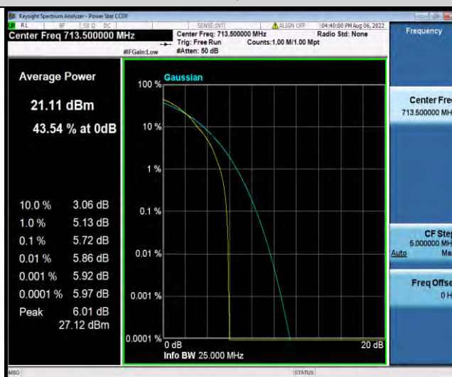
Band12-5MHz-64QAM-23155-25RB#0
