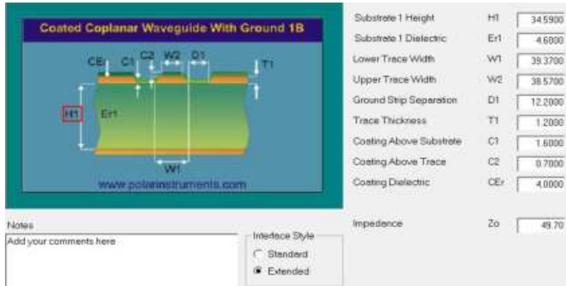
Figure 2: Grand referring to layer 4 Finished Copper, 39.37 mil
