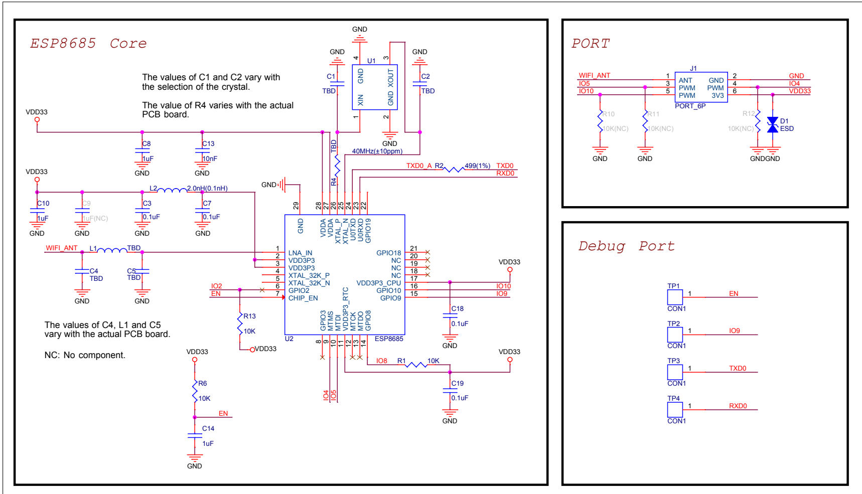
Figure 4: ESP8685-WROOM-07 Schematics
