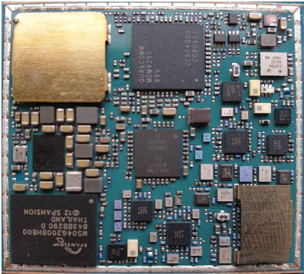
BOTTOM VIEW
