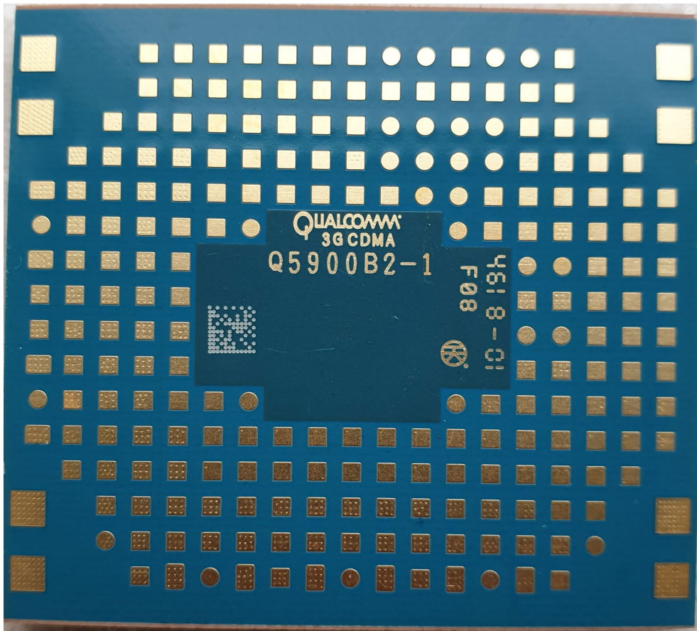
BOTTOM VIEW
