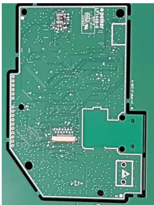
Main-Board, bottom and top view.
