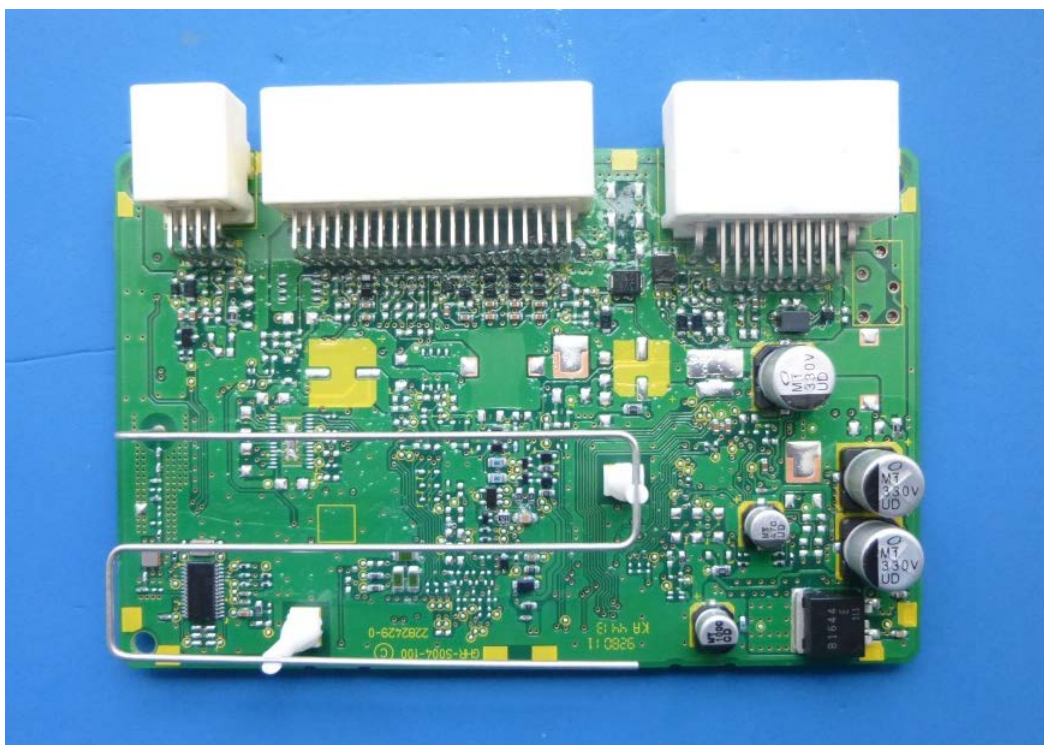
Figure 8.1 S54P0 PCB assy (top view)
