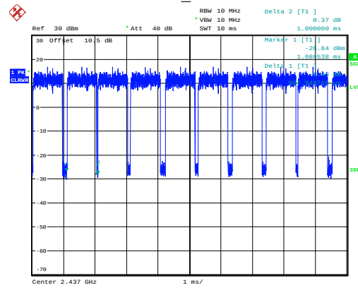
n40_2437MHz
