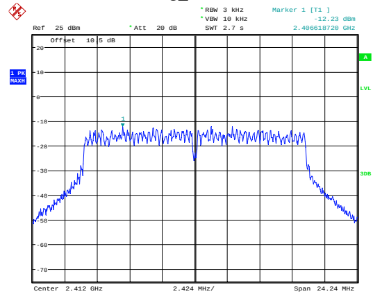
g_2412MHz
