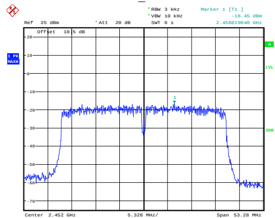
n40_2452MHz
