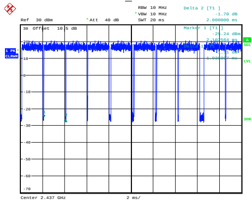
n20_2437MHz
