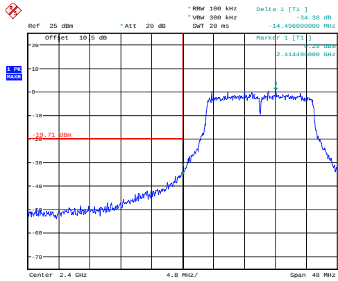
g_2412MHz
