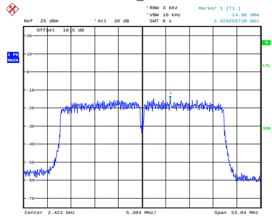
n40_2422MHz
