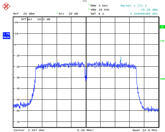
n40_2437MHz
