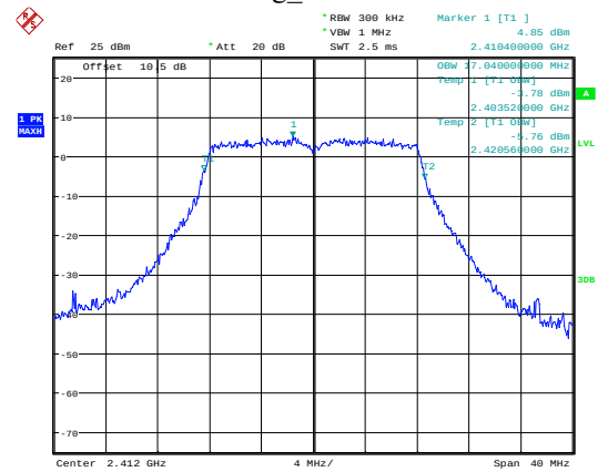
g_2412MHz
