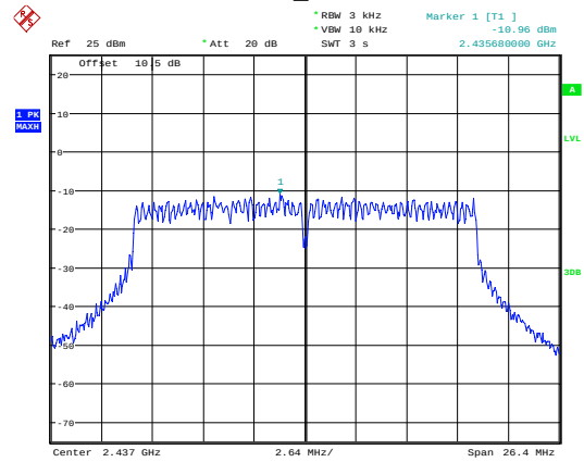
n20_2437MHz
