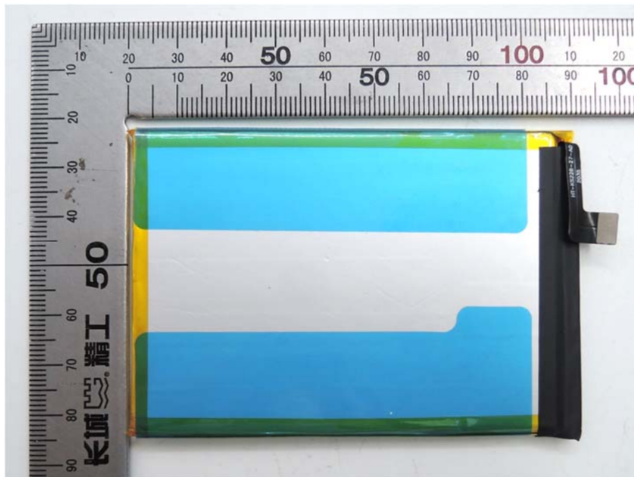
The battery view(ShenzhenAerospaceElectronicCo.,Ltd)
