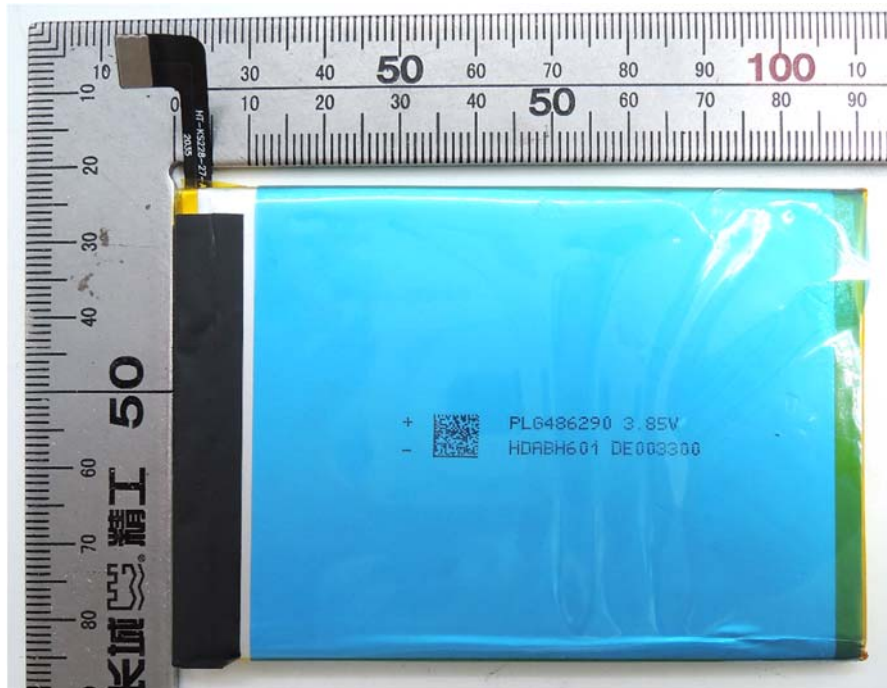
The battery view(DONGGUANG MILEY ElectronicCo.,Ltd)
