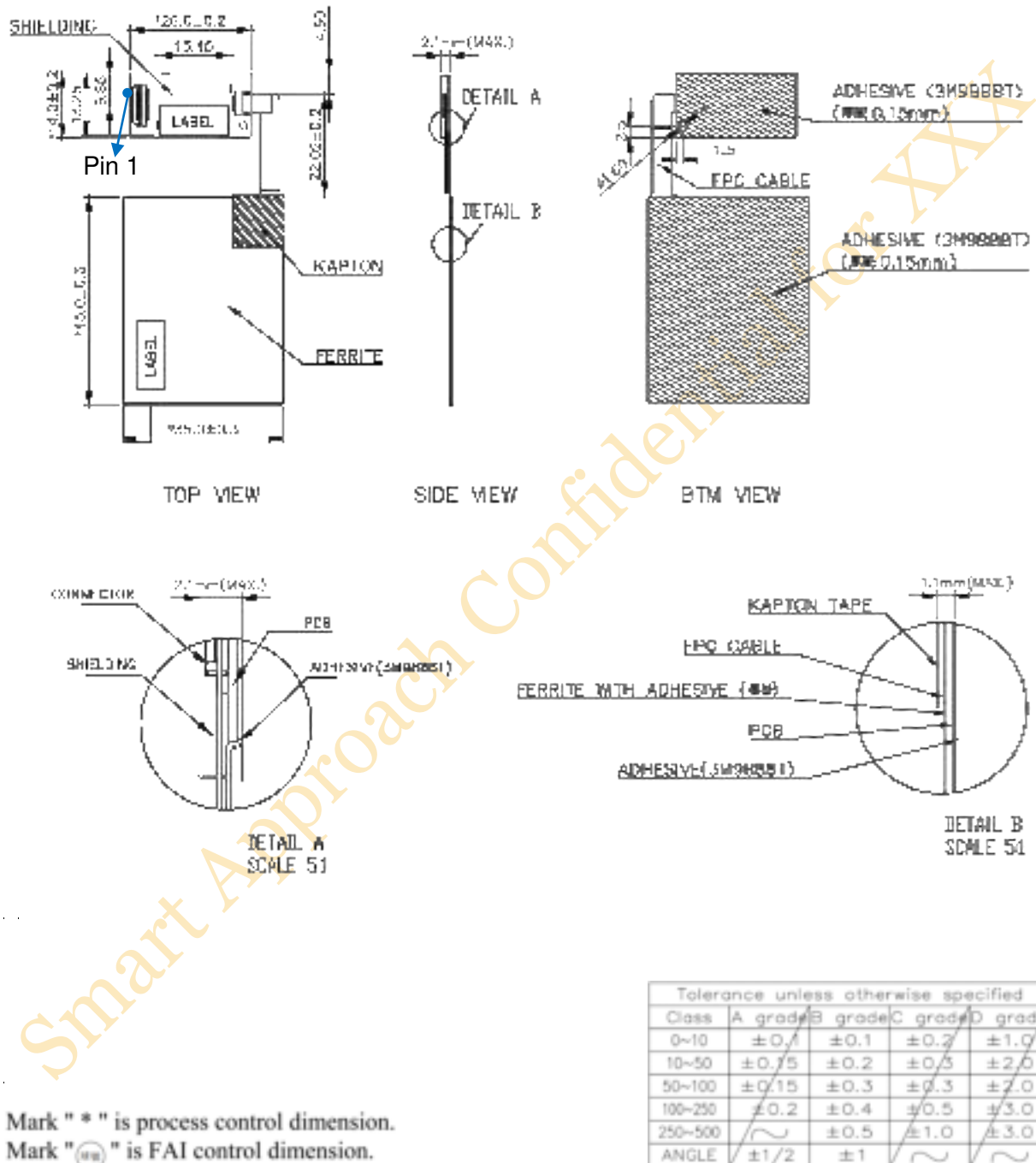
Figure 9 Antenna Module Drawing
