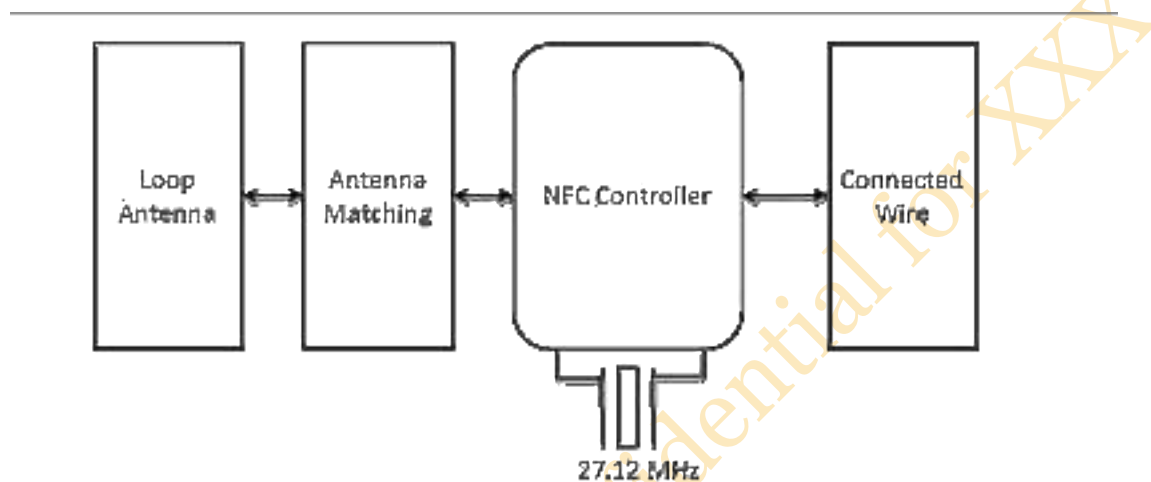
Figure 3 Module Block Diagram
