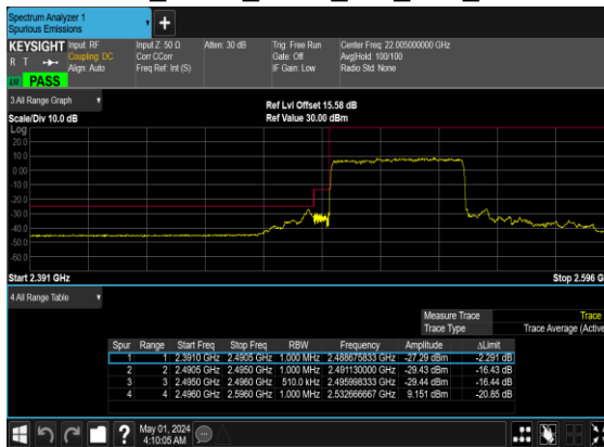
B2_N41(50M)_DFT-s- OFDM_BPSK_Outer_Full_Low_CH
