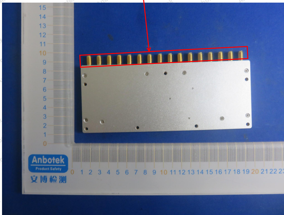
Ant Connector
