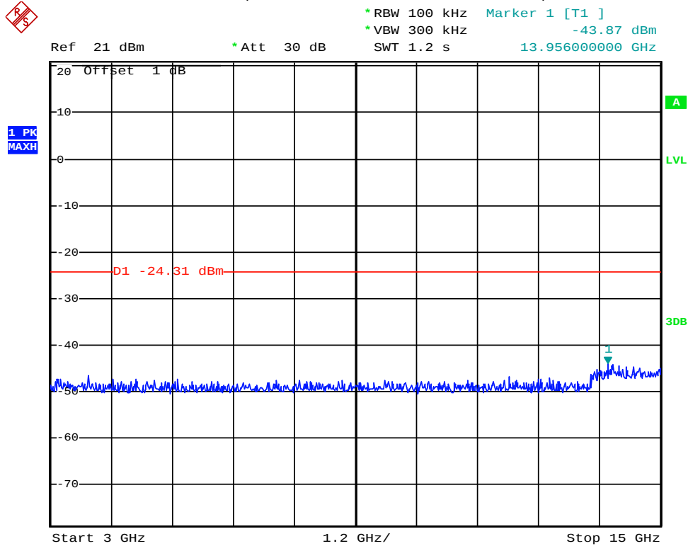
(Plot 4.7 C1: Channel 39: 2480MHz)
