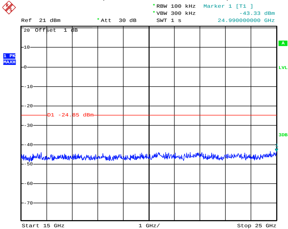
(Plot 4.7 B2: Channel 19: 2440MHz)
