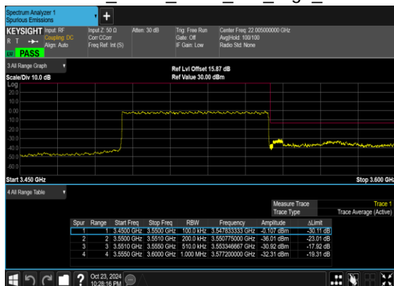
N78(60M)_DFT-s- OFDM_BPSK_Outer_Full_High_CH
