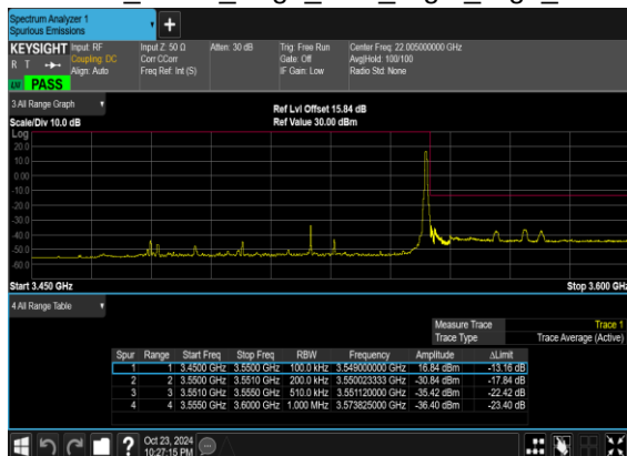
N78(60M)_DFT-s- OFDM_BPSK_Edge_1RB_Right_High_CH
