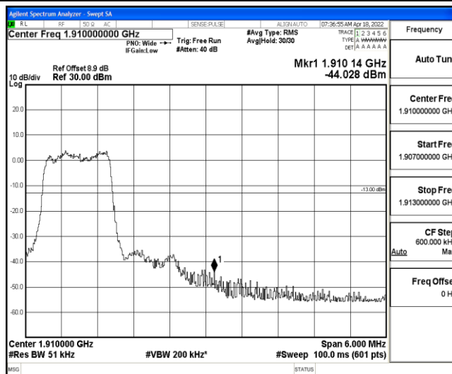
Band2-3MHz-16QAM-19185-6-0-Low--44.03-PASS
