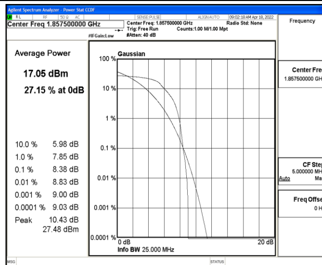
Band2-15MHz-QPSK-18675-6-0-Low-8.38-&lt;=13-PASS
