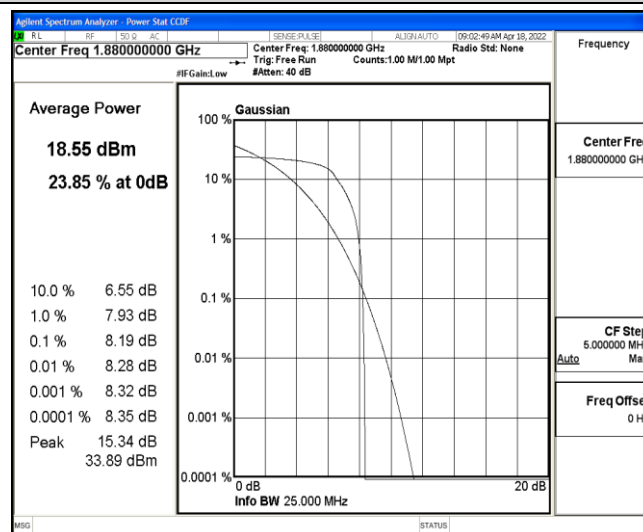
Band2-15MHz-16QAM-18900-6-0-Low-8.19-&lt;=13-PASS
