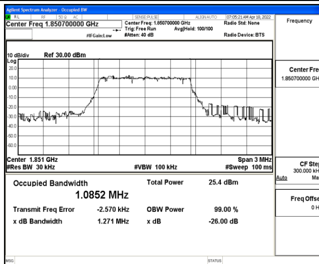
Band2-1.4MHz-16QAM-18607-6-0-Low-1.0852-1.271-PASS
