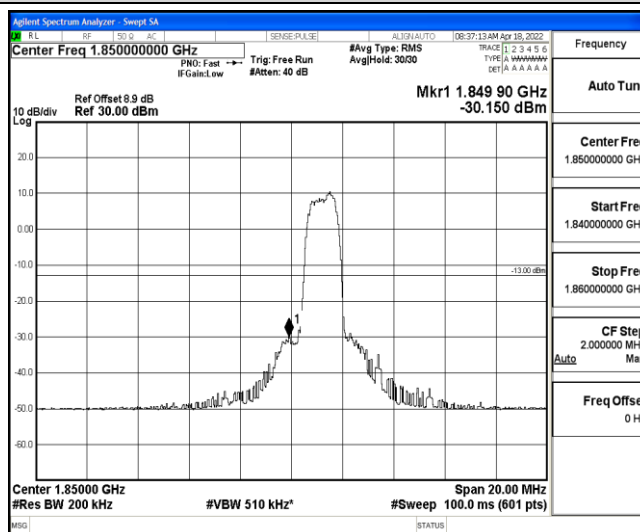
Band2-10MHz-16QAM-18650-6-0-Low--30.15-PASS
