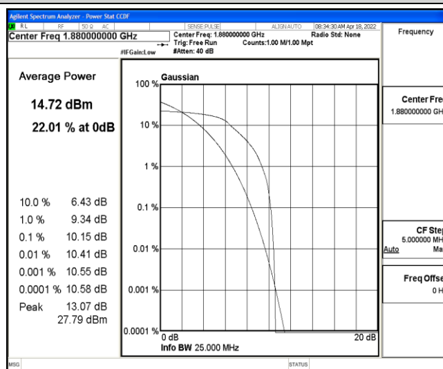
Band2-10MHz-QPSK-18900-6-0-Low-10.15-&lt;=13-PASS
