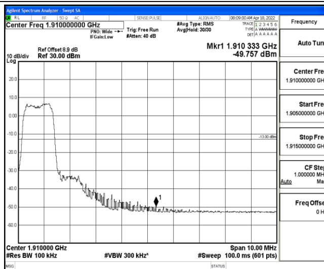
Band2-5MHz-QPSK-19175-6-0-Low--49.76-PASS
