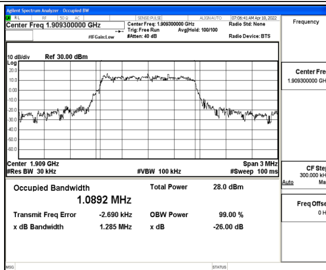
Band2-1.4MHz-16QAM-19193-6-0-High-1.0892-1.285-PASS
