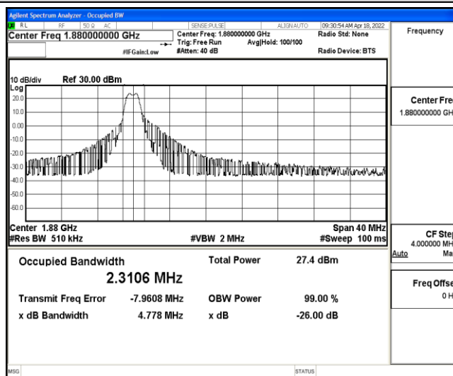
Band2-20MHz-QPSK-18900-6-0-Low-2.3106-4.778-PASS
