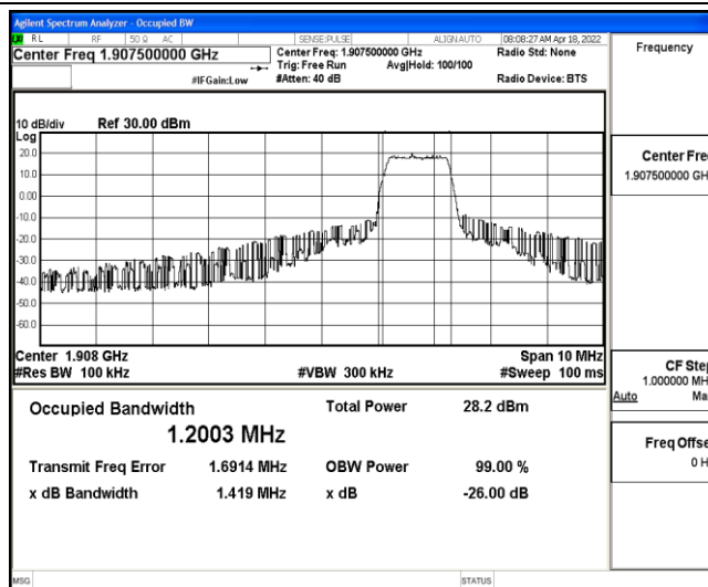
Band2-5MHz-16QAM-19175-6-0-High-1.2003-1.419-PASS
