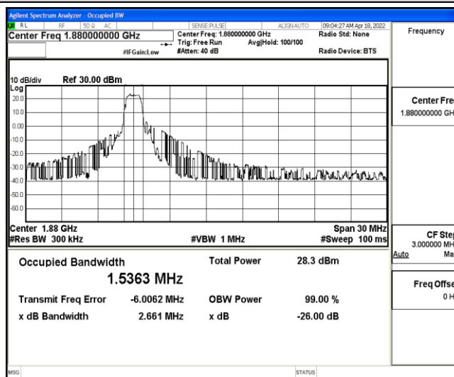
Band2-15MHz-16QAM-18900-6-0-Low-1.5363-2.661-PASS
