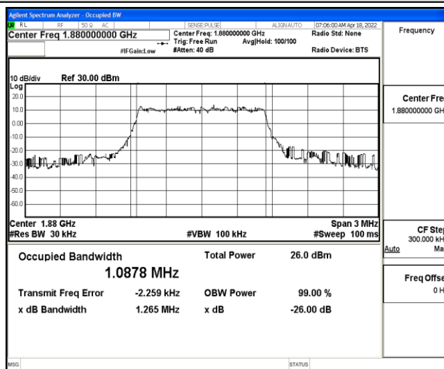
Band2-1.4MHz-16QAM-18900-6-0-Low-1.0878-1.265-PASS
