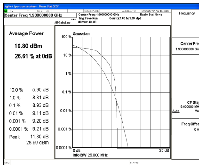
Band2-20MHz-QPSK-19100-6-0-Low-8.93-&lt;=13-PASS
