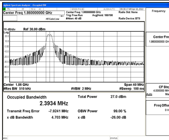
Band2-20MHz-QPSK-18700-6-0-Low-2.3934-4.703-PASS
