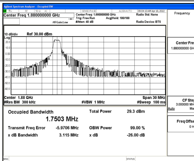
Band2-15MHz-QPSK-18900-6-0-Low-1.7503-3.115-PASS
