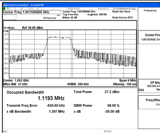
Band2-3MHz-16QAM-18615-6-0-Low-1.1193-1.397-PASS
