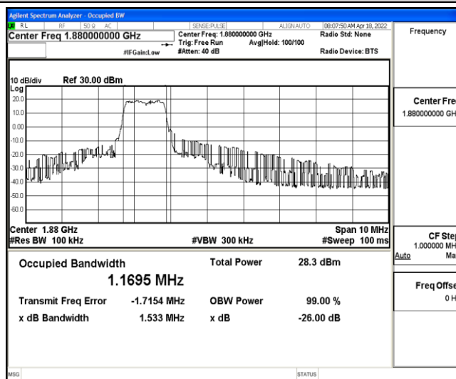
Band2-5MHz-16QAM-18900-6-0-Low-1.1695-1.533-PASS
