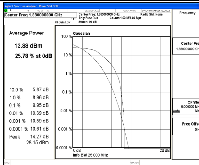
Band2-1.4MHz-QPSK-18900-6-0-Low-9.95-&lt;=13-PASS
