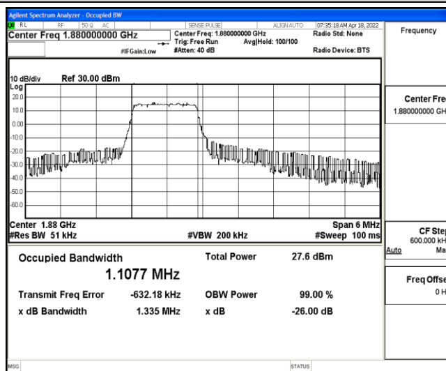
Band2-3MHz-QPSK-18900-6-0-Low-1.1077-1.335-PASS
