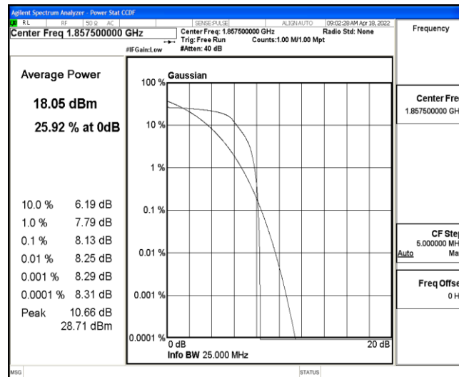
Band2-15MHz-16QAM-18675-6-0-Low-8.13-&lt;=13-PASS
