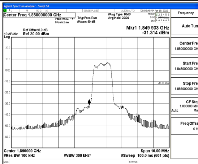
Band2-5MHz-16QAM-18625-6-0-Low--31.31-PASS
