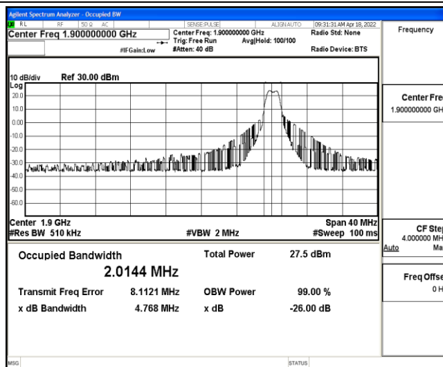
Band2-20MHz-QPSK-19100-6-0-High-2.0144-4.768-PASS
