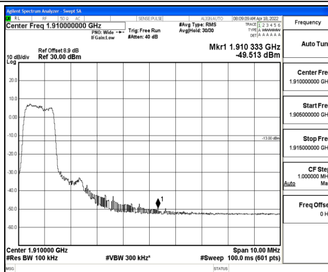
Band2-5MHz-16QAM-19175-6-0-Low--49.51-PASS
