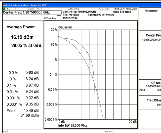
Band2-5MHz-QPSK-19175-6-0-Low-8.97-&lt;=13-PASS
