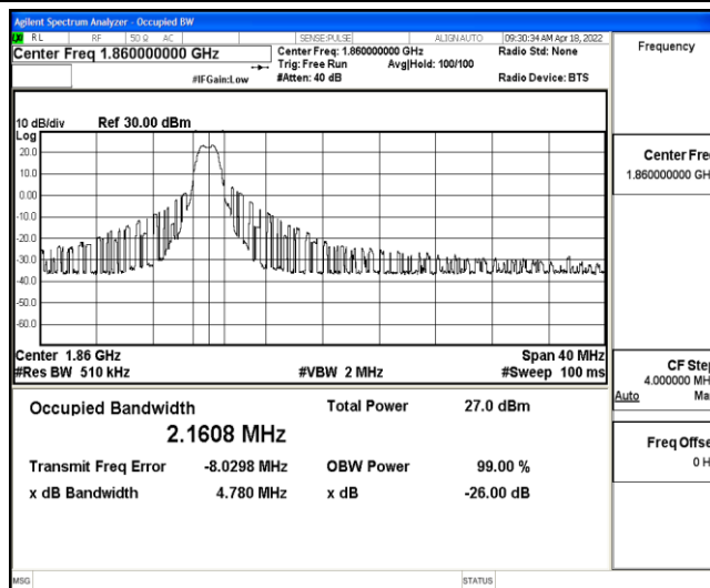
Band2-20MHz-16QAM-18700-6-0-Low-2.1608-4.780-PASS
