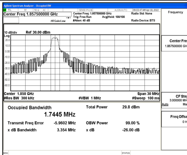
Band2-15MHz-16QAM-18675-6-0-Low-1.7445-3.354-PASS
