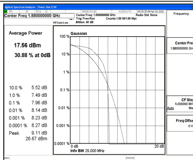
Band2-20MHz-16QAM-18900-6-0-Low-7.96-&lt;=13-PASS
