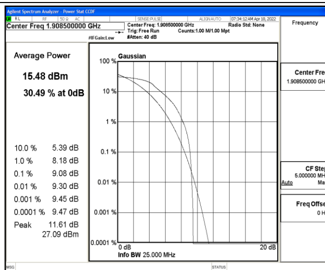
Band2-3MHz-QPSK-19185-6-0-Low-9.08-&lt;=13-PASS
