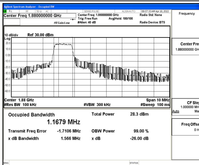
Band2-5MHz-QPSK-18900-6-0-Low-1.1679-1.566-PASS
