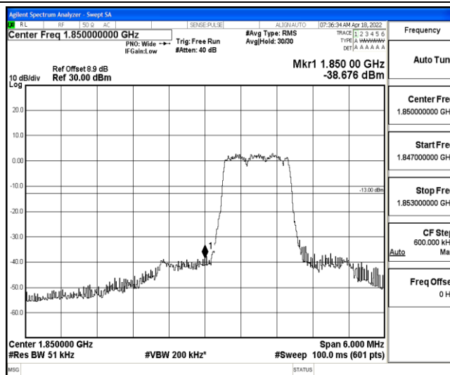
Band2-3MHz-16QAM-18615-6-0-Low--38.68-PASS
