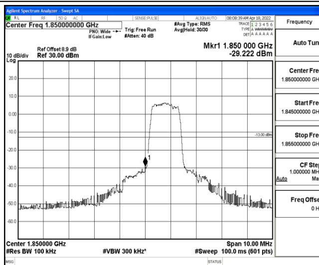
Band2-5MHz-QPSK-18625-6-0-Low--29.22-PASS
