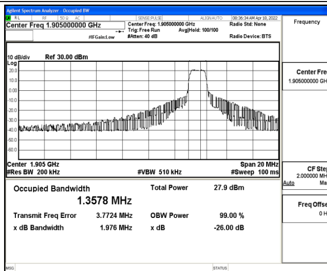
Band2-10MHz-QPSK-19150-6-0-High-1.3578-1.976-PASS
