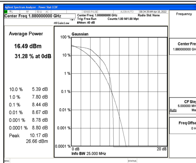
Band2-10MHz-16QAM-18900-6-0-Low-8.44-&lt;=13-PASS
