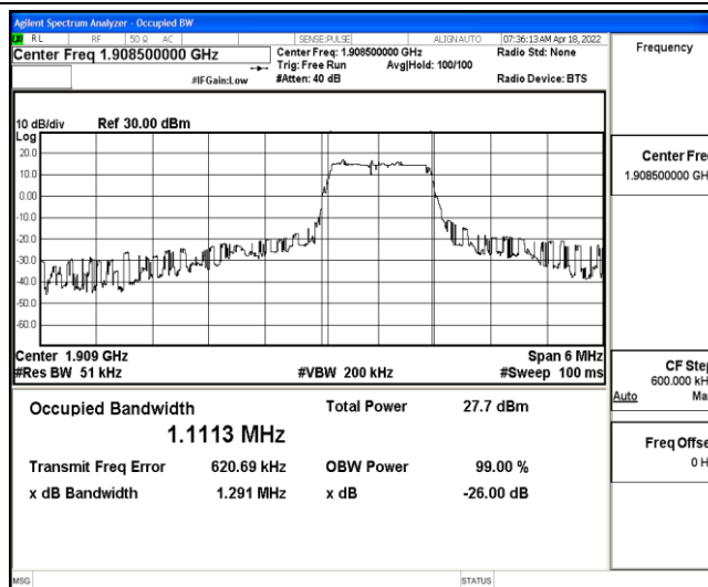
Band2-3MHz-16QAM-19185-6-0-High-1.1113-1.291-PASS
