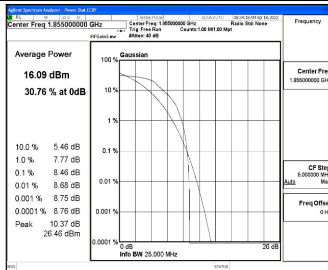
Band2-10MHz-16QAM-18650-6-0-Low-8.46-&lt;=13-PASS
