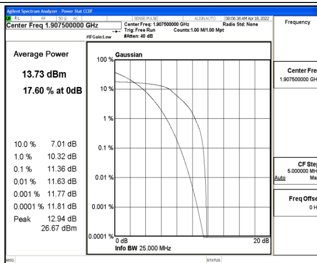
Band2-5MHz-16QAM-19175-6-0-Low-11.36-&lt;=13-PASS
