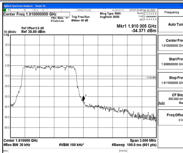
Band2-1.4MHz-16QAM-19193-6-0-Low--34.37-PASS
