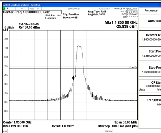
Band2-15MHz-QPSK-18675-6-0-Low--25.84-PASS
