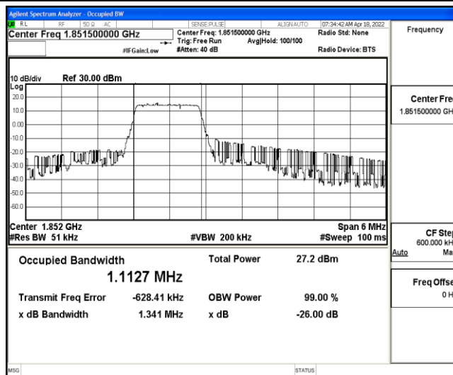
Band2-3MHz-QPSK-18615-6-0-Low-1.1127-1.341-PASS
