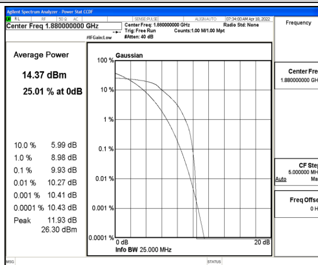
Band2-3MHz-16QAM-18900-6-0-Low-9.93-&lt;=13-PASS
