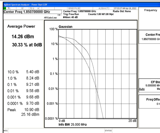
Band2-1.4MHz-QPSK-18607-6-0-Low-9.21-&lt;=13-PASS
