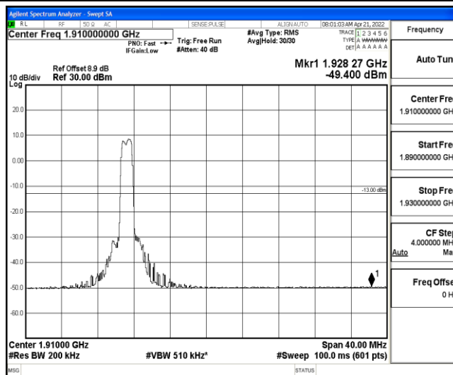
Band2-10MHz-QPSK-19150-6-0-Low--49.40-PASS
