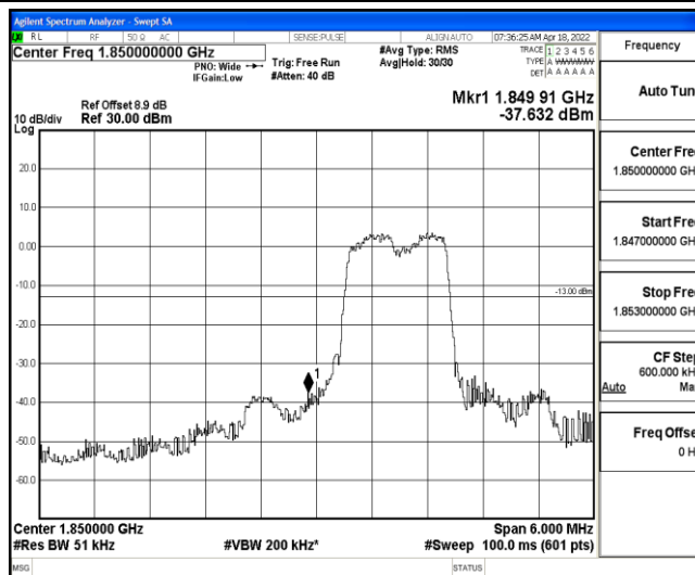
Band2-3MHz-QPSK-18615-6-0-Low--37.63-PASS
