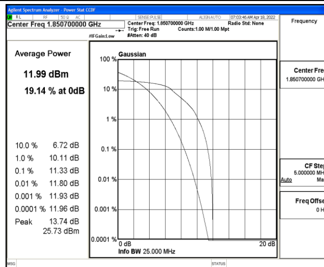
Band2-1.4MHz-16QAM-18607-6-0-Low-11.33-&lt;=13-PASS
