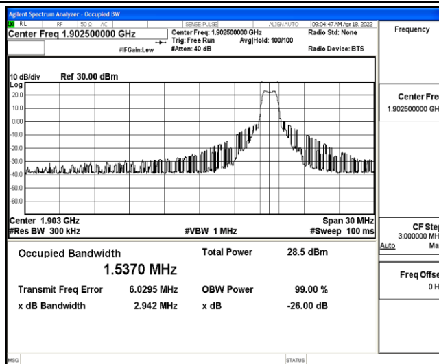
Band2-15MHz-QPSK-19125-6-0-High-1.5370-2.942-PASS
