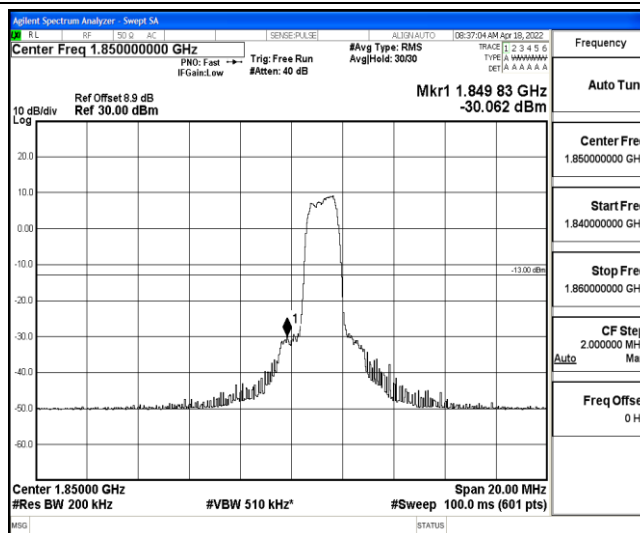
Band2-10MHz-QPSK-18650-6-0-Low--30.06-PASS
