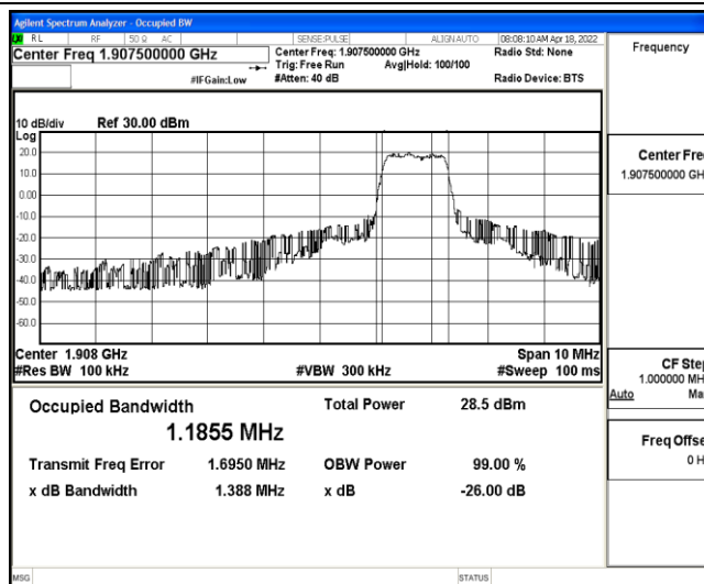
Band2-5MHz-QPSK-19175-6-0-High-1.1855-1.388-PASS
