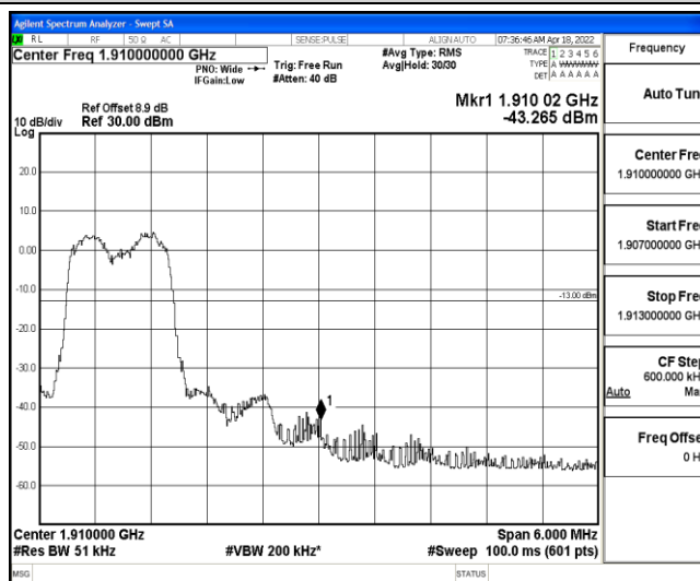
Band2-3MHz-QPSK-19185-6-0-Low--43.27-PASS
