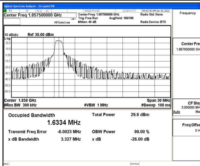
Band2-15MHz-QPSK-18675-6-0-Low-1.6334-3.327-PASS
