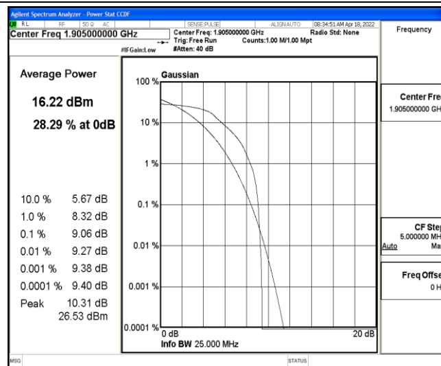
Band2-10MHz-QPSK-19150-6-0-Low-9.06-&lt;=13-PASS
