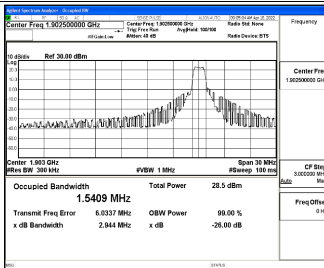
Band2-15MHz-16QAM-19125-6-0-High-1.5409-2.944-PASS
