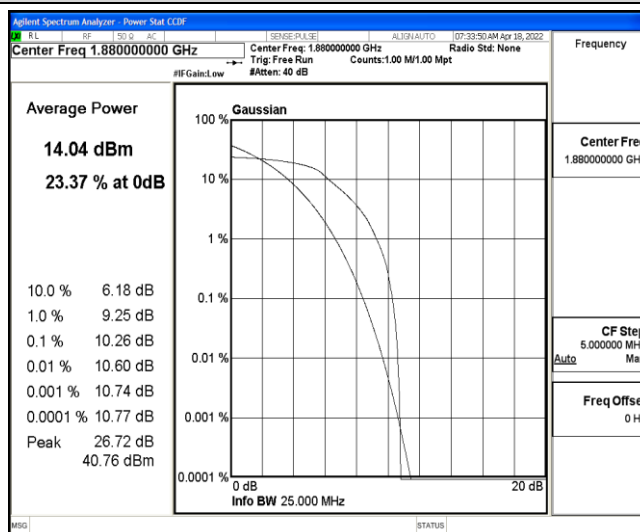
Band2-3MHz-QPSK-18900-6-0-Low-10.26-&lt;=13-PASS
