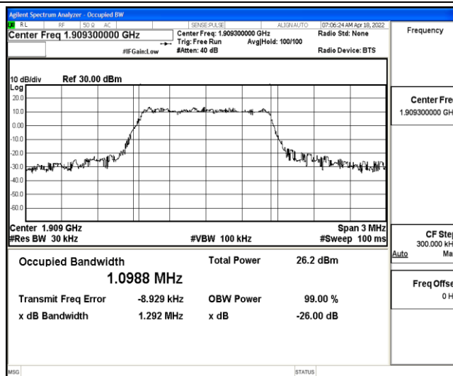
Band2-1.4MHz-QPSK-19193-6-0-High-1.0988-1.292-PASS
