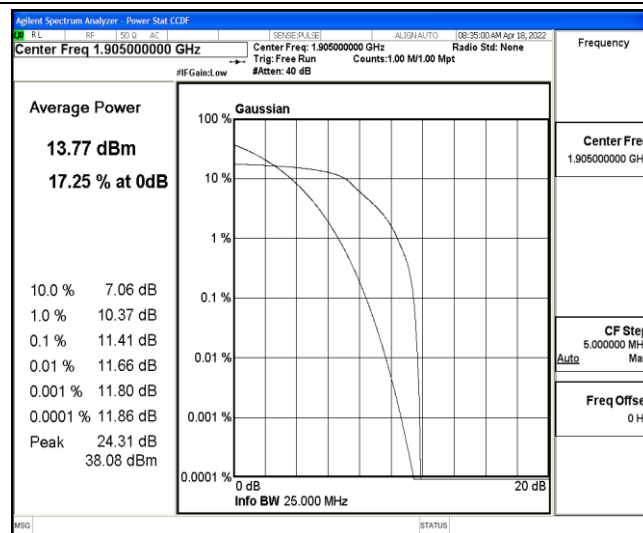
Band2-10MHz-16QAM-19150-6-0-Low-11.41-&lt;=13-PASS
