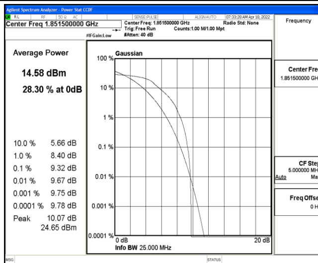
Band2-3MHz-QPSK-18615-6-0-Low-9.32-&lt;=13-PASS
