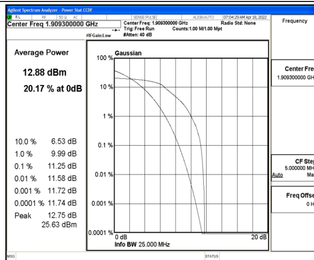
Band2-1.4MHz-QPSK-19193-6-0-Low-11.25-&lt;=13-PASS
