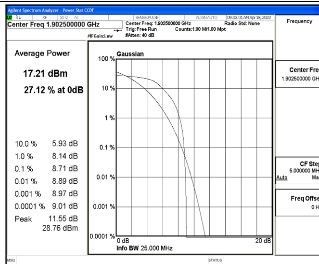
Band2-15MHz-QPSK-19125-6-0-Low-8.71-&lt;=13-PASS
