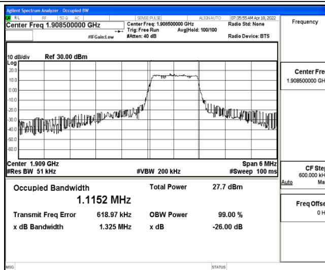
Band2-3MHz-QPSK-19185-6-0-High-1.1152-1.325-PASS
