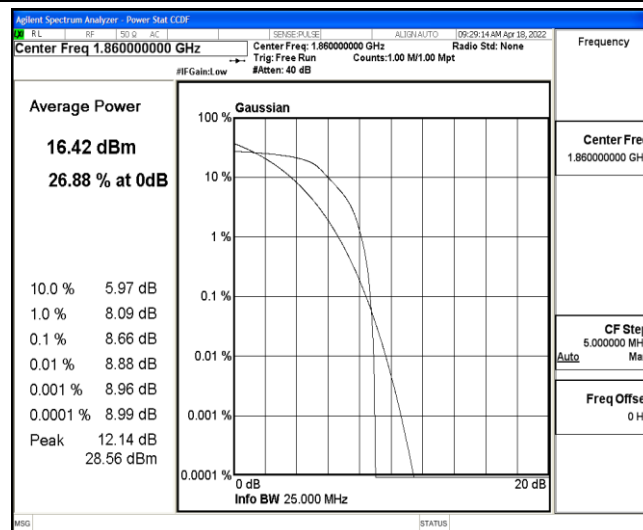
Band2-20MHz-16QAM-18700-6-0-Low-8.66-&lt;=13-PASS
