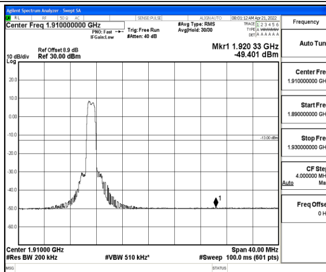
Band2-10MHz-16QAM-19150-6-0-Low--49.40-PASS
