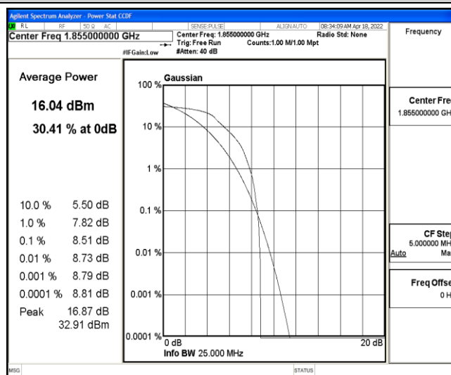
Band2-10MHz-QPSK-18650-6-0-Low-8.51-&lt;=13-PASS
