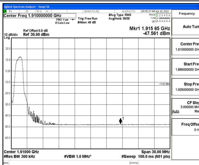
Band2-15MHz-QPSK-19125-6-0-Low--47.56-PASS
