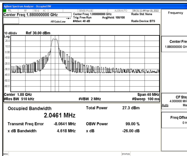
Band2-20MHz-16QAM-18900-6-0-Low-2.0461-4.618-PASS
