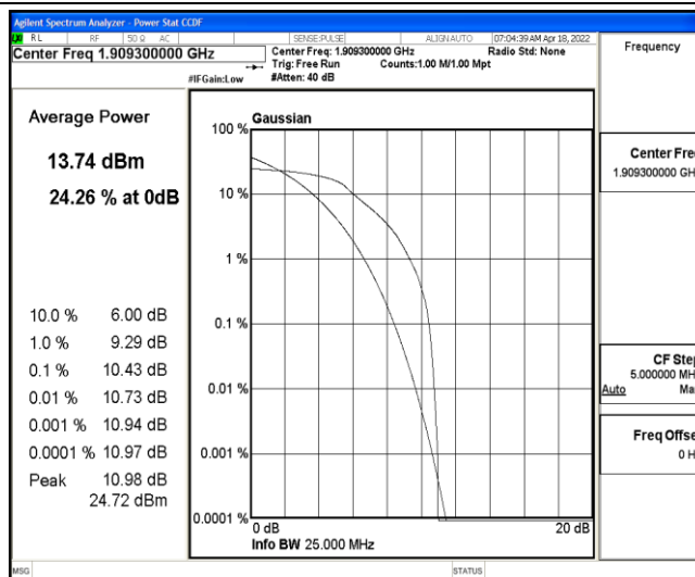
Band2-1.4MHz-16QAM-19193-6-0-Low-10.43-&lt;=13-PASS
