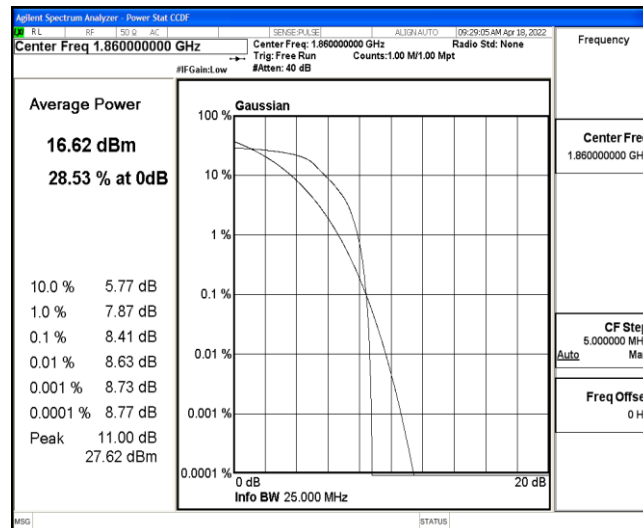
Band2-20MHz-QPSK-18700-6-0-Low-8.41-&lt;=13-PASS
