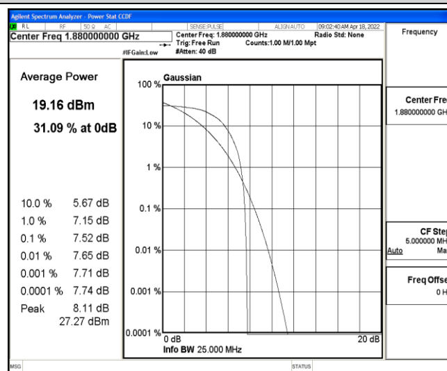
Band2-15MHz-QPSK-18900-6-0-Low-7.52-&lt;=13-PASS
