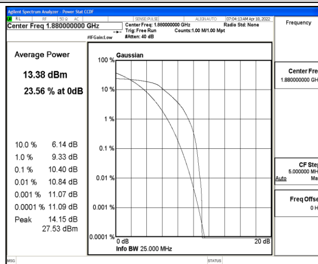
Band2-1.4MHz-16QAM-18900-6-0-Low-10.40-&lt;=13-PASS
