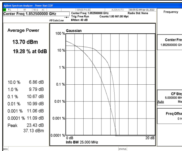
Band2-5MHz-16QAM-18625-6-0-Low-10.67-&lt;=13-PASS
