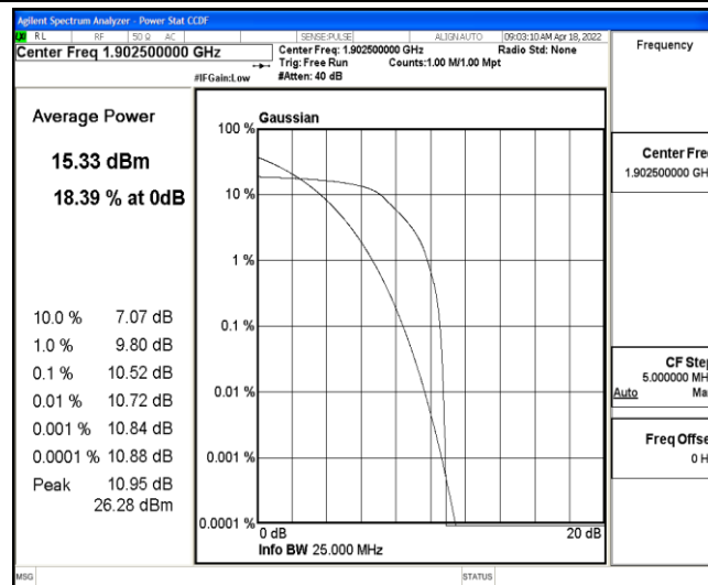
Band2-15MHz-16QAM-19125-6-0-Low-10.52-&lt;=13-PASS
