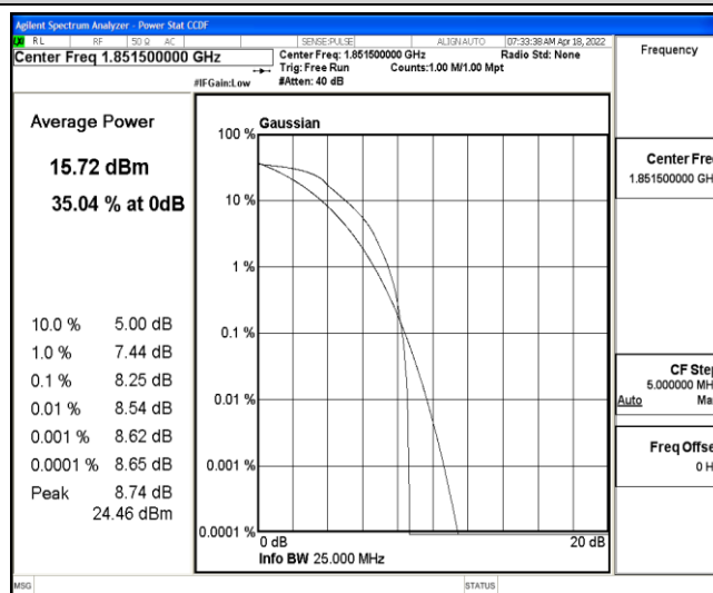
Band2-3MHz-16QAM-18615-6-0-Low-8.25-&lt;=13-PASS
