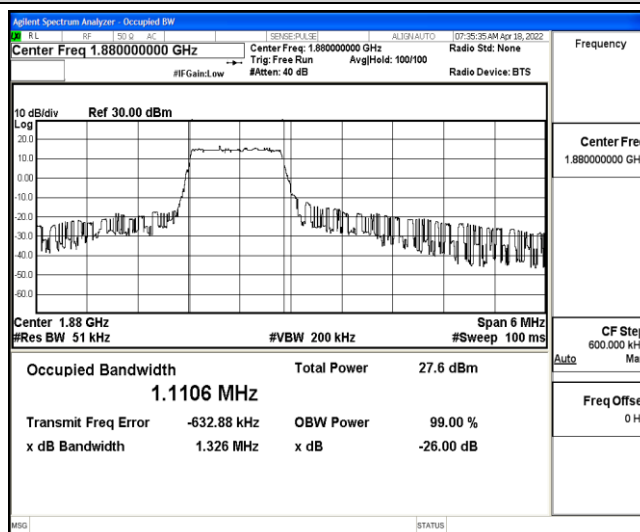
Band2-3MHz-16QAM-18900-6-0-Low-1.1106-1.326-PASS
