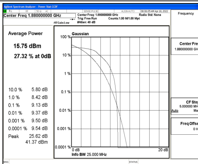
Band2-5MHz-QPSK-18900-6-0-Low-9.13-&lt;=13-PASS
