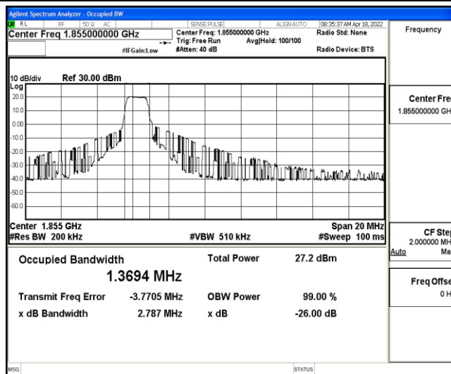
Band2-10MHz-16QAM-18650-6-0-Low-1.3694-2.787-PASS
