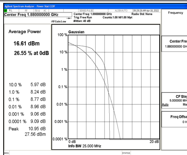
Band2-20MHz-QPSK-18900-6-0-Low-8.77-&lt;=13-PASS
