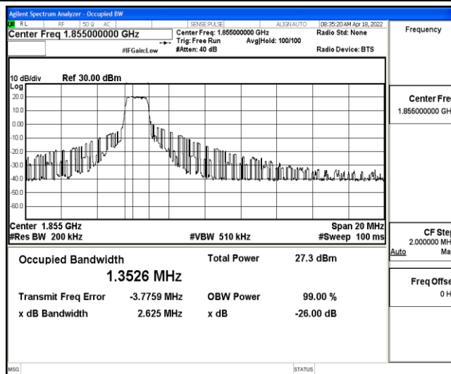
Band2-10MHz-QPSK-18650-6-0-Low-1.3526-2.625-PASS
