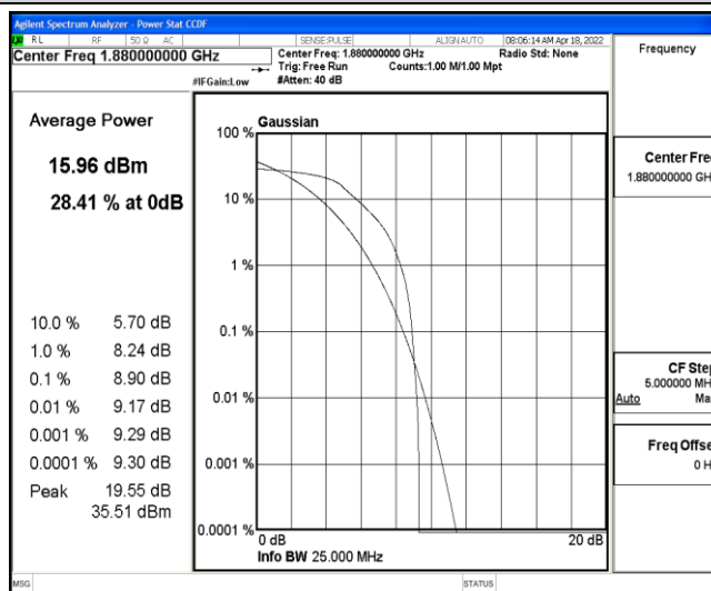
Band2-5MHz-16QAM-18900-6-0-Low-8.90-&lt;=13-PASS
