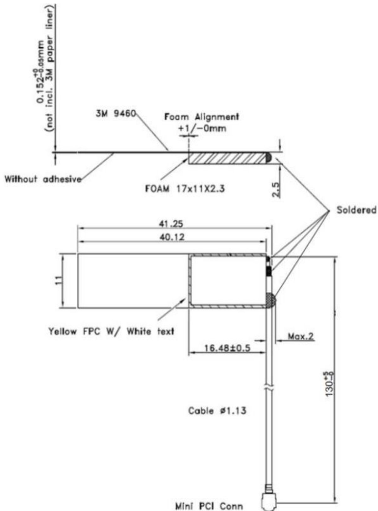
Figure 2: FlexPIFA mechanical drawing of EFB2400A3S-13MHF1
