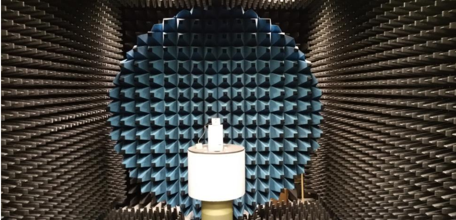
Figure 4: Antenna chamber
