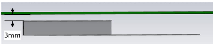
Figure 20: Top clearance
