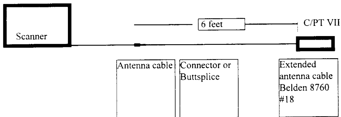
Figure 3.2.2 Scanner Connection
