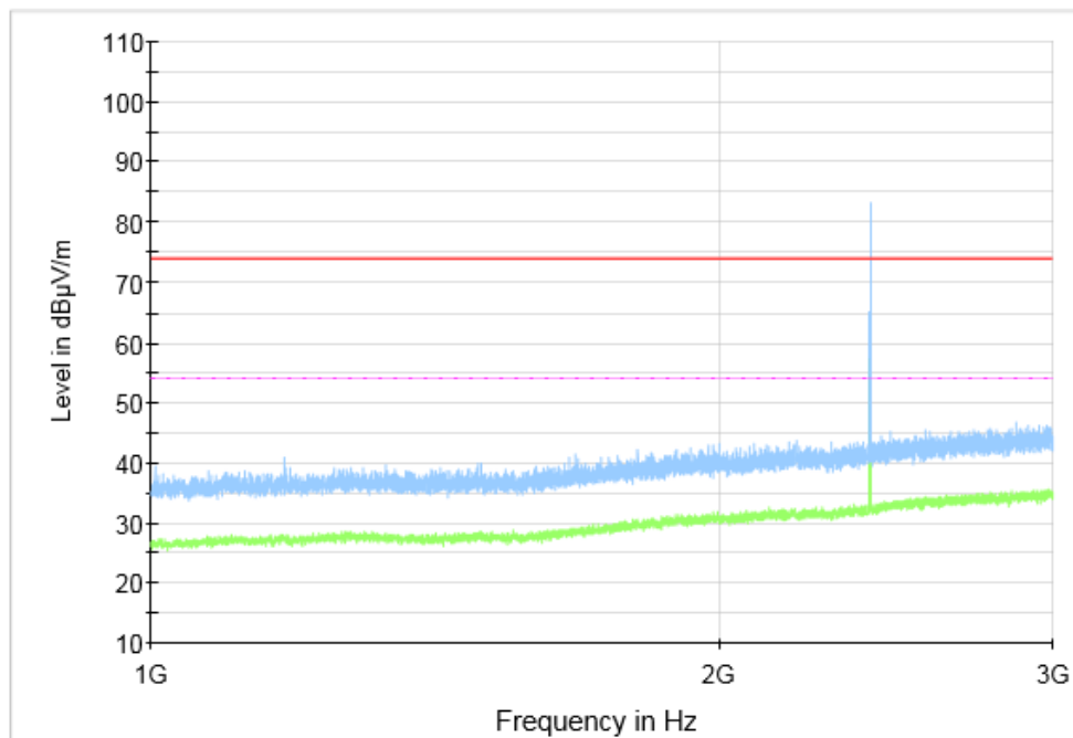
Fig.50 Radiated Spurious Emission (GFSK, Ch0, 1 GHz ~3 GHz), LE 2M
