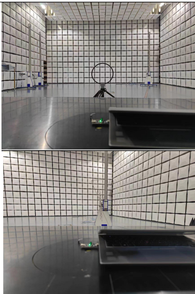
Spurious Radiated Emissions Test setup
