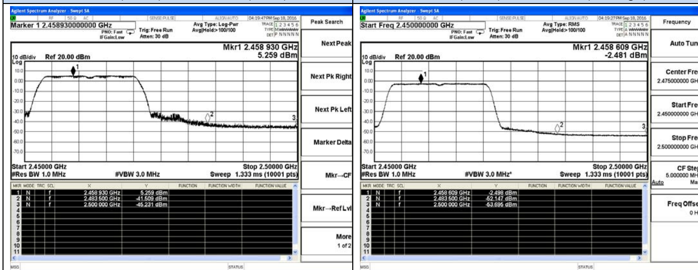
802.11n(HT20)-High channel(Peak)
