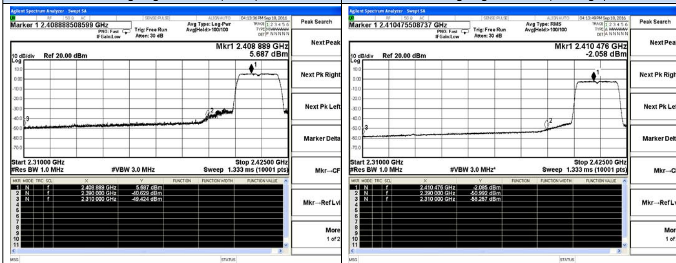
802.11n(HT20)-Low channel(Peak)
