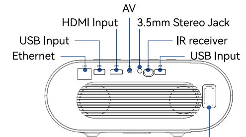
Power Socket
