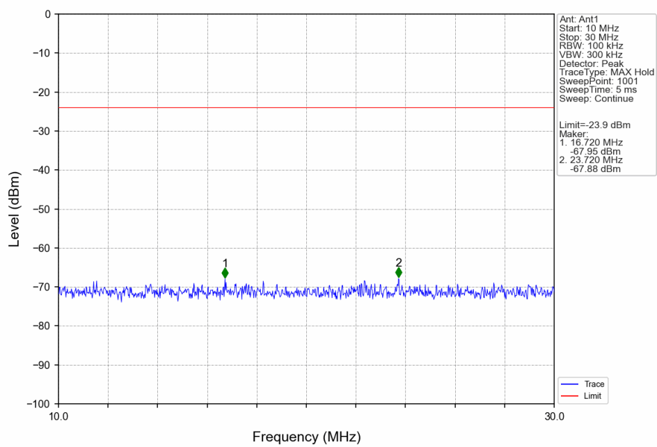
1M_HCH_2480MHz_Ant1_NTNV
