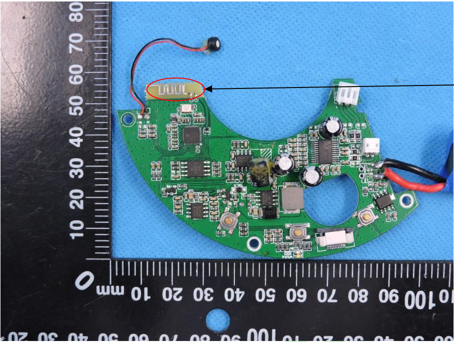
BT Antenna
