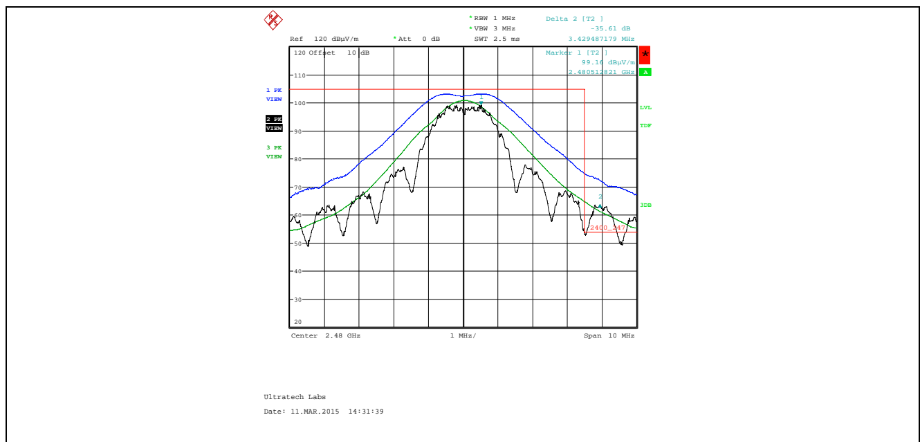
Plot 5.4.4.4.2.4. Band-Edge RF Radiated Emissions at 3 m, Vertical Polarization High End of Frequency Band, QPSK Modulation, Power -24 Mode 3
