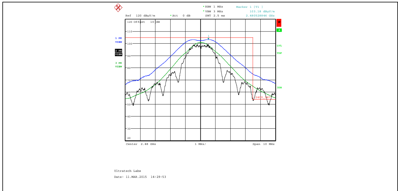
Plot 5.4.4.4.2.3. Band-Edge RF Radiated Emissions at 3 m, Vertical Polarization High End of Frequency Band, QPSK Modulation, Power -24 Mode 3
