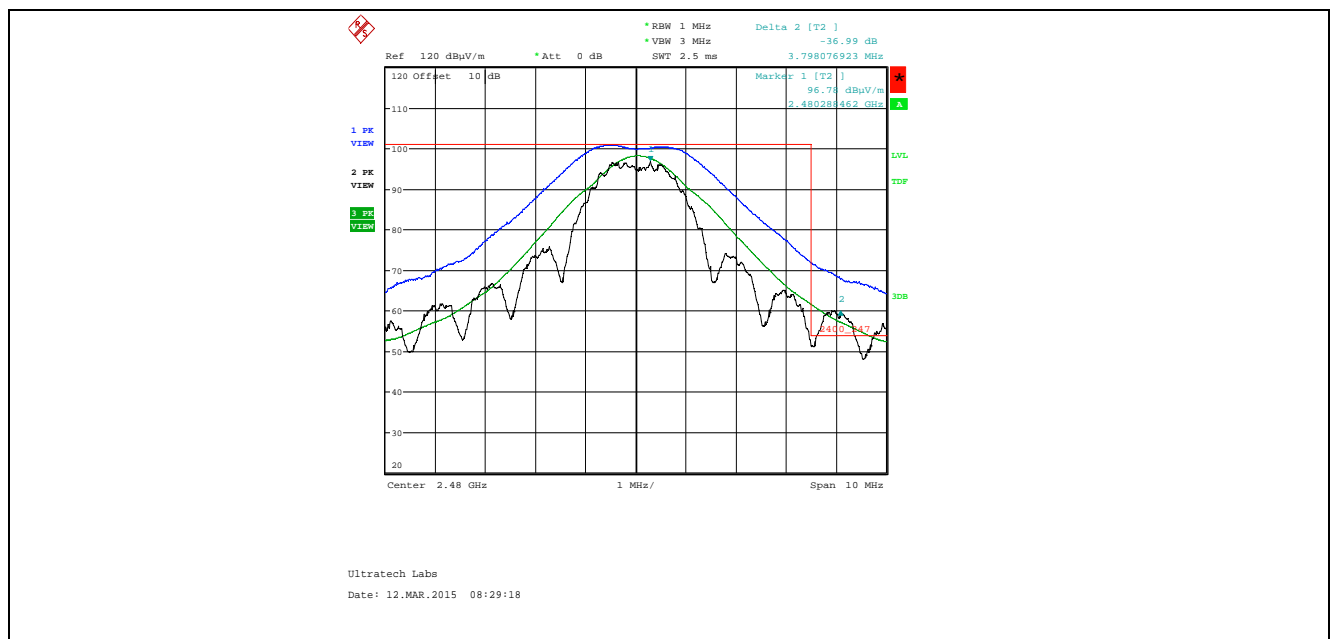
Plot 5.4.4.5.2.4. Band-Edge RF Radiated Emissions at 3 m, Vertical Polarization High End of Frequency Band, QPSK Modulation, Power -24 Mode 3
