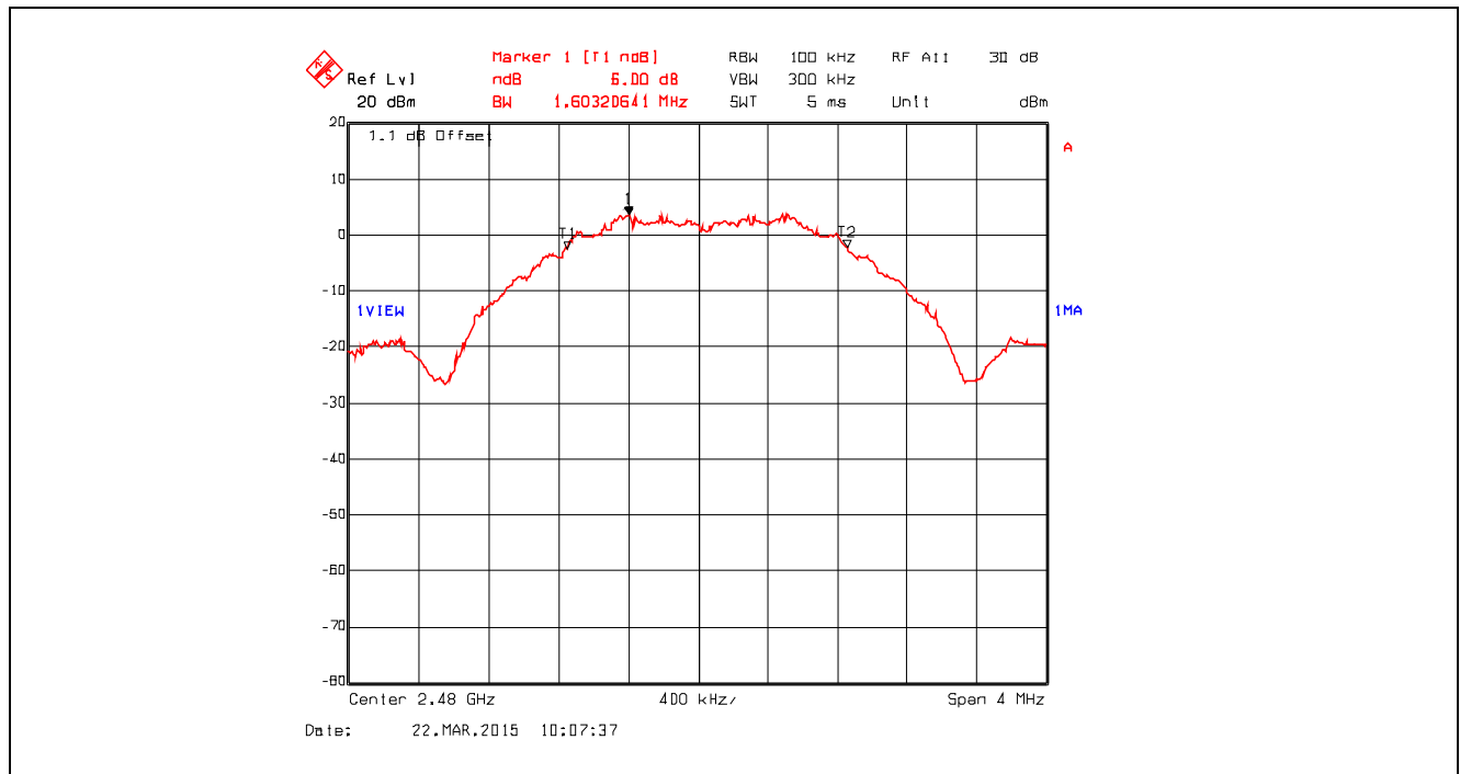
Plot 5.1.4.1. 6 dB Bandwidth, Channel 26, 2480 MHz, QPSK Modulation, Power Setting -24 Mode 3
