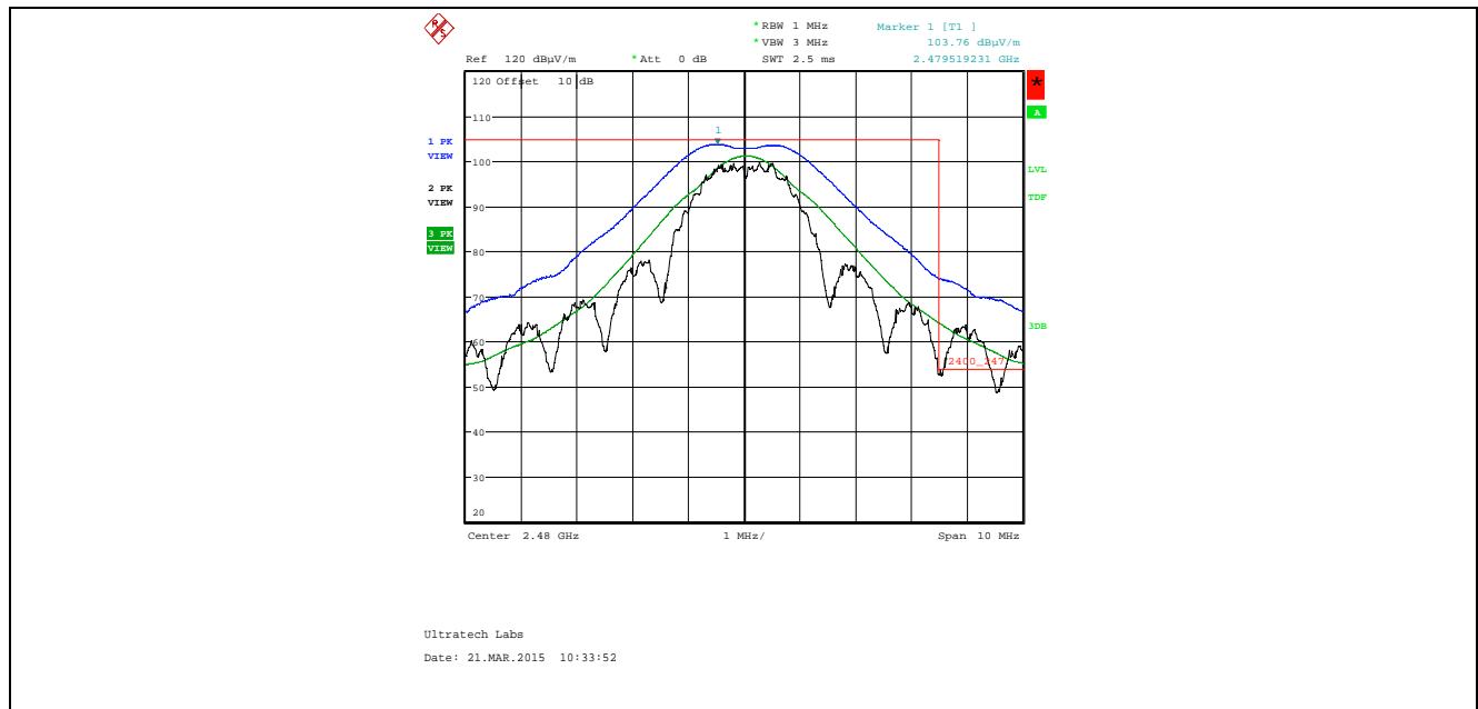
Plot 5.4.4.1.2.3. Band-Edge RF Radiated Emissions at 3 m, Vertical Polarization High End of Frequency Band, QPSK Modulation, Power -24 Mode 3
