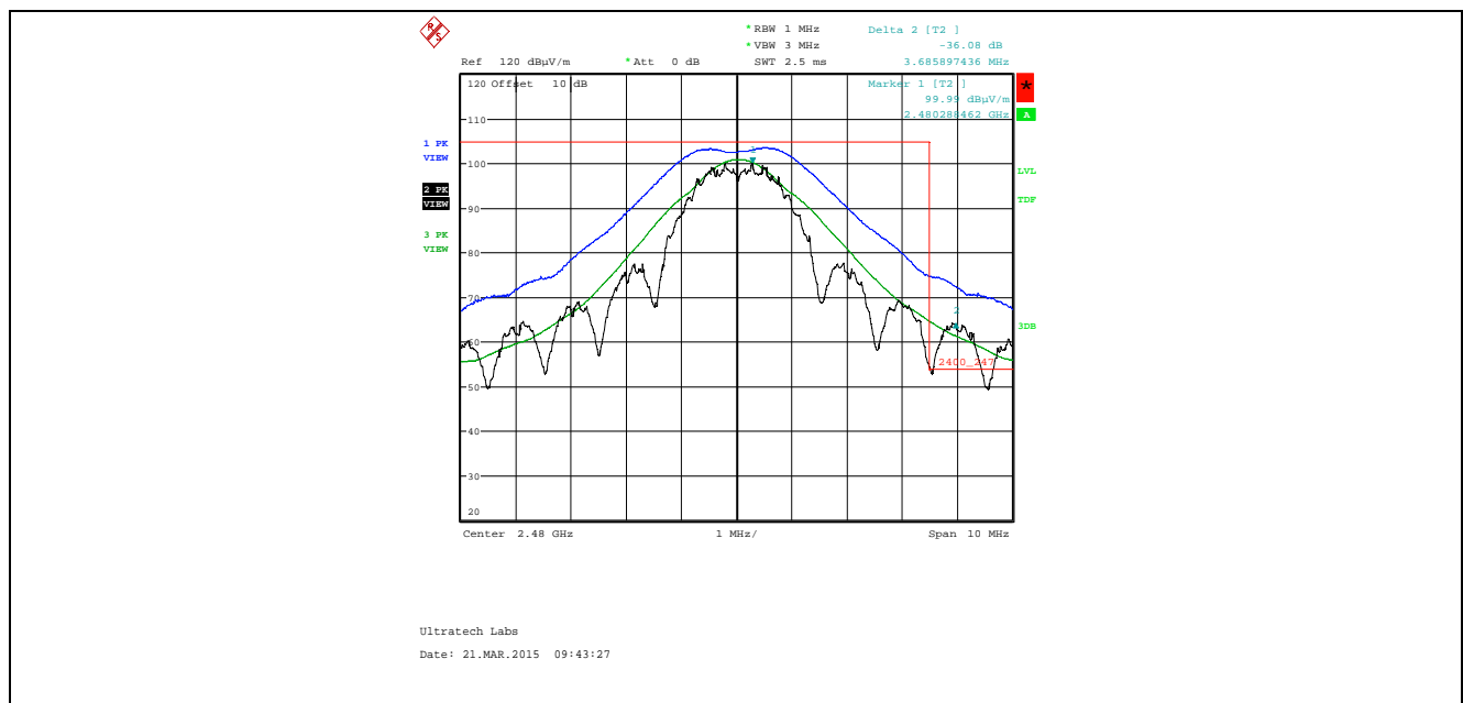
Plot 5.4.4.2.2.4. Band-Edge RF Radiated Emissions at 3 m, Vertical Polarization High End of Frequency Band, QPSK Modulation, Power -24 Mode 3
