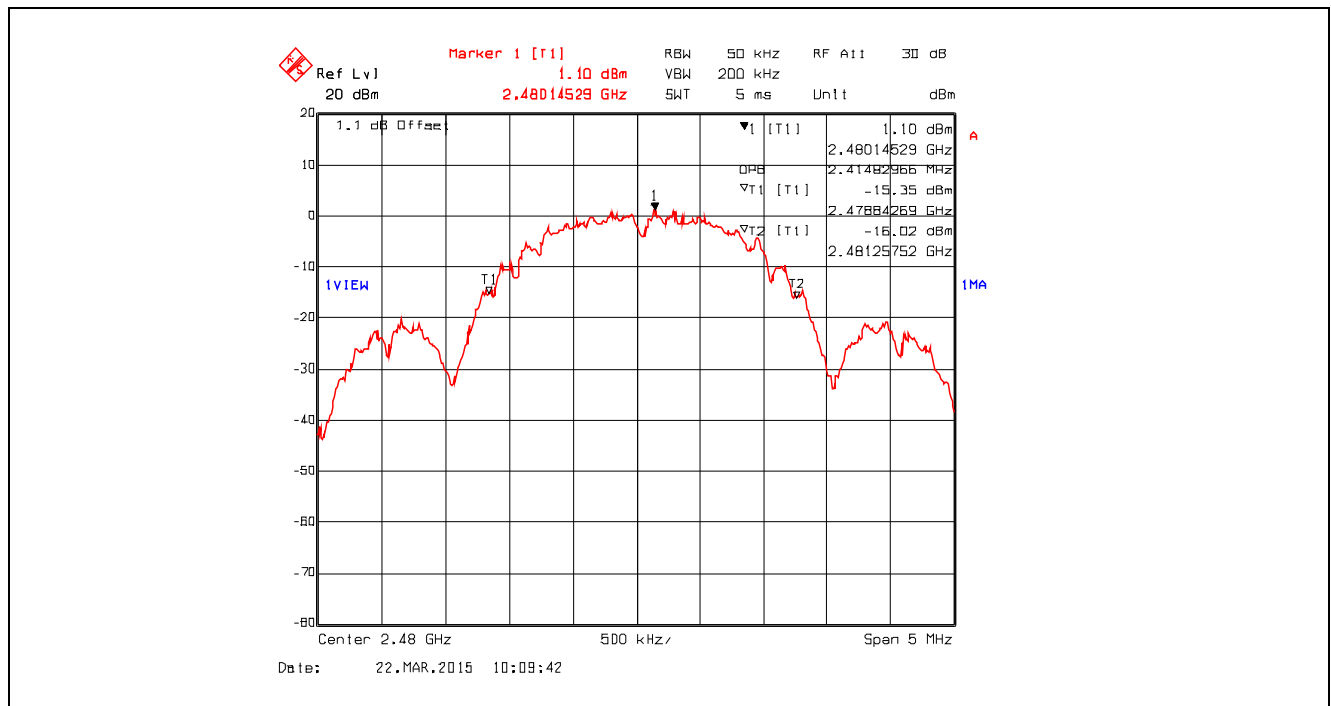
Plot 5.1.4.2. 99% Occupied Bandwidth, Channel 26, 2480 MHz, QPSK Modulation, Power Setting -24 Mode 3
