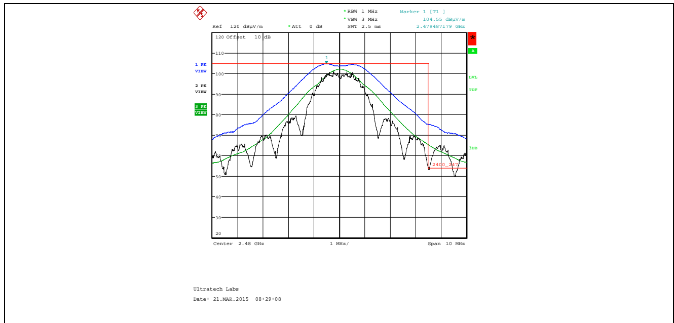
Plot 5.4.4.3.2.3. Band-Edge RF Radiated Emissions at 3 m, Vertical Polarization High End of Frequency Band, QPSK Modulation, Power -24 Mode 3
