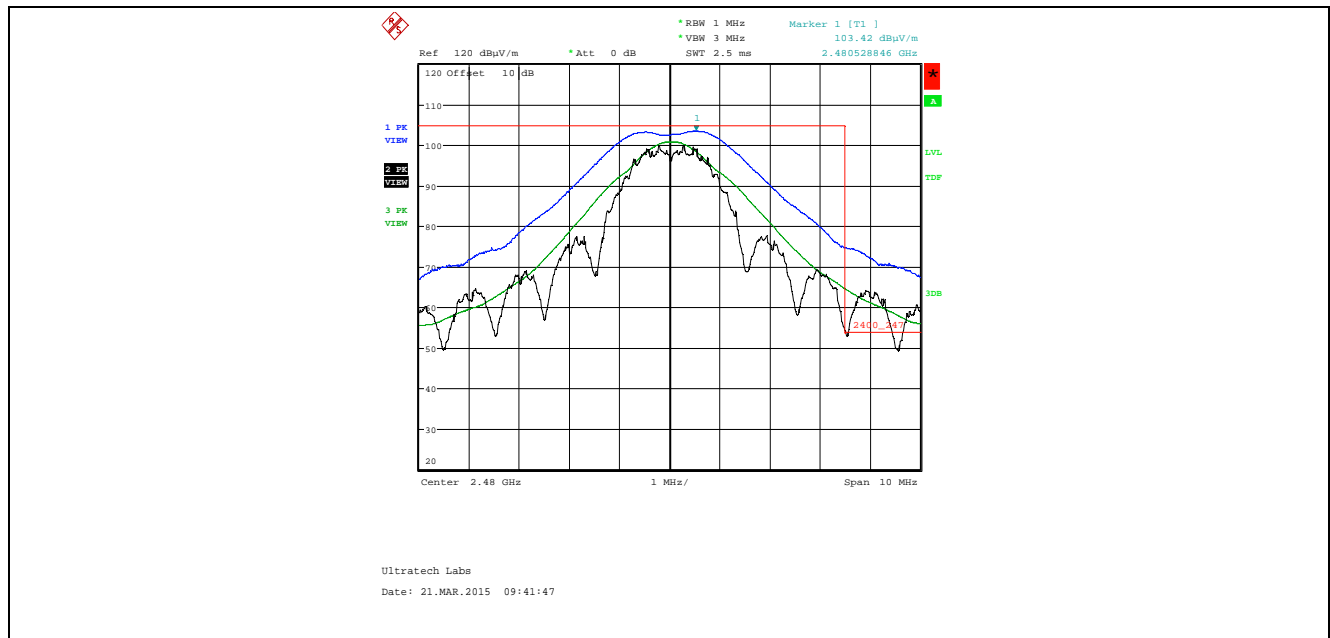
Plot 5.4.4.2.2.3. Band-Edge RF Radiated Emissions at 3 m, Vertical Polarization High End of Frequency Band, QPSK Modulation, Power -24 Mode 3
