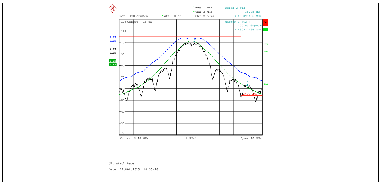
Plot 5.4.4.1.2.4. Band-Edge RF Radiated Emissions at 3 m, Vertical Polarization High End of Frequency Band, QPSK Modulation, Power -24 Mode 3
