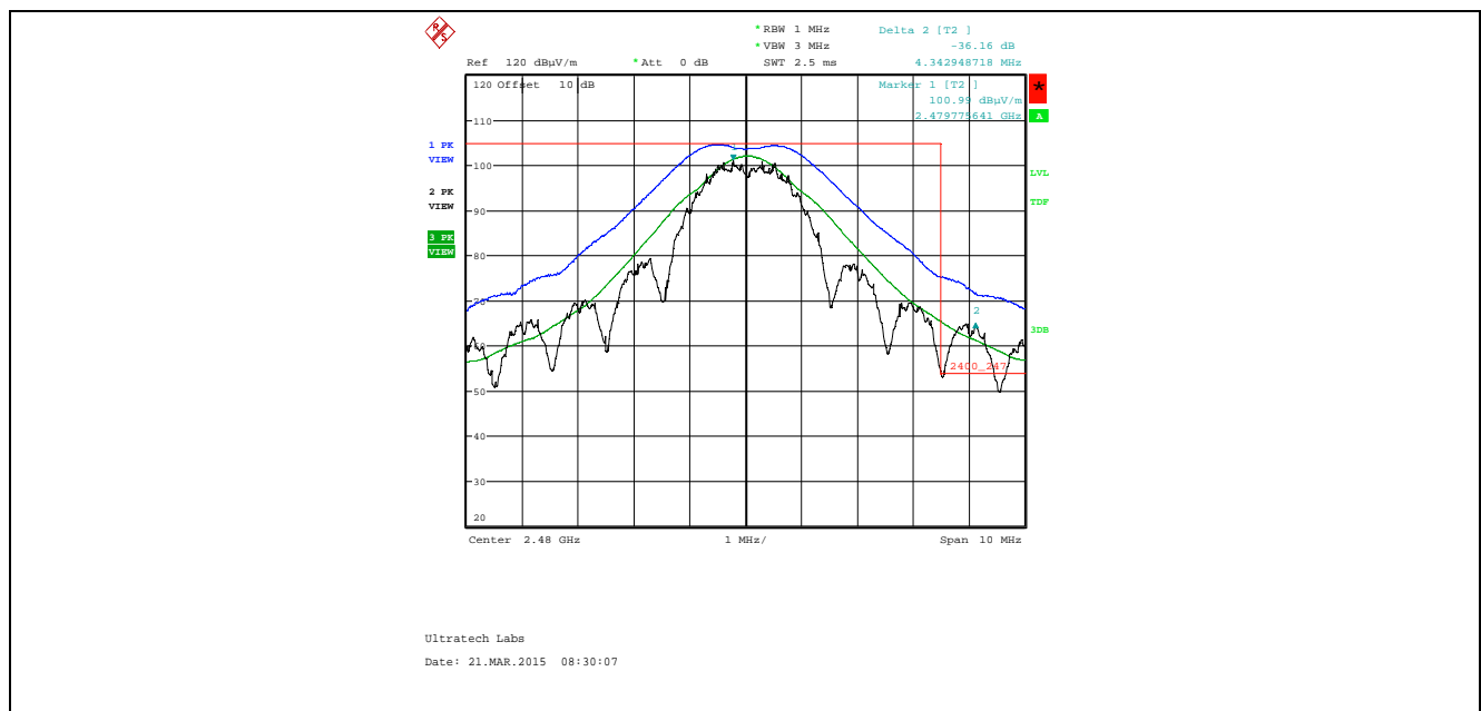
Plot 5.4.4.3.2.4. Band-Edge RF Radiated Emissions at 3 m, Vertical Polarization High End of Frequency Band, QPSK Modulation, Power -24 Mode 3
