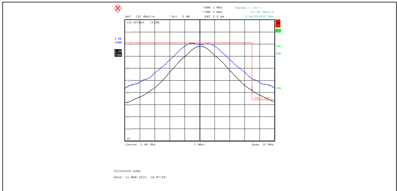
Plot 5.4.4.4.2.2. Band-Edge RF Radiated Emissions at 3 m, Horizontal Polarization High End of Frequency Band, QPSK Modulation, Power -24 Mode 3
