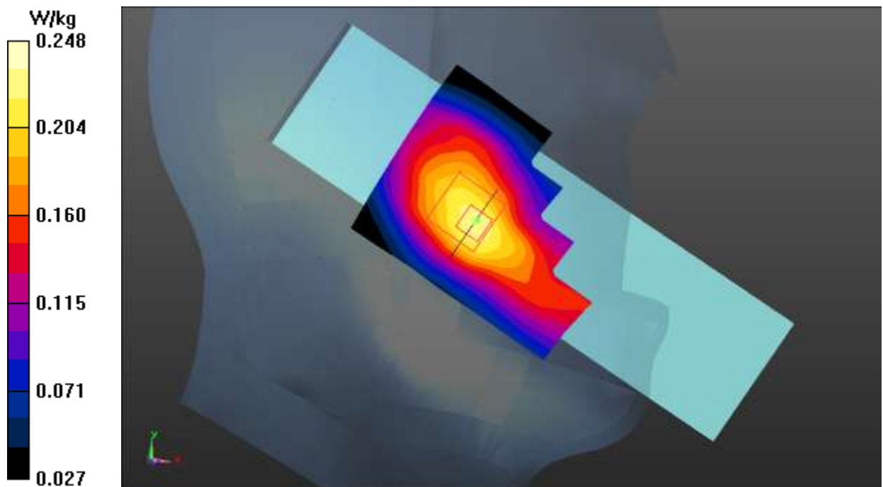
Fig.19 LTE Band 12
