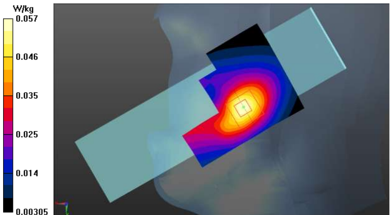
Fig.31 LTE Band 71
