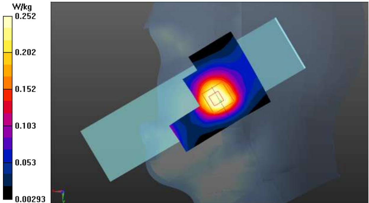
Fig.29 LTE Band 66
