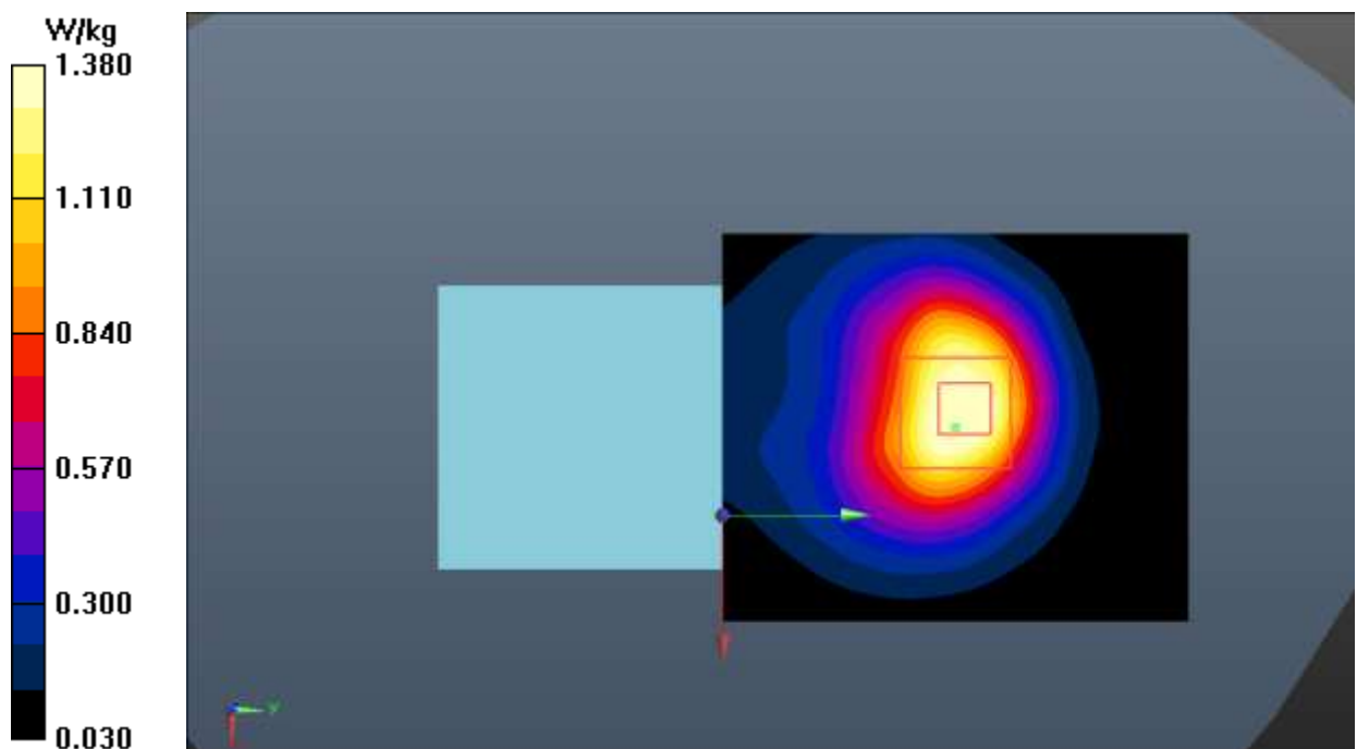
Fig.30 LTE Band 66
