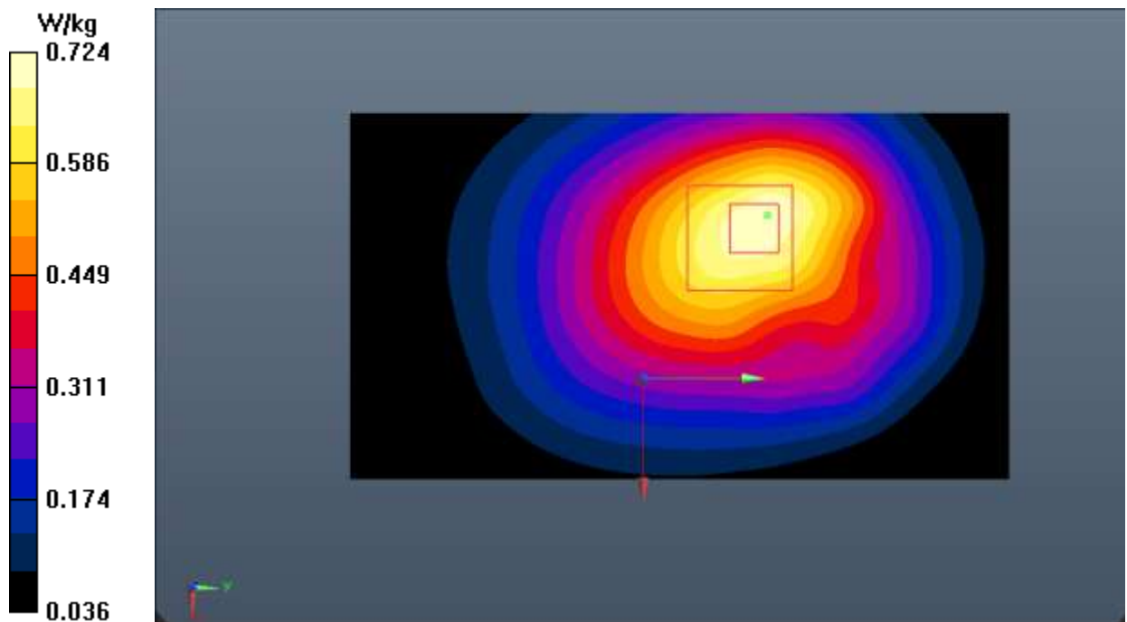
Fig.26 LTE Band 26
