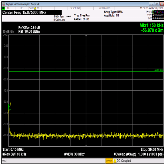
Band5_3MHz_QPSK_20635_1RB#0_0.15~30_0.15~30
