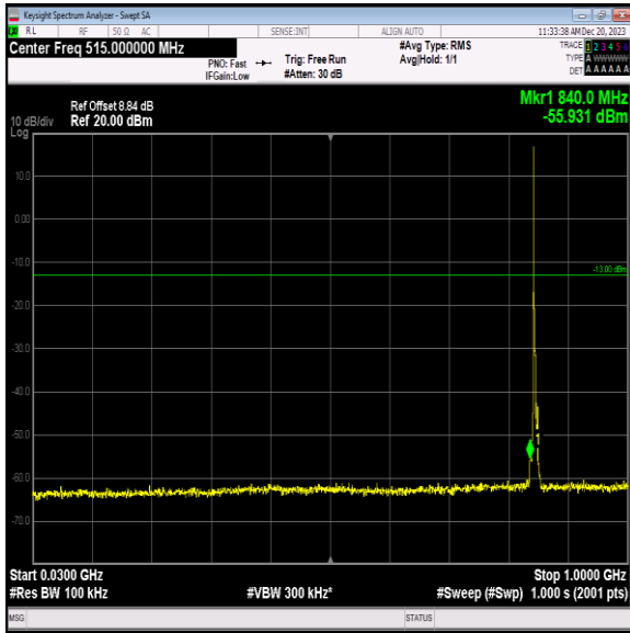
Band5_3MHz_16QAM_20635_1RB#0_30~1000_30~1000
