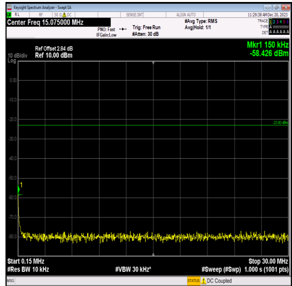
Band5_3MHz_QPSK_20525_1RB#0_0.15~30_0.15~30
