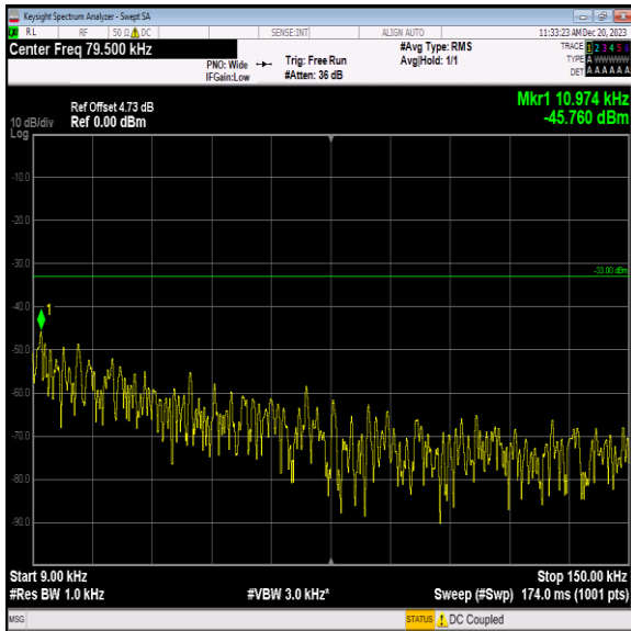
Band5_3MHz_16QAM_20635_1RB#0_0.009~0.15_0.009~0.15 5
