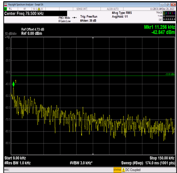
Band5_3MHz_64QAM_20415_1RB#0_0.009~0.15_0.009~0.15 5
