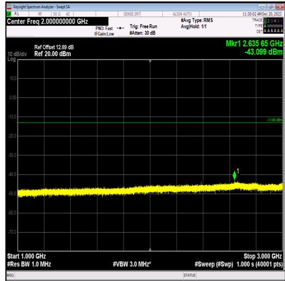
Band5_3MHz_QPSK_20525_1RB#0_1000~3000_1000~3000
