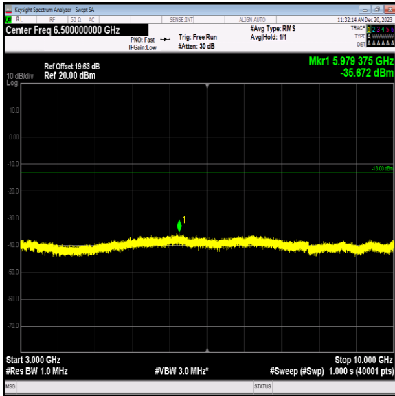
Band5_3MHz_64QAM_20525_1RB#0_3000~10000_3000~10000
