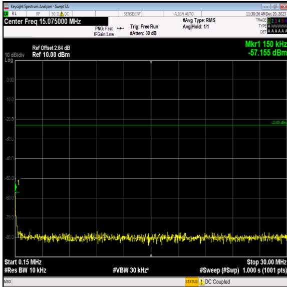
Band5_3MHz_16QAM_20525_1RB#0_0.15~30_0.15~30
