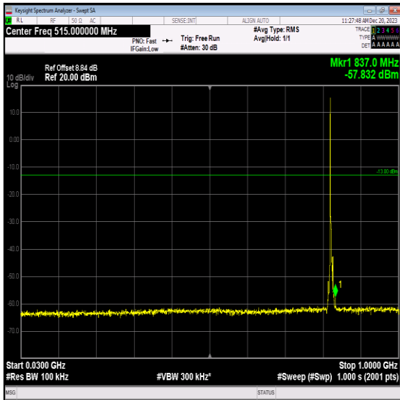
Band5_3MHz_16QAM_20415_1RB#0_30~1000_30~1000
