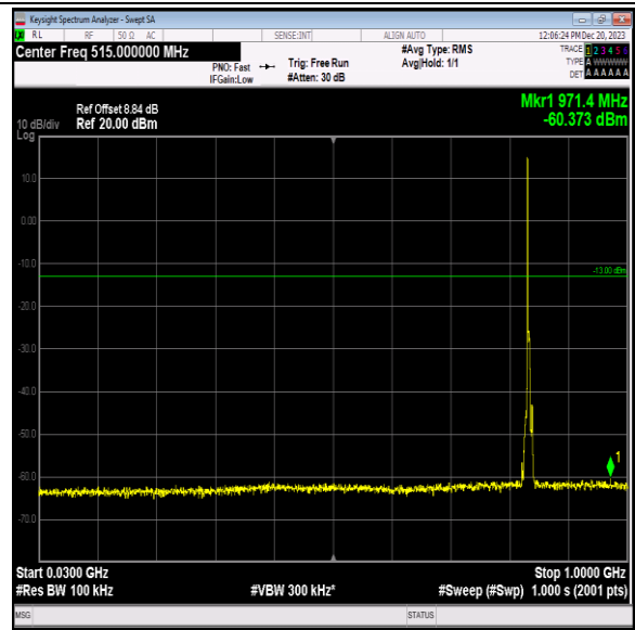
Band5_5MHz_QPSK_20525_1RB#0_30~1000_30~1000
