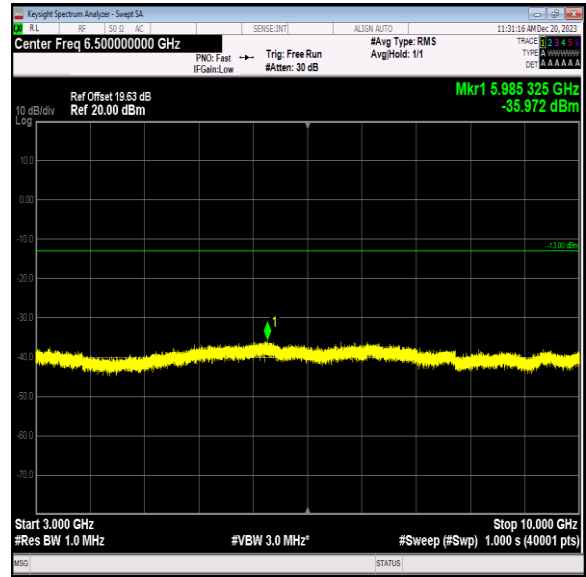
Band5_3MHz_16QAM_20525_1RB#0_3000~10000_3000~10000 000
