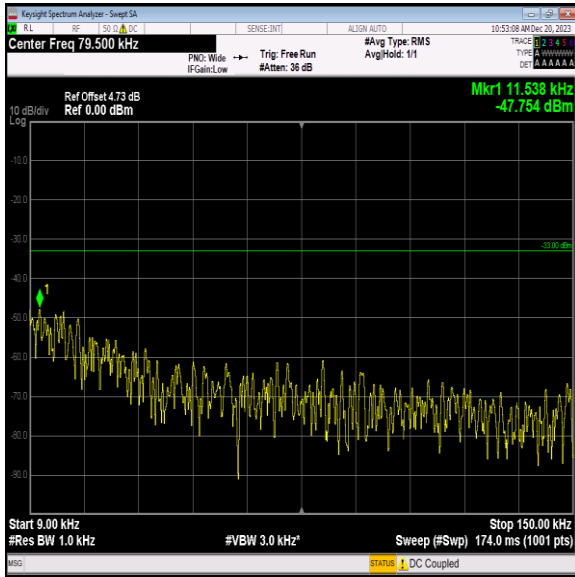
Band5_1.4MHz_64QAM_20643_1RB#0_0.009~0.15_0.009~0.15
