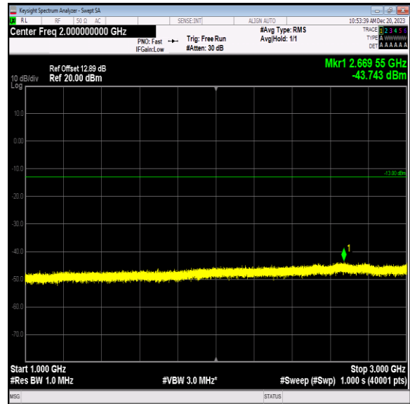
Band5_1.4MHz_64QAM_20643_1RB#0_1000~3000_1000~3000
