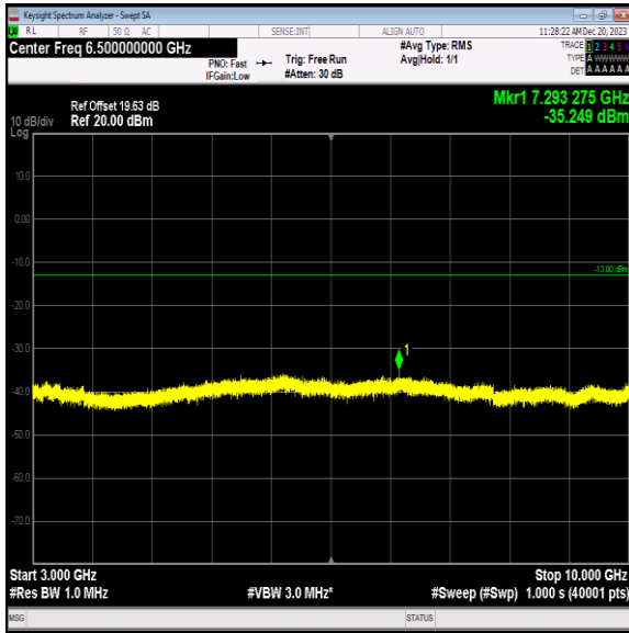
Band5_3MHz_16QAM_20415_1RB#0_3000~10000_3000~10000
