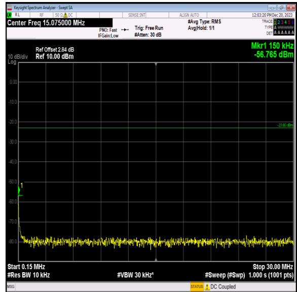
Band5_5MHz_QPSK_20425_1RB#0_0.15~30_0.15~30
