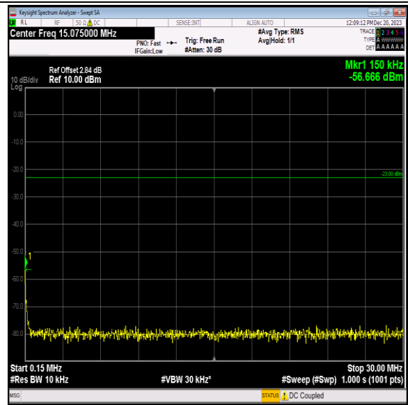
Band5_5MHz_QPSK_20625_1RB#0_0.15~30_0.15~30
