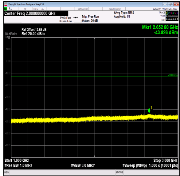
Band5_5MHz_QPSK_20425_1RB#0_1000~3000_1000~3000
