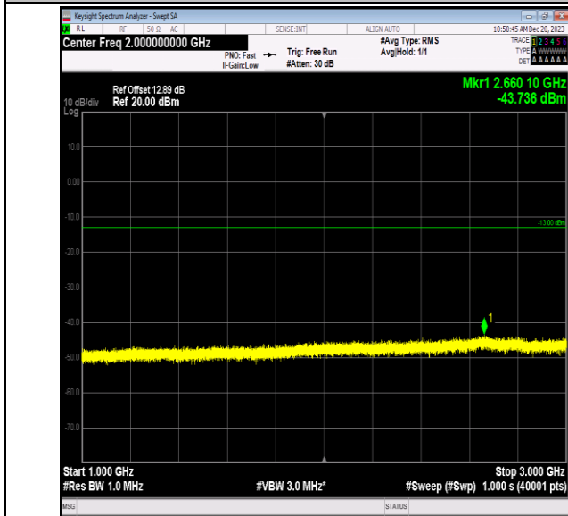
Band5_1.4MHz_64QAM_20525_1RB#0_1000~3000_1000~3000
