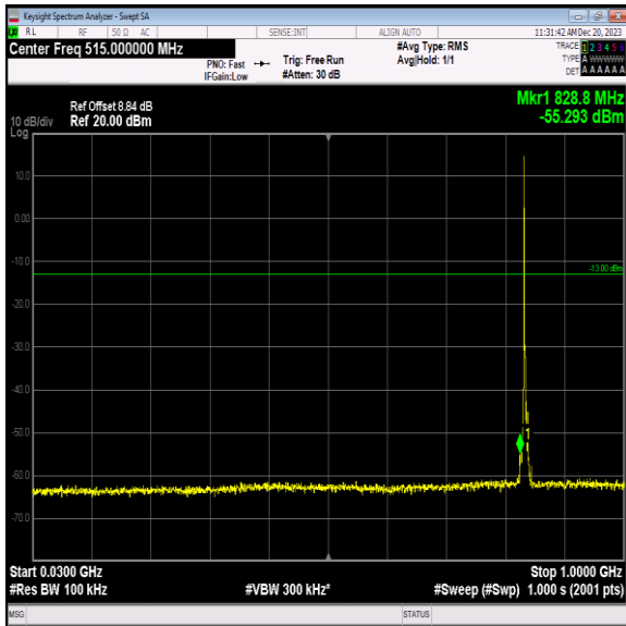
Band5_3MHz_64QAM_20525_1RB#0_30~1000_30~1000
