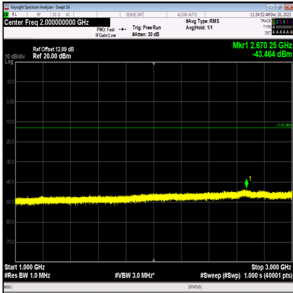
Band5_3MHz_64QAM_20635_1RB#0_1000~3000_1000~3000 0
