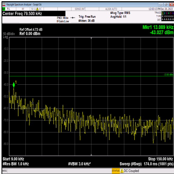
Band5_5MHz_QPSK_20425_1RB#0_0.009~0.15_0.009~0.15
