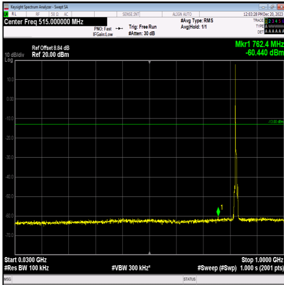
Band5_5MHz_QPSK_20425_1RB#0_30~1000_30~1000
