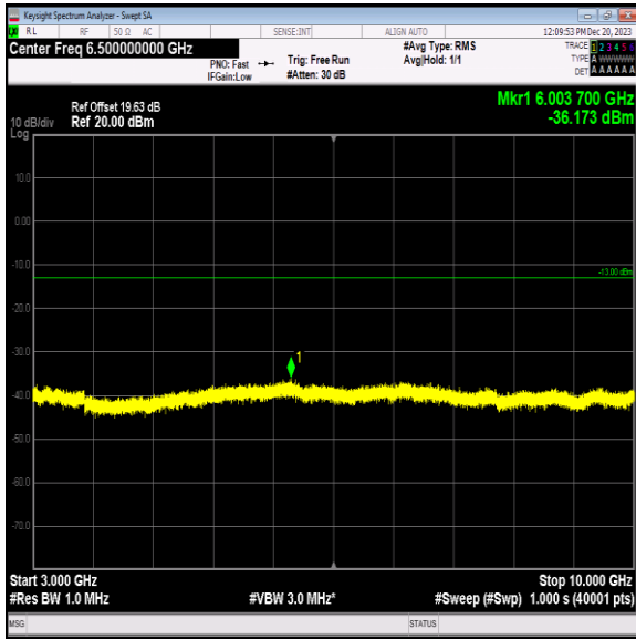
Band5_5MHz_QPSK_20625_1RB#0_3000~10000_3000~100 00
