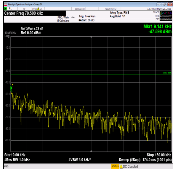
Band5_5MHz_16QAM_20625_1RB#0_0.009~0.15_0.009~0.15 5
