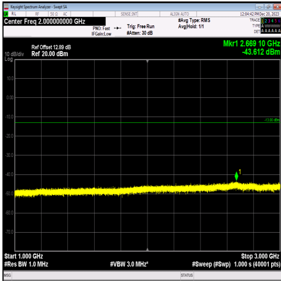
Band5_5MHz_16QAM_20425_1RB#0_1000~3000_1000~3000 0
