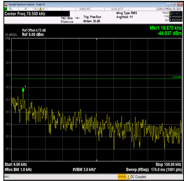
Band5_5MHz_16QAM_20425_1RB#0_0.009~0.15_0.009~0.1 5
