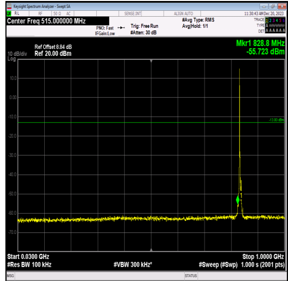
Band5_3MHz_16QAM_20525_1RB#0_30~1000_30~1000
