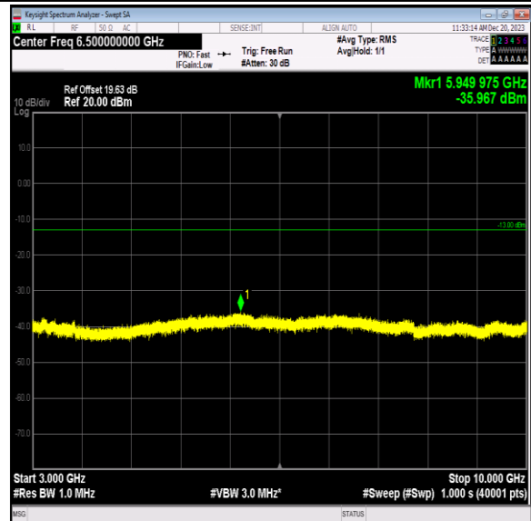
Band5_3MHz_QPSK_20635_1RB#0_3000~10000_3000~10000 00
