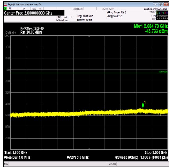
Band5_3MHz_16QAM_20415_1RB#0_1000~3000_1000~300 0
