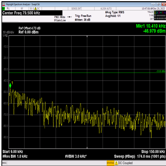
Band5_1.4MHz_64QAM_20407_1RB#0_0.009~0.15_0.009~0.15
