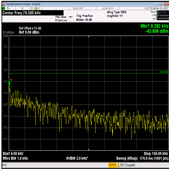
Band5_3MHz_16QAM_20415_1RB#0_0.009~0.15_0.009~0.1 5
