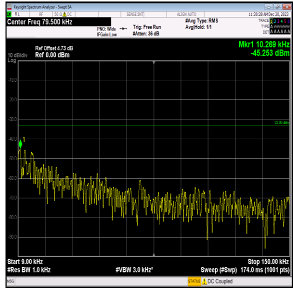
Band5_3MHz_16QAM_20525_1RB#0_0.009~0.15_0.009~0.15
