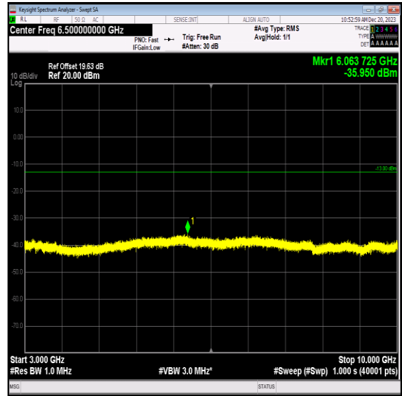
Band5_1.4MHz_16QAM_20643_1RB#0_3000~10000_3000~10000
