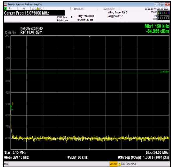
Band5_3MHz_16QAM_20635_1RB#0_0.15~30_0.15~30
