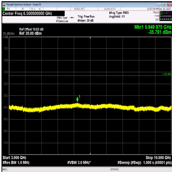
Band5_5MHz_16QAM_20525_1RB#0_3000~10000_3000~10000 000
