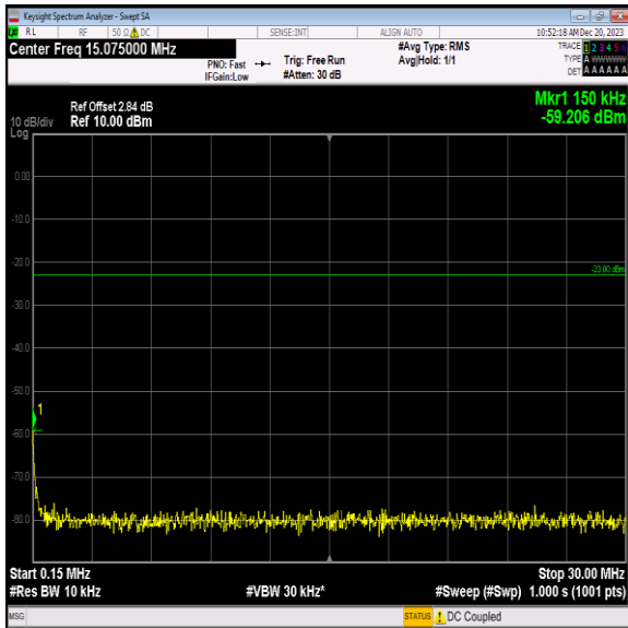
Band5_1.4MHz_16QAM_20643_1RB#0_0.15~30_0.15~30
