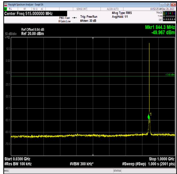
Band5_1.4MHz_16QAM_20643_1RB#0_30~1000_30~1000
