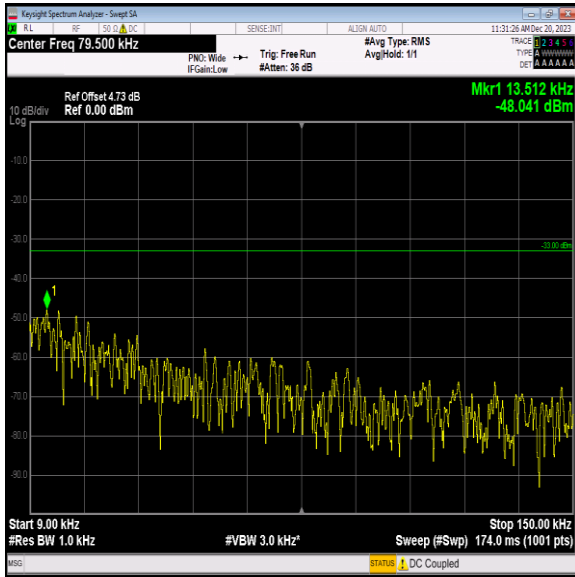
Band5_3MHz_64QAM_20525_1RB#0_0.009~0.15_0.009~0.1 5
