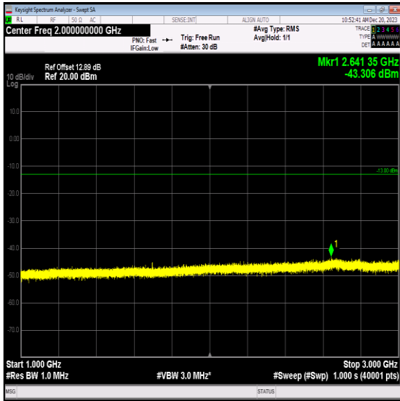
Band5_1.4MHz_16QAM_20643_1RB#0_1000~3000_1000~3000
