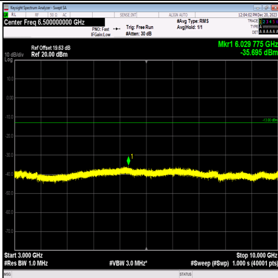
Band5_5MHz_QPSK_20425_1RB#0_3000~10000_3000~100
