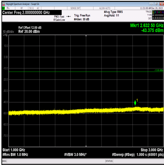
Band5_3MHz_16QAM_20525_1RB#0_1000~3000_1000~3000 0
