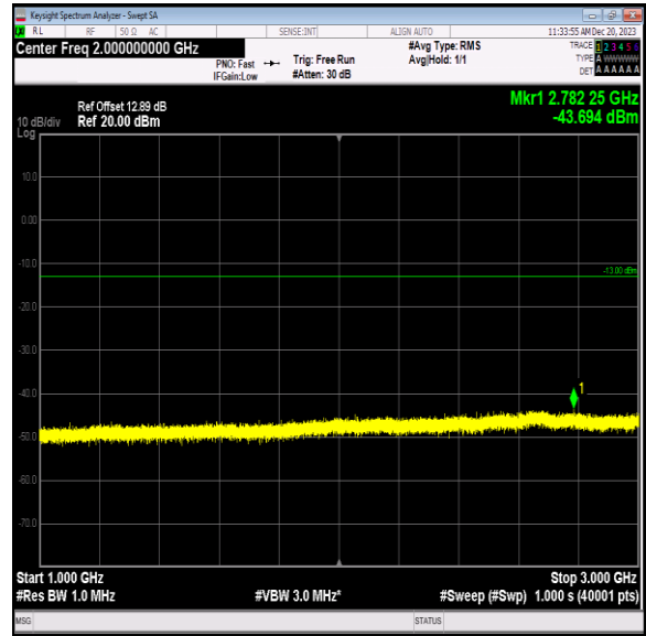
Band5_3MHz_16QAM_20635_1RB#0_1000~3000_1000~3000 0
