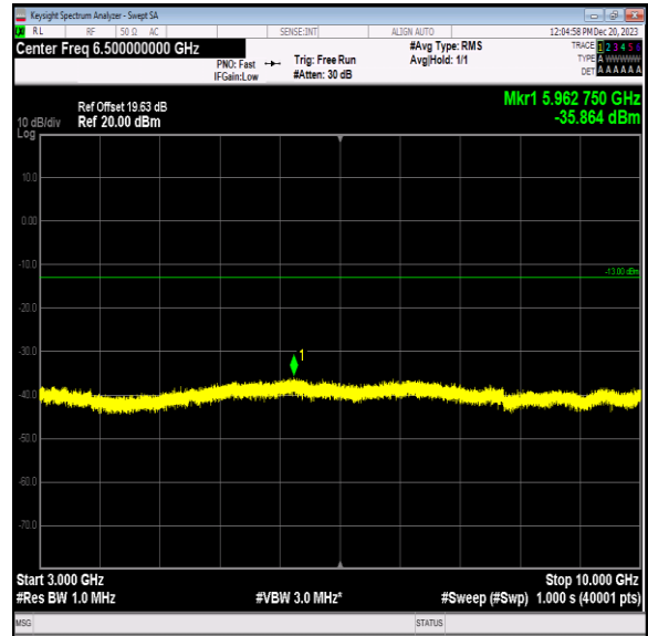
Band5_5MHz_16QAM_20425_1RB#0_3000~10000_3000~10000 000
