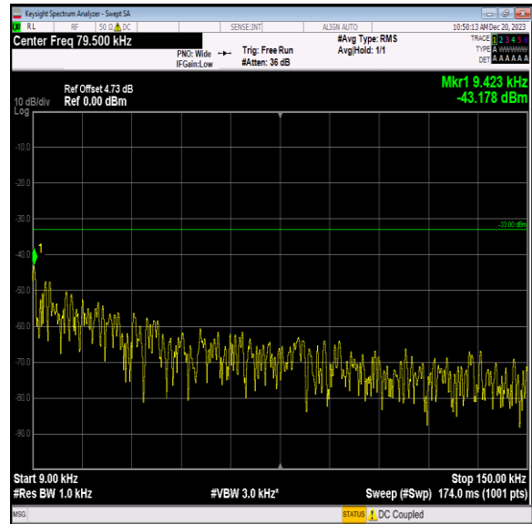
Band5_1.4MHz_64QAM_20525_1RB#0_0.009~0.15_0.009~0.15
