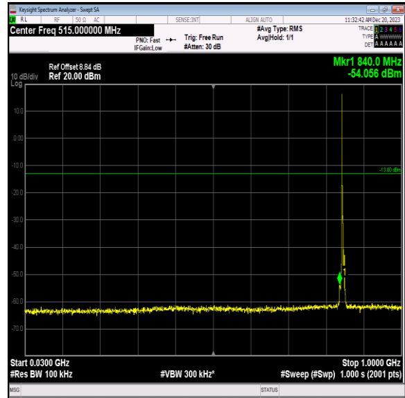
Band5_3MHz_QPSK_20635_1RB#0_30~1000_30~1000
