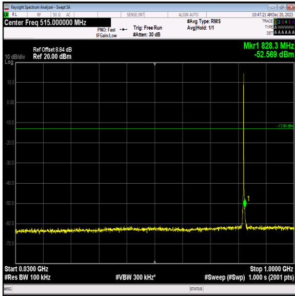
Band5_1.4MHz_64QAM_20407_1RB#0_30~1000_30~1000
