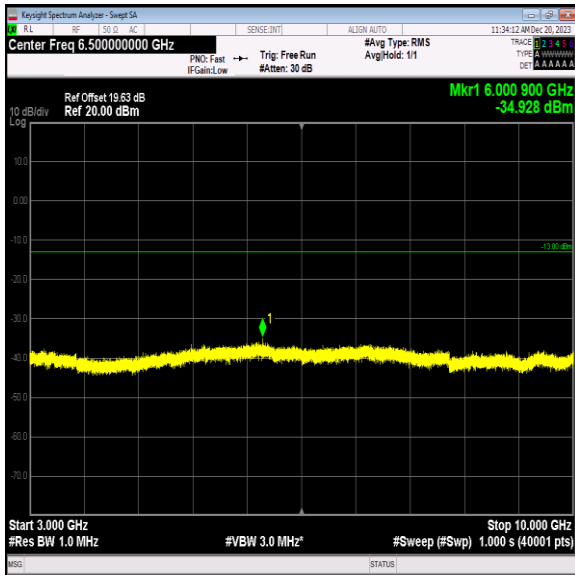
Band5_3MHz_16QAM_20635_1RB#0_3000~10000_3000~10000
