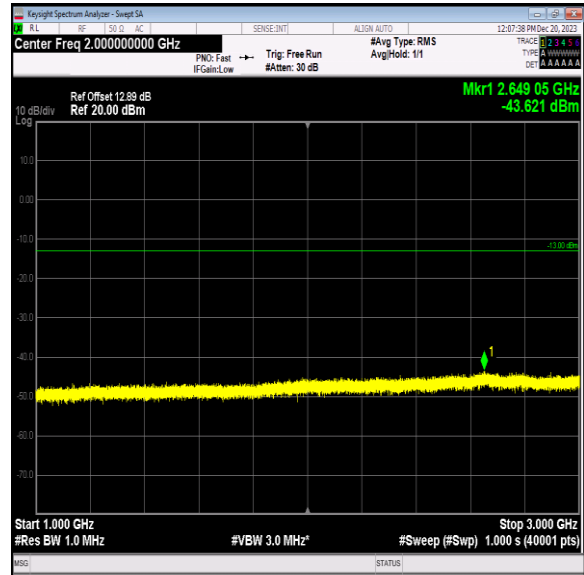
Band5_5MHz_16QAM_20525_1RB#0_1000~3000_1000~3000 0
