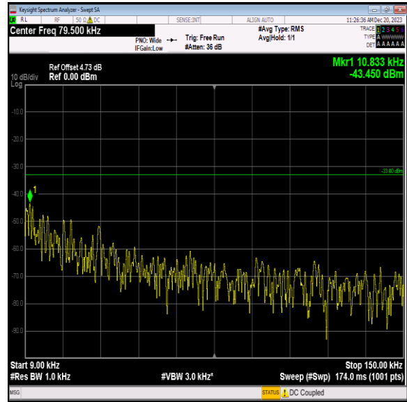
Band5_3MHz_QPSK_20415_1RB#0_0.009~0.15_0.009~0.15
