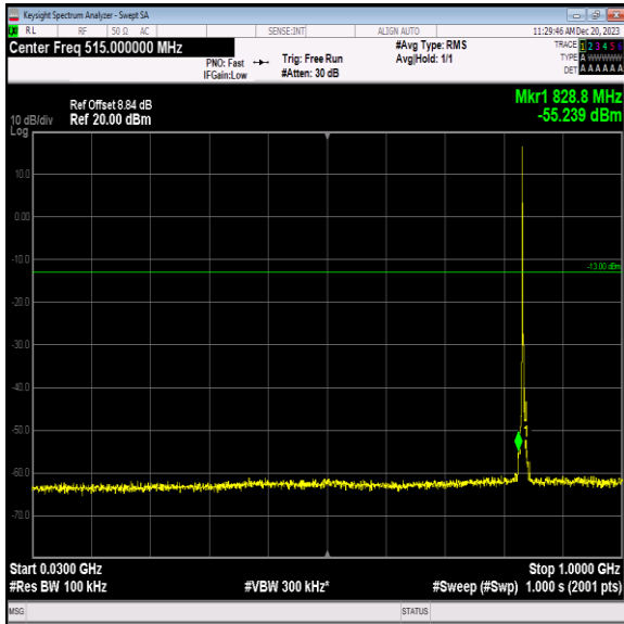
Band5_3MHz_QPSK_20525_1RB#0_30~1000_30~1000
