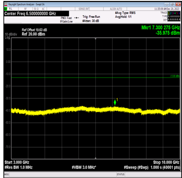
Band5_3MHz_64QAM_20635_1RB#0_3000~10000_3000~10000 000
