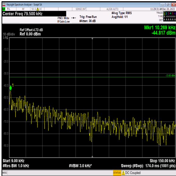
Band5_3MHz_QPSK_20525_1RB#0_0.009~0.15_0.009~0.15
