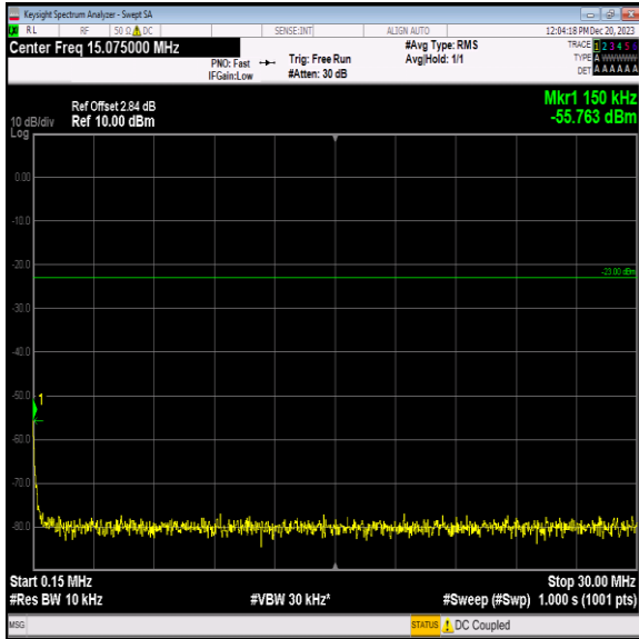
Band5_5MHz_16QAM_20425_1RB#0_0.15~30_0.15~30
