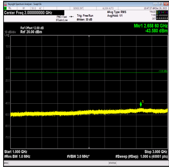
Band5_1.4MHz_64QAM_20407_1RB#0_1000~3000_1000~3000
