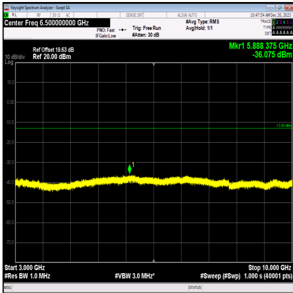
Band5_1.4MHz_64QAM_20407_1RB#0_3000~10000_3000~10000
