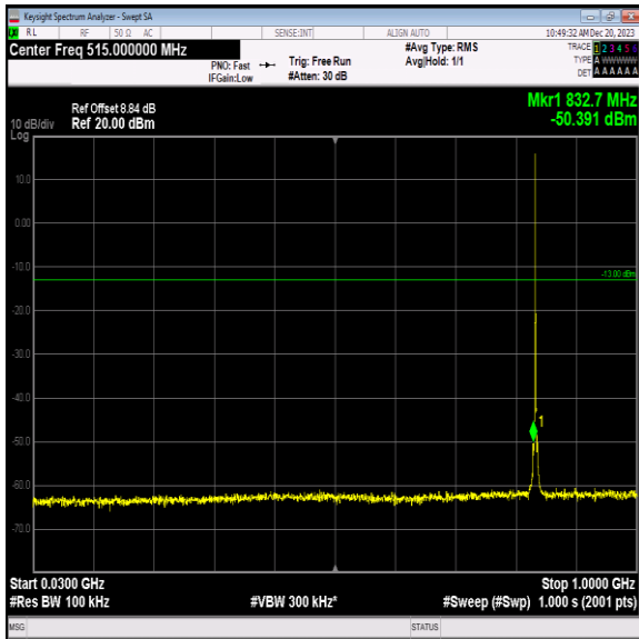
Band5_1.4MHz_16QAM_20525_1RB#0_30~1000_30~1000
