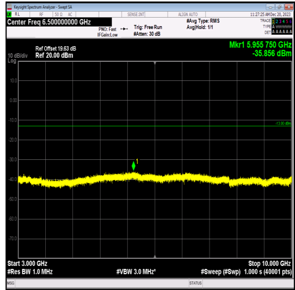
Band5_3MHz_QPSK_20415_1RB#0_3000~10000_3000~10000
