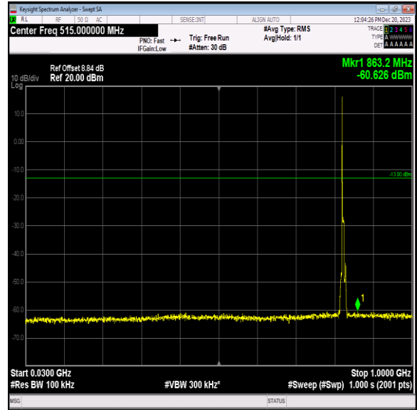
Band5_5MHz_16QAM_20425_1RB#0_30~1000_30~1000
