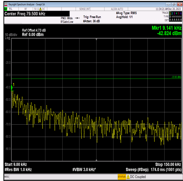
Band5_3MHz_64QAM_20635_1RB#0_0.009~0.15_0.009~0.15
