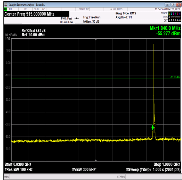
Band5_3MHz_64QAM_20635_1RB#0_30~1000_30~1000
