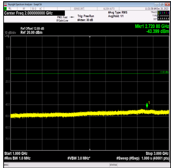
Band5_3MHz_64QAM_20525_1RB#0_1000~3000_1000~300 0
