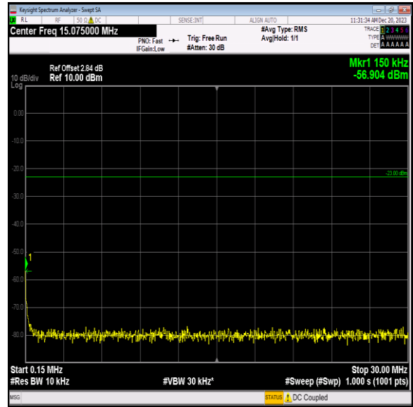
Band5_3MHz_64QAM_20525_1RB#0_0.15~30_0.15~30
