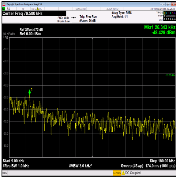
Band5_1.4MHz_16QAM_20525_1RB#0_0.009~0.15_0.009~0.15
