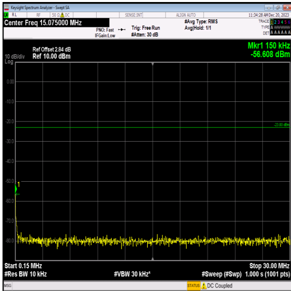
Band5_3MHz_64QAM_20635_1RB#0_0.15~30_0.15~30
