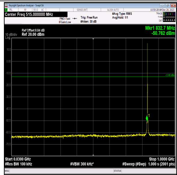
Band5_1.4MHz_64QAM_20525_1RB#0_30~1000_30~1000
