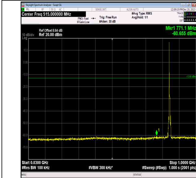
Band5_5MHz_QPSK_20625_1RB#0_30~1000_30~1000
