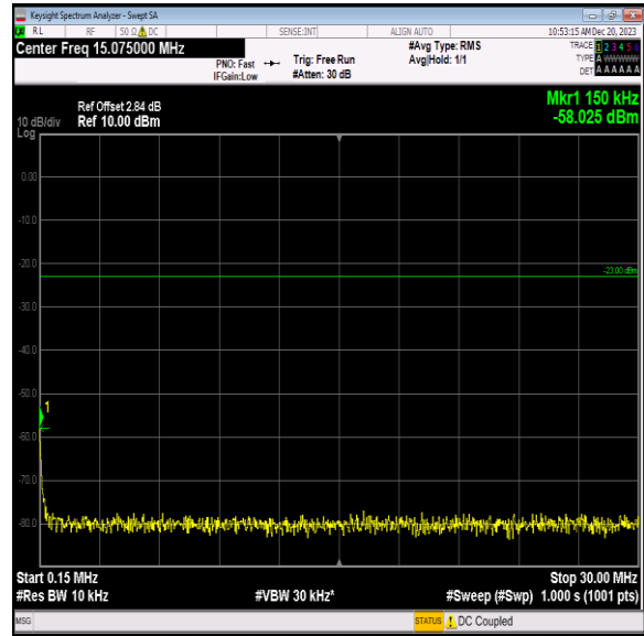
Band5_1.4MHz_64QAM_20643_1RB#0_0.15~30_0.15~30
