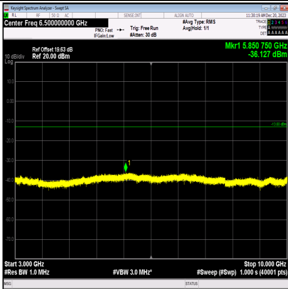
Band5_3MHz_QPSK_20525_1RB#0_3000~10000_3000~100
