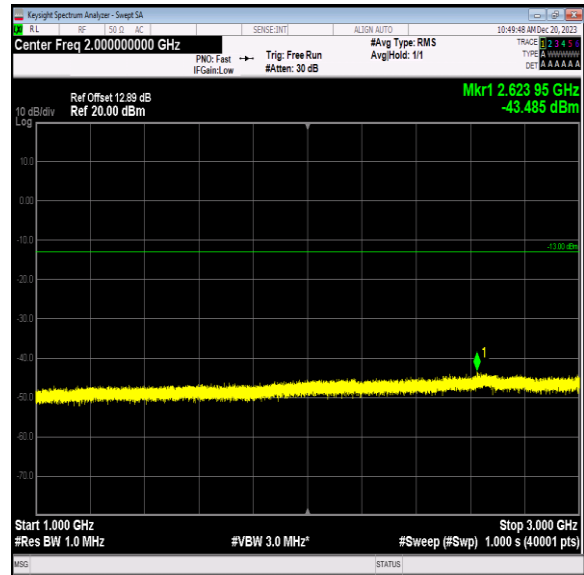
Band5_1.4MHz_16QAM_20525_1RB#0_1000~3000_1000~3000
