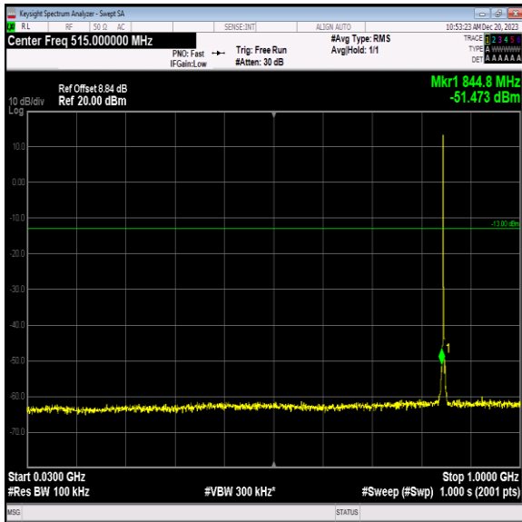
Band5_1.4MHz_64QAM_20643_1RB#0_30~1000_30~1000
