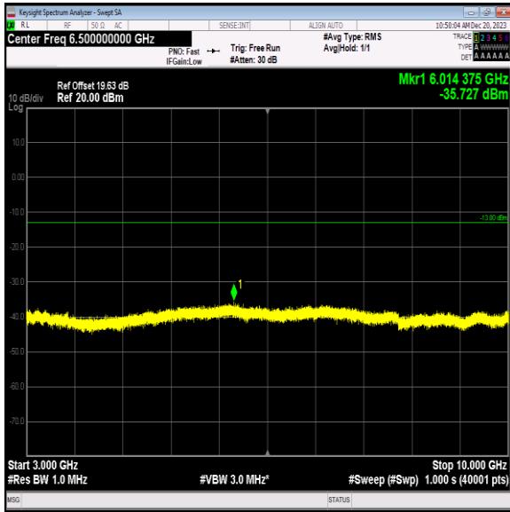
Band5_1.4MHz_16QAM_20525_1RB#0_3000~10000_3000~10000
