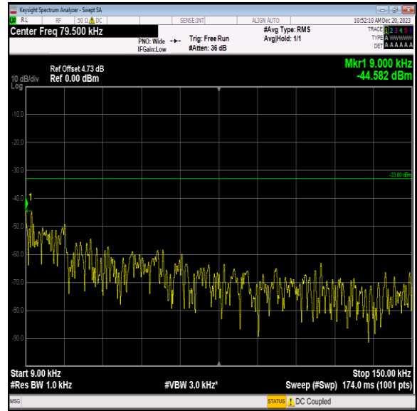
Band5_1.4MHz_16QAM_20643_1RB#0_0.009~0.15_0.009~0.15
