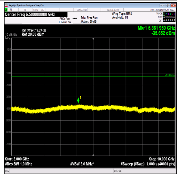
Band5_1.4MHz_64QAM_20525_1RB#0_3000~10000_3000~10000
