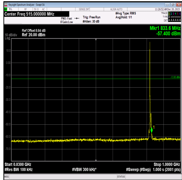
Band5_3MHz_QPSK_20415_1RB#0_30~1000_30~1000
