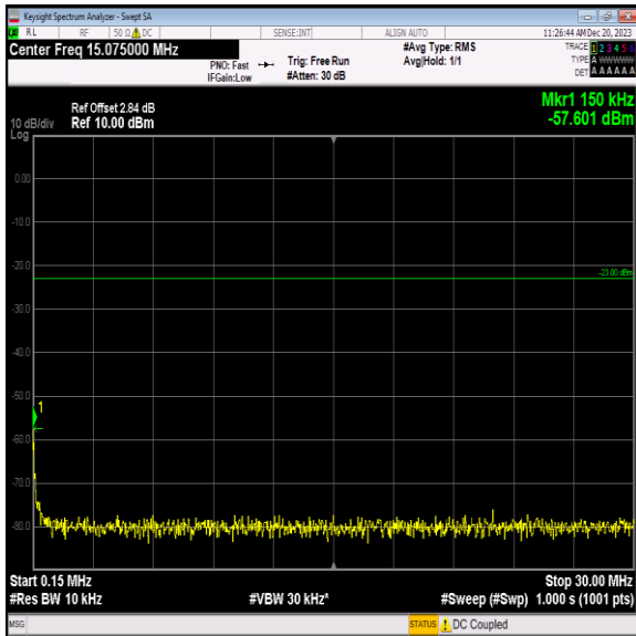
Band5_3MHz_QPSK_20415_1RB#0_0.15~30_0.15~30
