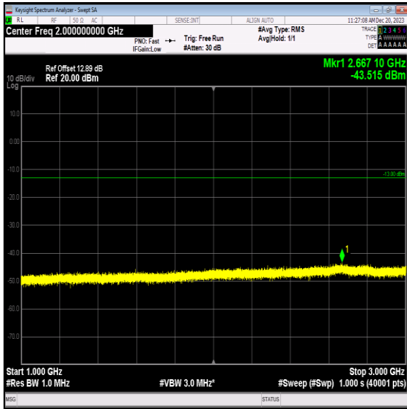
Band5_3MHz_QPSK_20415_1RB#0_1000~3000_1000~3000
