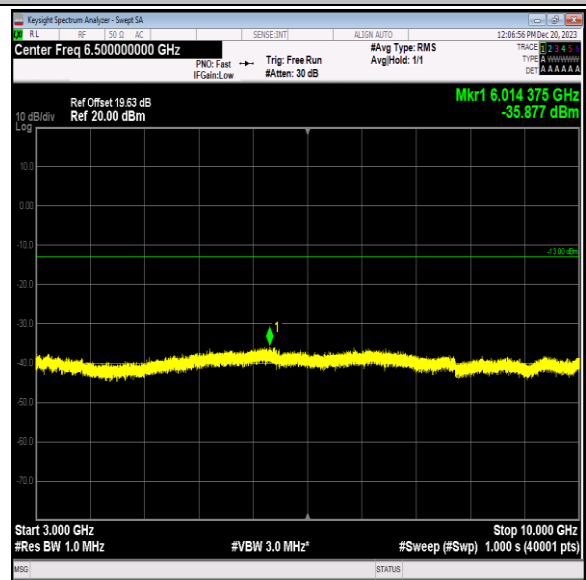
Band5_5MHz_QPSK_20525_1RB#0_3000~10000_3000~10000
