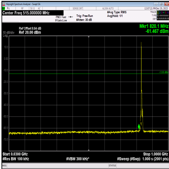
Band5_5MHz_16QAM_20525_1RB#0_30~1000_30~1000
