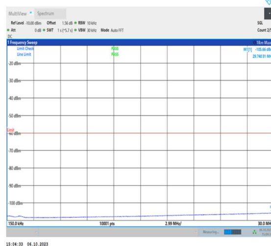
1-N48-PC3-30-30-L-1-DFT-QPSK- Edge_1RB_Left-1@0-0.15-30-Ant2-29.74--105.66- -60-PASS
