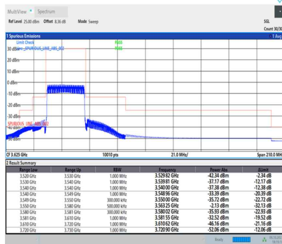
1-N48-PC3-30-30-L-6-CP-QPSK-Outer_Full- 78@0-Ant2-1--PASS-see graph
