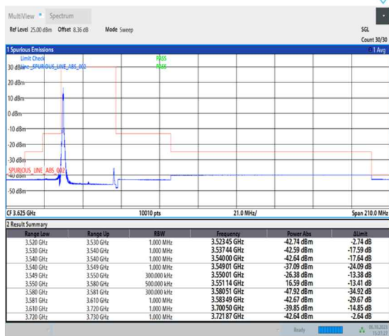
1-N48-PC3-30-30-L-4-CP-QPSK-Edge_1RB_Left- 1@0-Ant2-1--PASS-see graph
