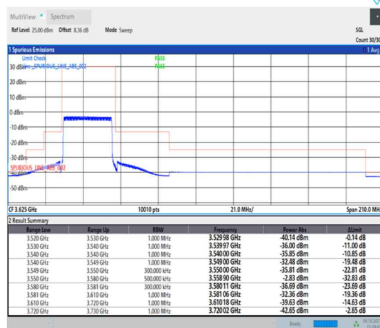
1-N48-PC3-30-30-L-3-DFT-PI2BPSK- Outer_Full-75@0-Ant2-1--PASS-see graph
