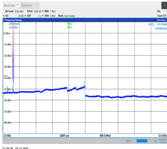
1-N48-PC3-30-30-L-1-DFT-QPSK- Edge_1RB_Left-1@0-3000-12000-Ant2-7479.30- -47.19--40-PASS
