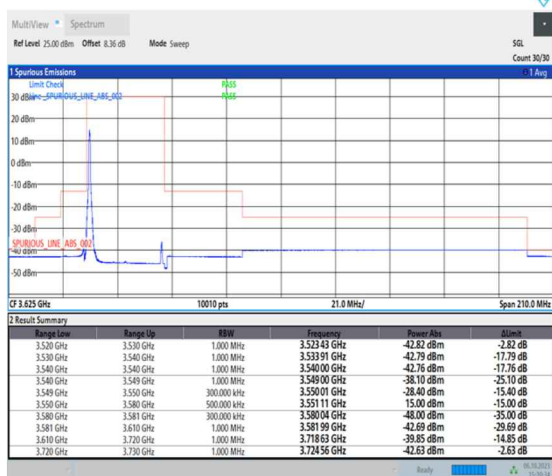
1-N48-PC3-30-30-L-1-DFT-PI2BPSK- Edge_1RB_Left-1@0-Ant2-1--PASS-see graph
