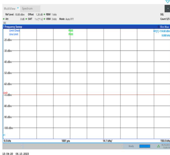
1-N48-PC3-30-30-L-1-DFT-QPSK- Edge_1RB_Left-1@0-0.009-0.15-Ant2-0.01-- 114.60--70-PASS
