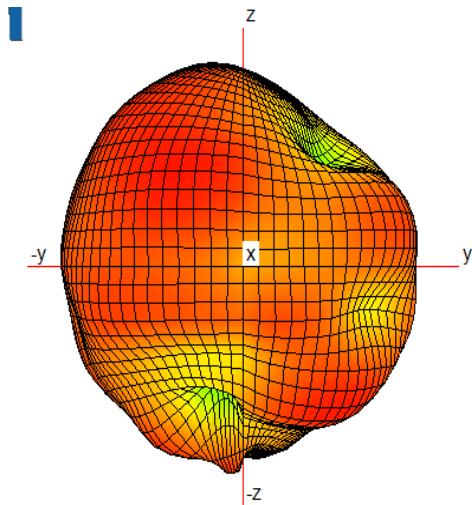
3D Antenna Pattern
