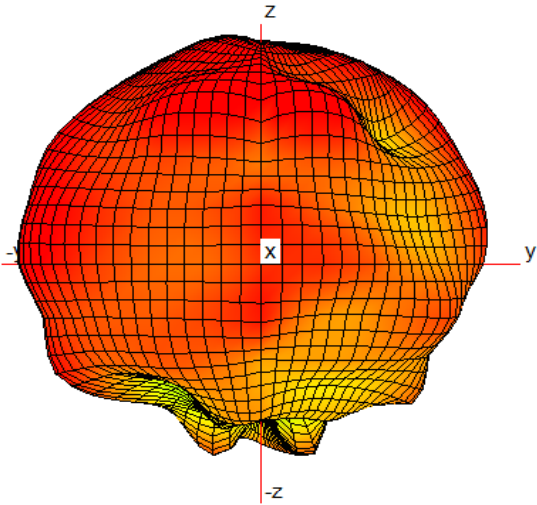
3D Antenna Pattern
