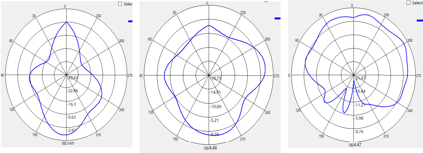
2D Antenna Pattern (X->Y;X->Z;Y->Z)
