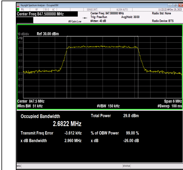
Band5-3MHz-16QAM-20635-15RB#0-PASS
