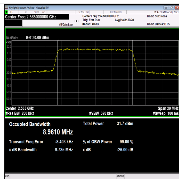
Band7-10MHz-QPSK-21400-50RB#0-PASS
