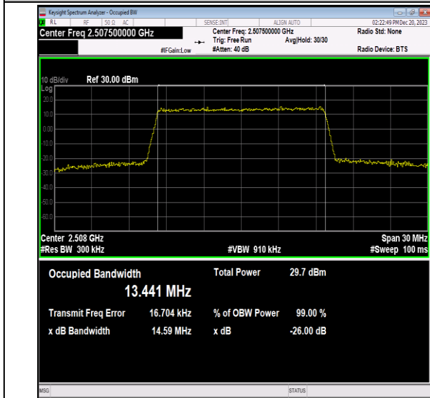
Band7-15MHz-64QAM-20825-75RB#0-PASS
