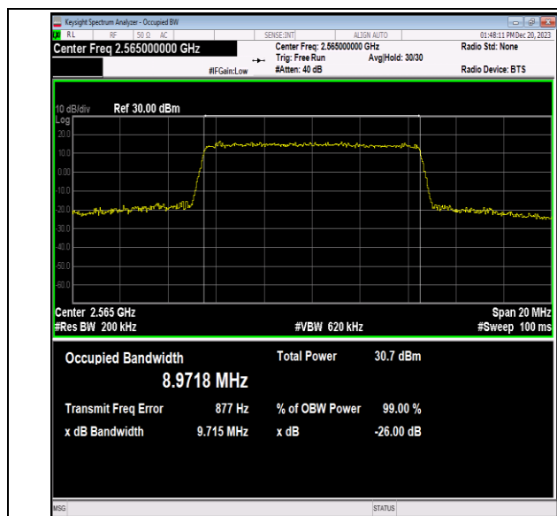
Band7-10MHz-16QAM-21400-50RB#0-PASS
