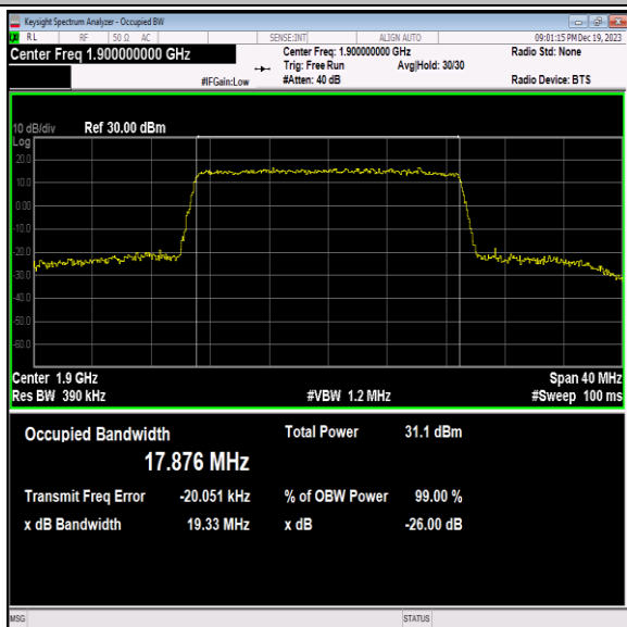
Band2-20MHz-16QAM-19100-100RB#0-PASS
