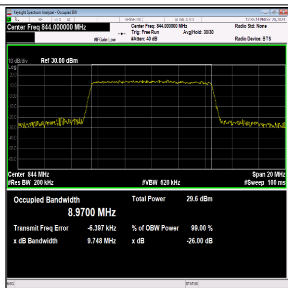
Band5-10MHz-64QAM-20600-50RB#0-PASS
