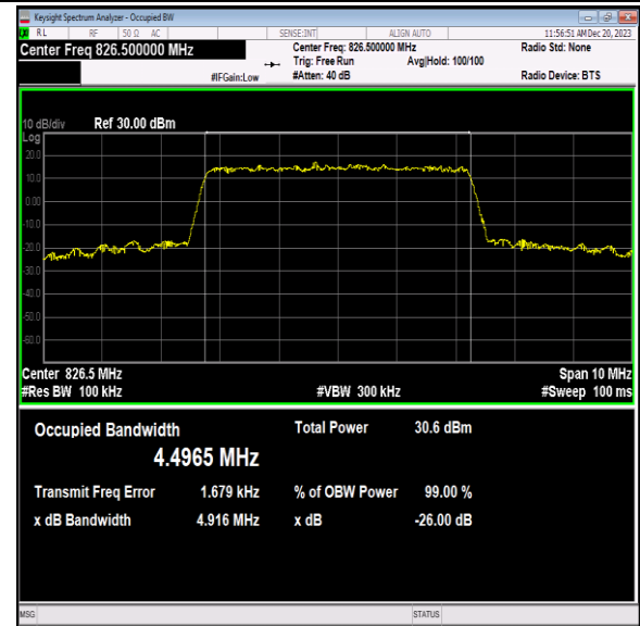
Band5-5MHz-16QAM-20425-25RB#0-PASS
