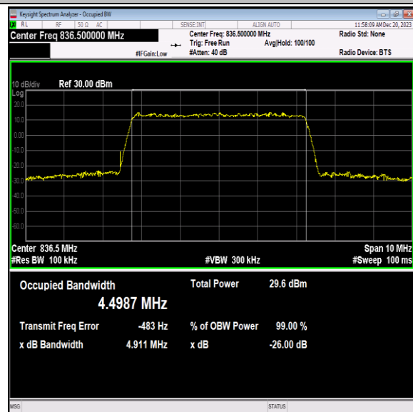
Band5-5MHz-64QAM-20525-25RB#0-PASS
