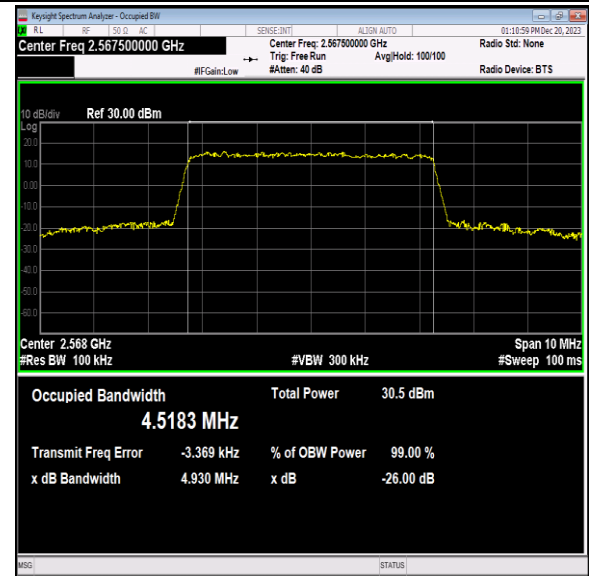
Band7-5MHz-16QAM-21425-25RB#0-PASS
