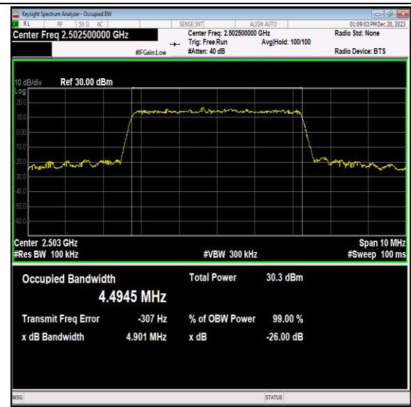
Band7-5MHz-16QAM-20775-25RB#0-PASS
