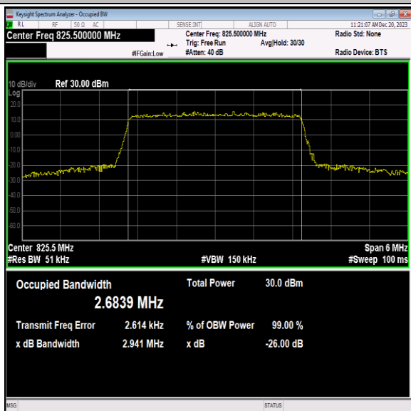
Band5-3MHz-16QAM-20415-15RB#0-PASS
