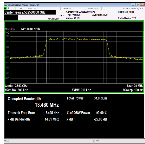
Band7-15MHz-16QAM-21375-75RB#0-PASS
