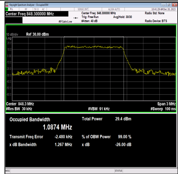
Band5-1.4MHz-16QAM-20643-6RB#0-PASS
