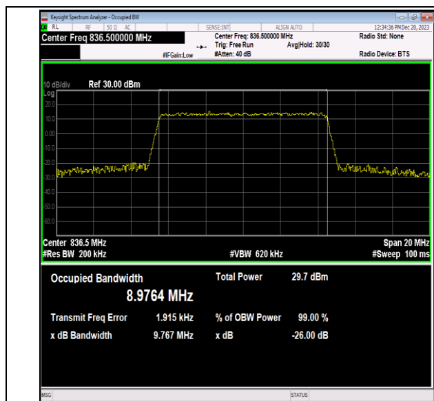
Band5-10MHz-64QAM-20525-50RB#0-PASS
