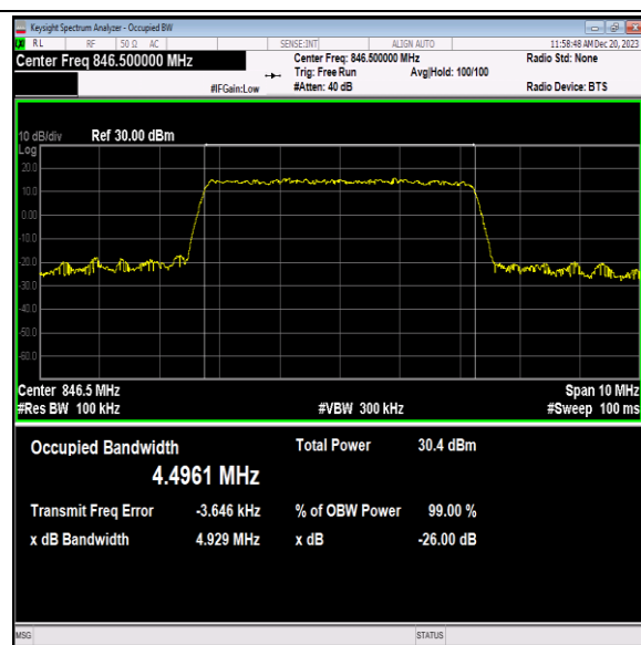
Band5-5MHz-16QAM-20625-25RB#0-PASS
