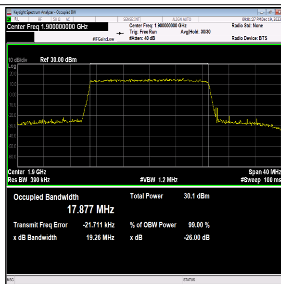
Band2-20MHz-64QAM-19100-100RB#0-PASS
