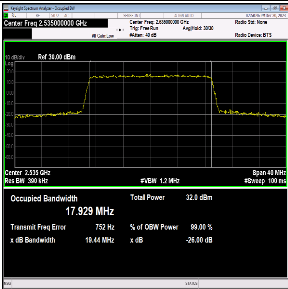
Band7-20MHz-QPSK-21100-100RB#0-PASS
