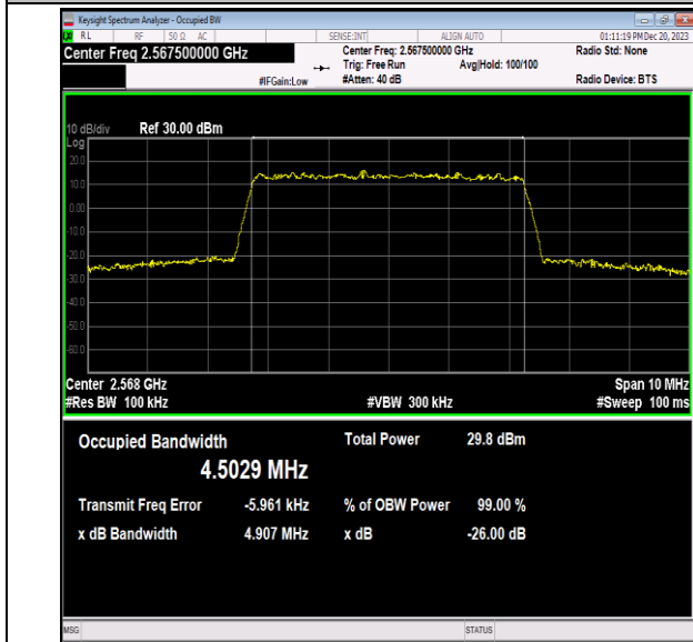
Band7-5MHz-64QAM-21425-25RB#0-PASS
