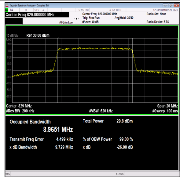
Band5-10MHz-64QAM-20450-50RB#0-PASS
