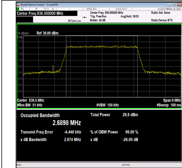
Band5-3MHz-64QAM-20525-15RB#0-PASS
