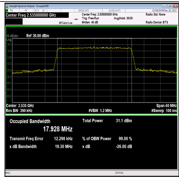
Band7-20MHz-16QAM-21100-100RB#0-PASS
