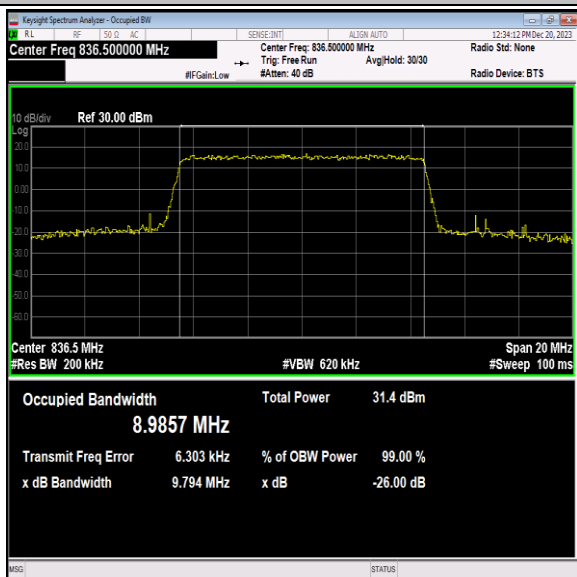
Band5-10MHz-QPSK-20525-50RB#0-PASS
