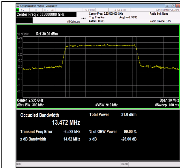
Band7-15MHz-16QAM-21100-75RB#0-PASS
