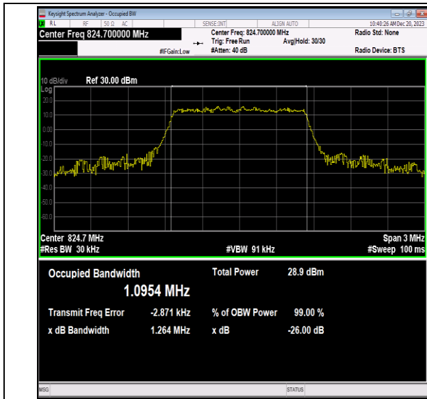
Band5-1.4MHz-64QAM-20407-6RB#0-PASS
