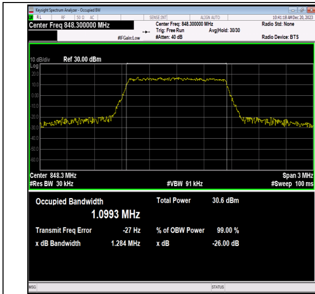
Band5-1.4MHz-QPSK-20643-6RB#0-PASS
