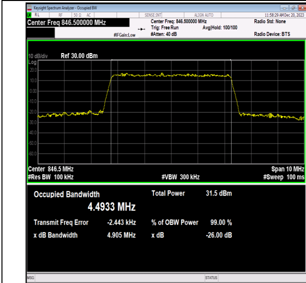
Band5-5MHz-QPSK-20625-25RB#0-PASS
