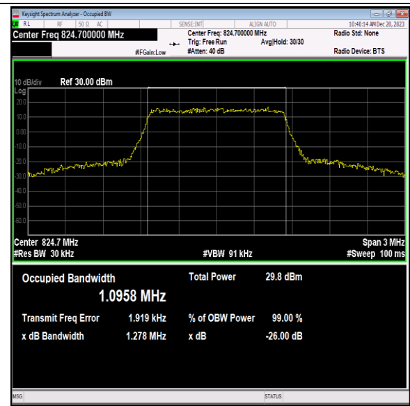
Band5-1.4MHz-16QAM-20407-6RB#0-PASS
