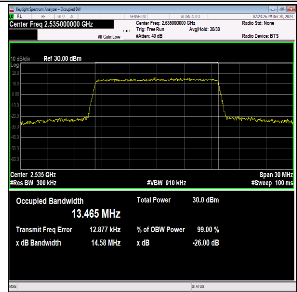
Band7-15MHz-64QAM-21100-75RB#0-PASS
