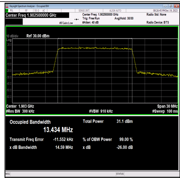
Band2-15MHz-16QAM-19125-75RB#0-PASS
