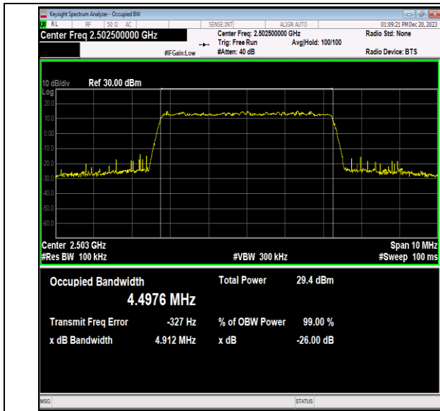
Band7-5MHz-64QAM-20775-25RB#0-PASS
