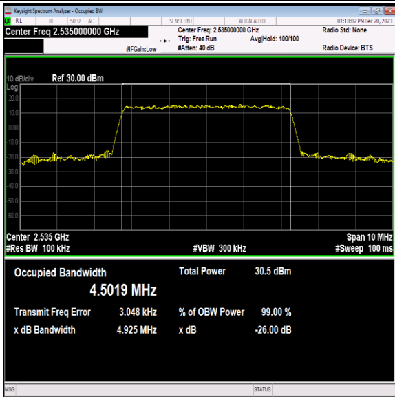
Band7-5MHz-16QAM-21100-25RB#0-PASS
