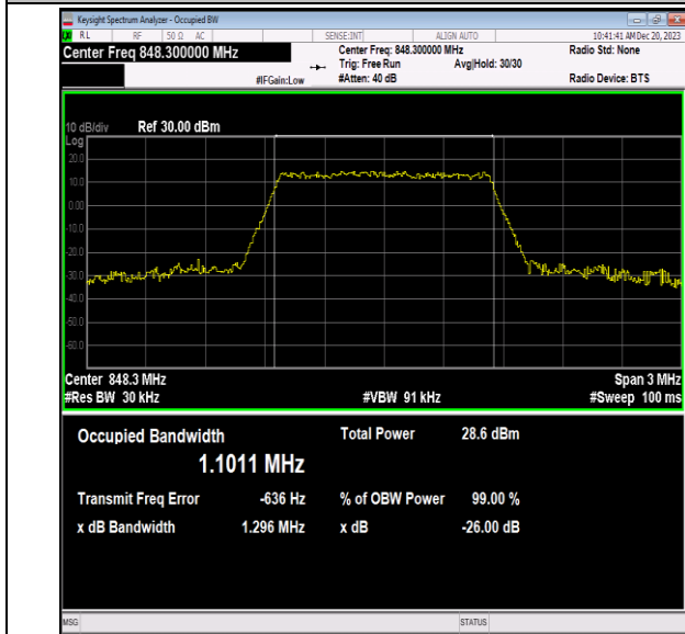
Band5-1.4MHz-64QAM-20643-6RB#0-PASS
