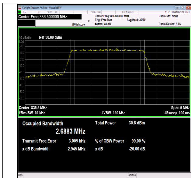
Band5-3MHz-QPSK-20525-15RB#0-PASS
