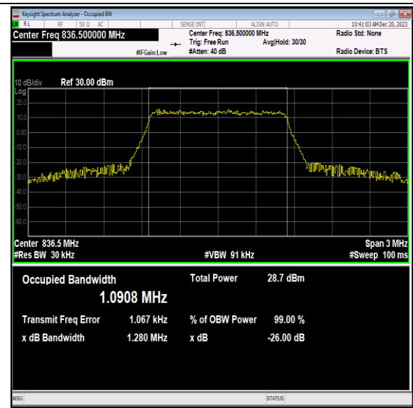
Band5-1.4MHz-64QAM-20525-6RB#0-PASS
