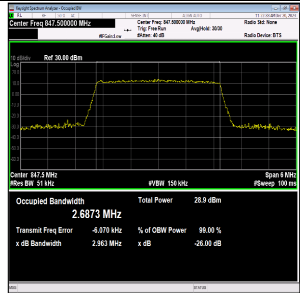
Band5-3MHz-64QAM-20635-15RB#0-PASS
