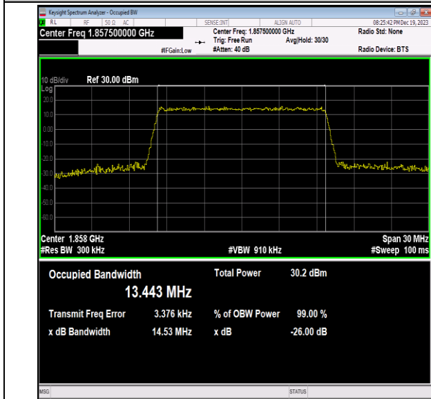
Band2-15MHz-64QAM-18675-75RB#0-PASS
