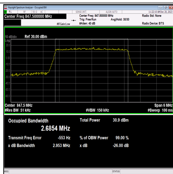
Band5-3MHz-QPSK-20635-15RB#0-PASS
