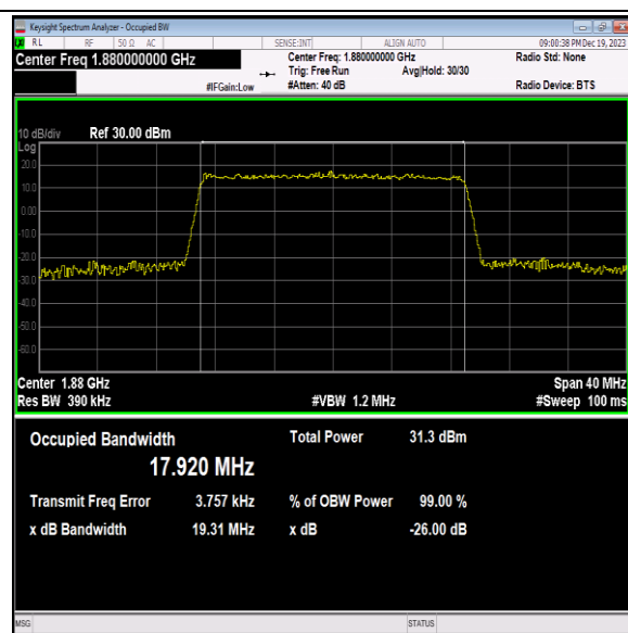
Band2-20MHz-16QAM-18900-100RB#0-PASS
