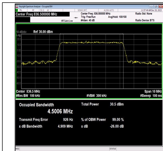
Band5-5MHz-16QAM-20525-25RB#0-PASS
