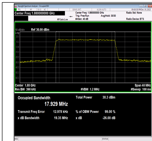
Band2-20MHz-64QAM-18900-100RB#0-PASS
