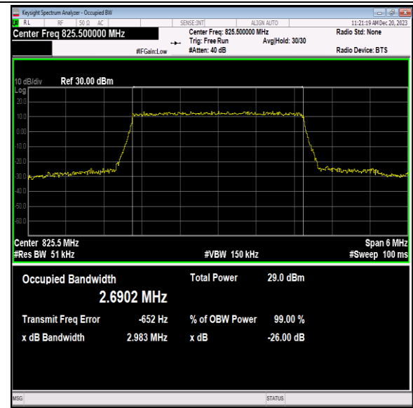
Band5-3MHz-64QAM-20415-15RB#0-PASS
