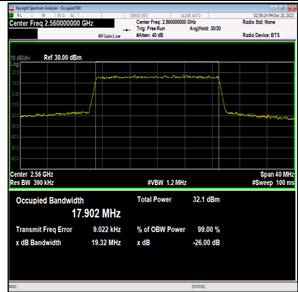
Band7-20MHz-QPSK-21350-100RB#0-PASS
