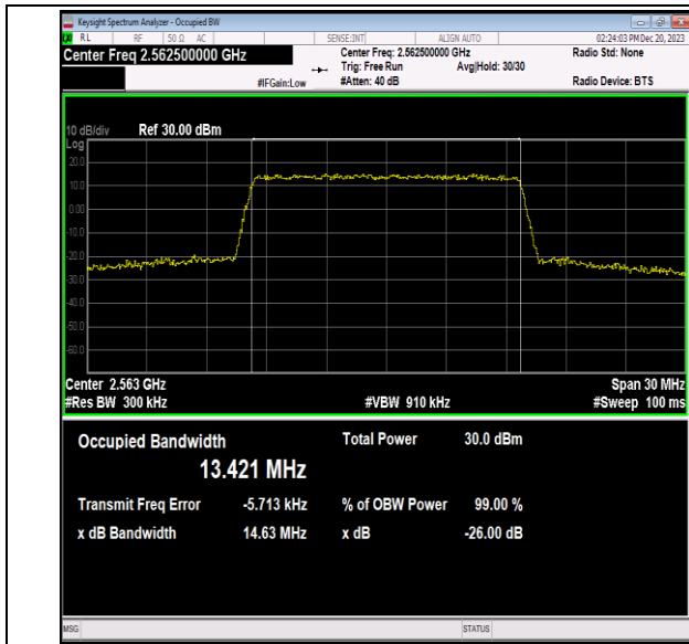
Band7-15MHz-64QAM-21375-75RB#0-PASS
