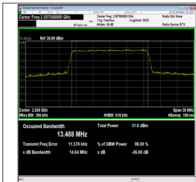
Band7-15MHz-QPSK-20825-75RB#0-PASS
