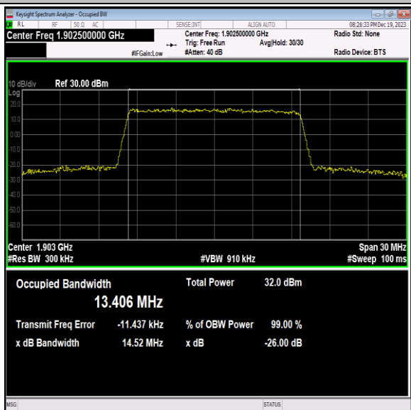
Band2-15MHz-QPSK-19125-75RB#0-PASS
