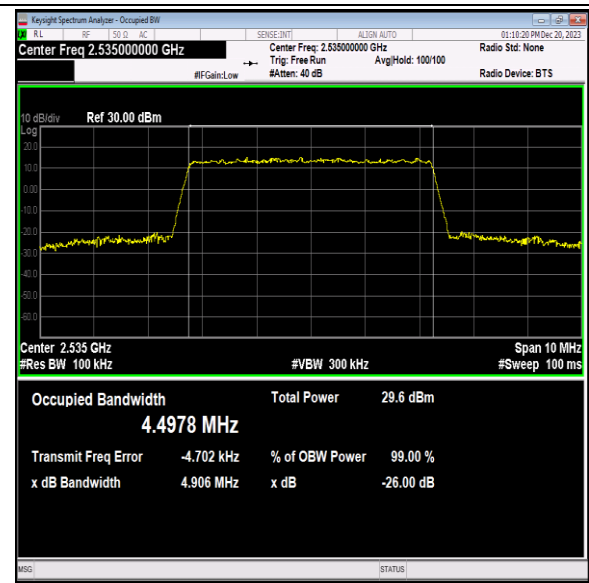
Band7-5MHz-64QAM-21100-25RB#0-PASS
