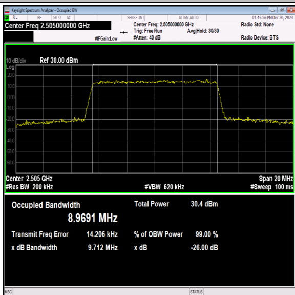
Band7-10MHz-16QAM-20800-50RB#0-PASS
