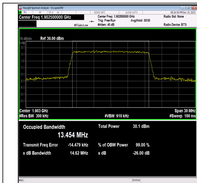
Band2-15MHz-64QAM-19125-75RB#0-PASS
