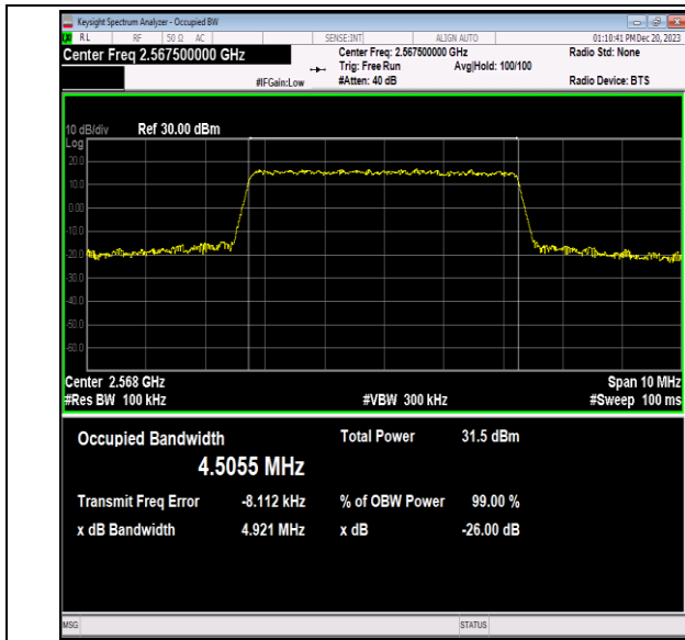
Band7-5MHz-QPSK-21425-25RB#0-PASS
