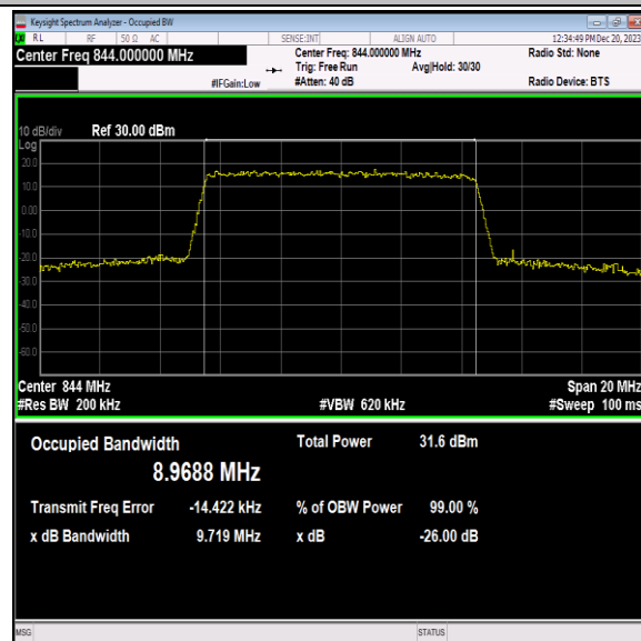
Band5-10MHz-QPSK-20600-50RB#0-PASS
