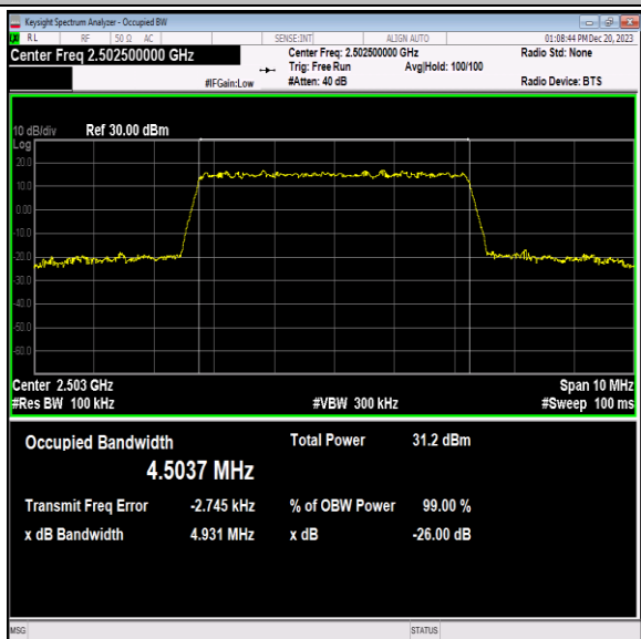
Band7-5MHz-QPSK-20775-25RB#0-PASS
