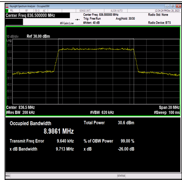
Band5-10MHz-16QAM-20525-50RB#0-PASS
