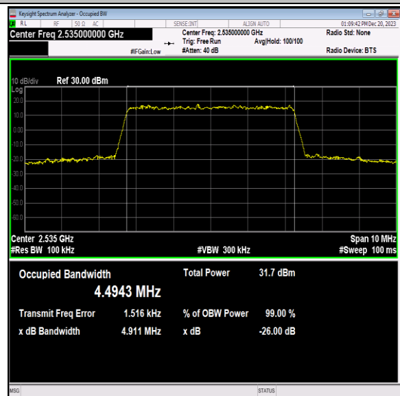
Band7-5MHz-QPSK-21100-25RB#0-PASS
