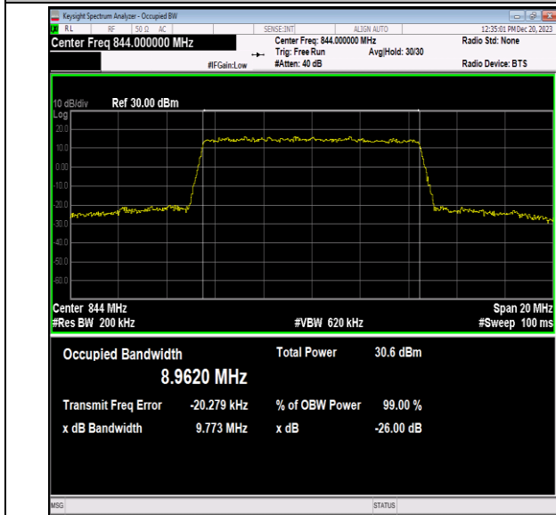
Band5-10MHz-16QAM-20600-50RB#0-PASS
