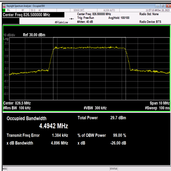
Band5-5MHz-64QAM-20425-25RB#0-PASS
