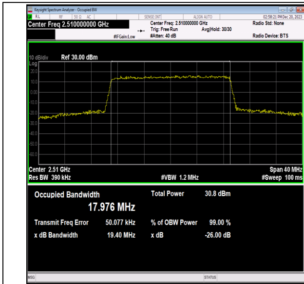
Band7-20MHz-16QAM-20850-100RB#0-PASS
