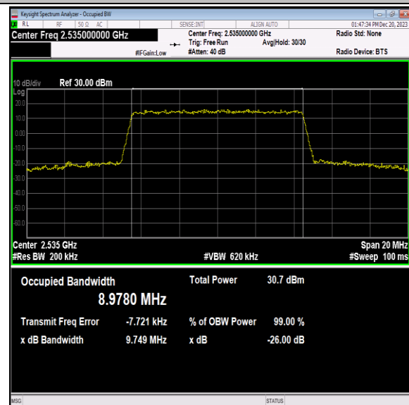
Band7-10MHz-16QAM-21100-50RB#0-PASS
