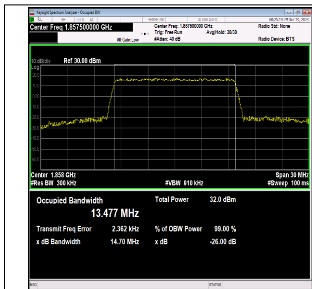
Band2-15MHz-QPSK-18675-75RB#0-PASS
