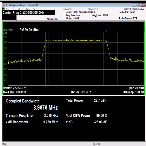
Band7-10MHz-64QAM-21100-50RB#0-PASS
