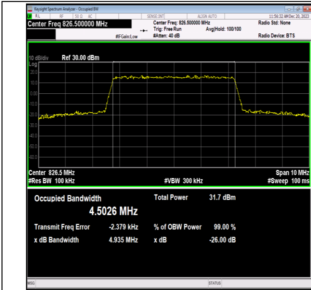
Band5-5MHz-QPSK-20425-25RB#0-PASS
