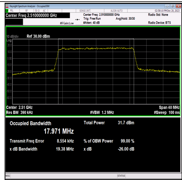
Band7-20MHz-QPSK-20850-100RB#0-PASS
