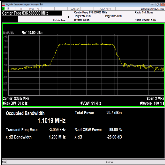
Band5-1.4MHz-16QAM-20525-6RB#0-PASS
