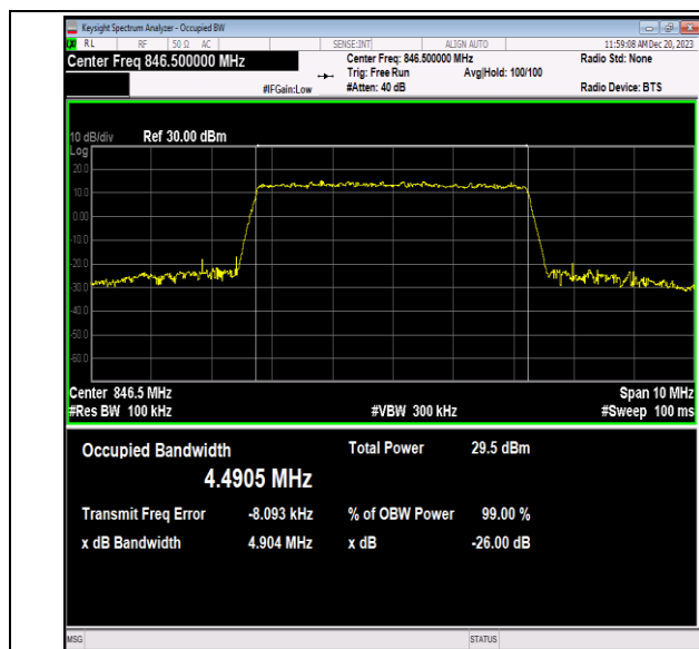
Band5-5MHz-64QAM-20625-25RB#0-PASS
