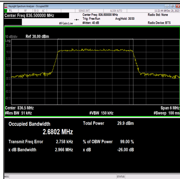
Band5-3MHz-16QAM-20525-15RB#0-PASS
