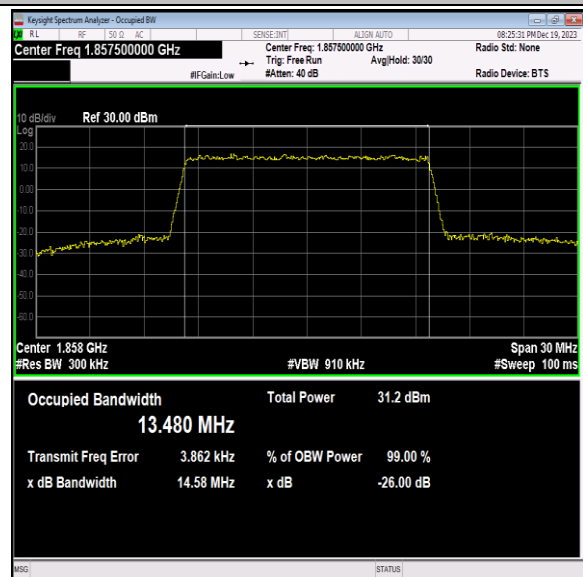
Band2-15MHz-16QAM-18675-75RB#0-PASS
