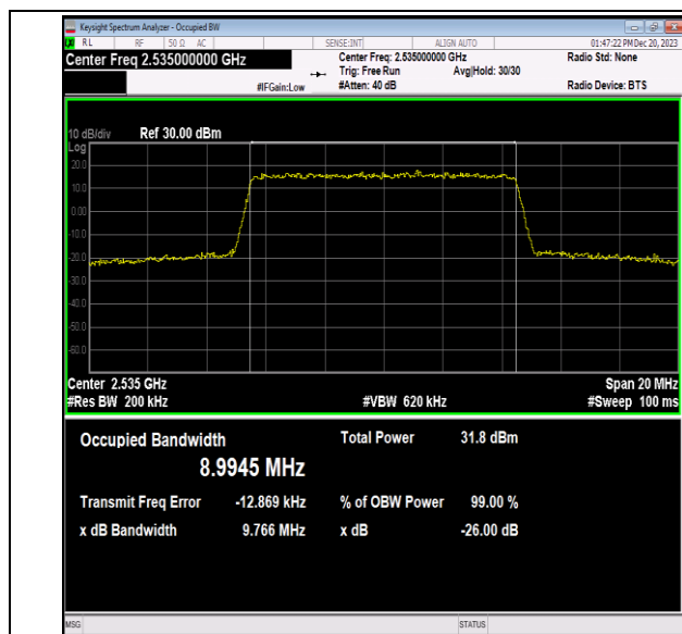
Band7-10MHz-QPSK-21100-50RB#0-PASS
