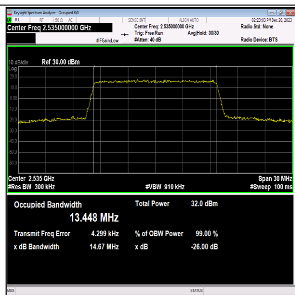
Band7-15MHz-QPSK-21100-75RB#0-PASS
