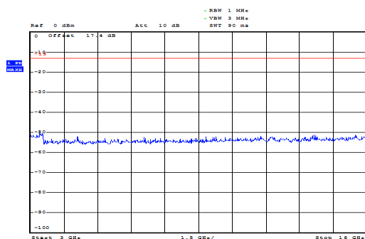
LTE Band 4 1.4MHz CH-Low 3GHz~18GHz
