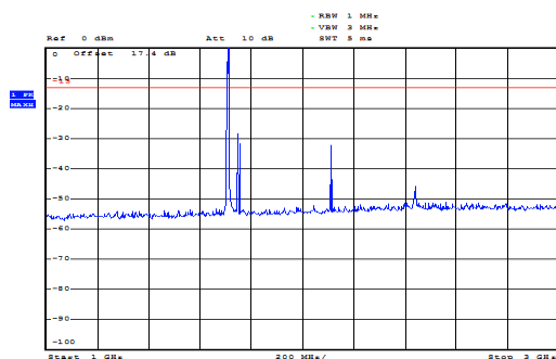
LTE Band 4 1.4MHz CH-Low 1GHz~3GHz
