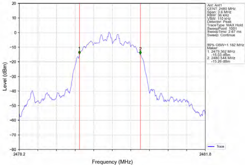
8DPSK_3DH5_HCH_2480MHz_Ant1_NTNV
