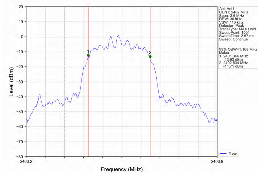
Pi/4DQPSK_2DH5_LCH_2402MHz_Ant1_NTNV
