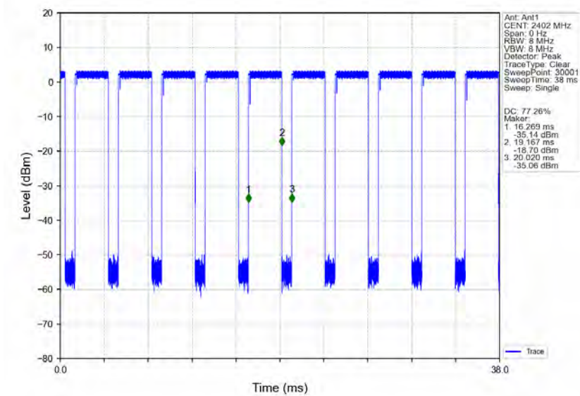
Pi/4DQPSK_2DH5_LCH_2402MHz_Ant1_NTNV
