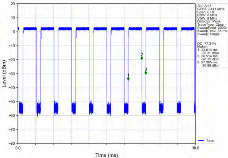
8DPSK_3DH5_MCH_2441MHz_Ant1_NTNV
