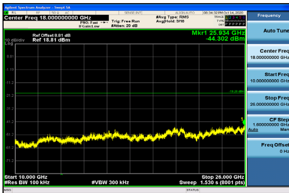
RF Conducted Spurious Emissions_RF4CE _2440
