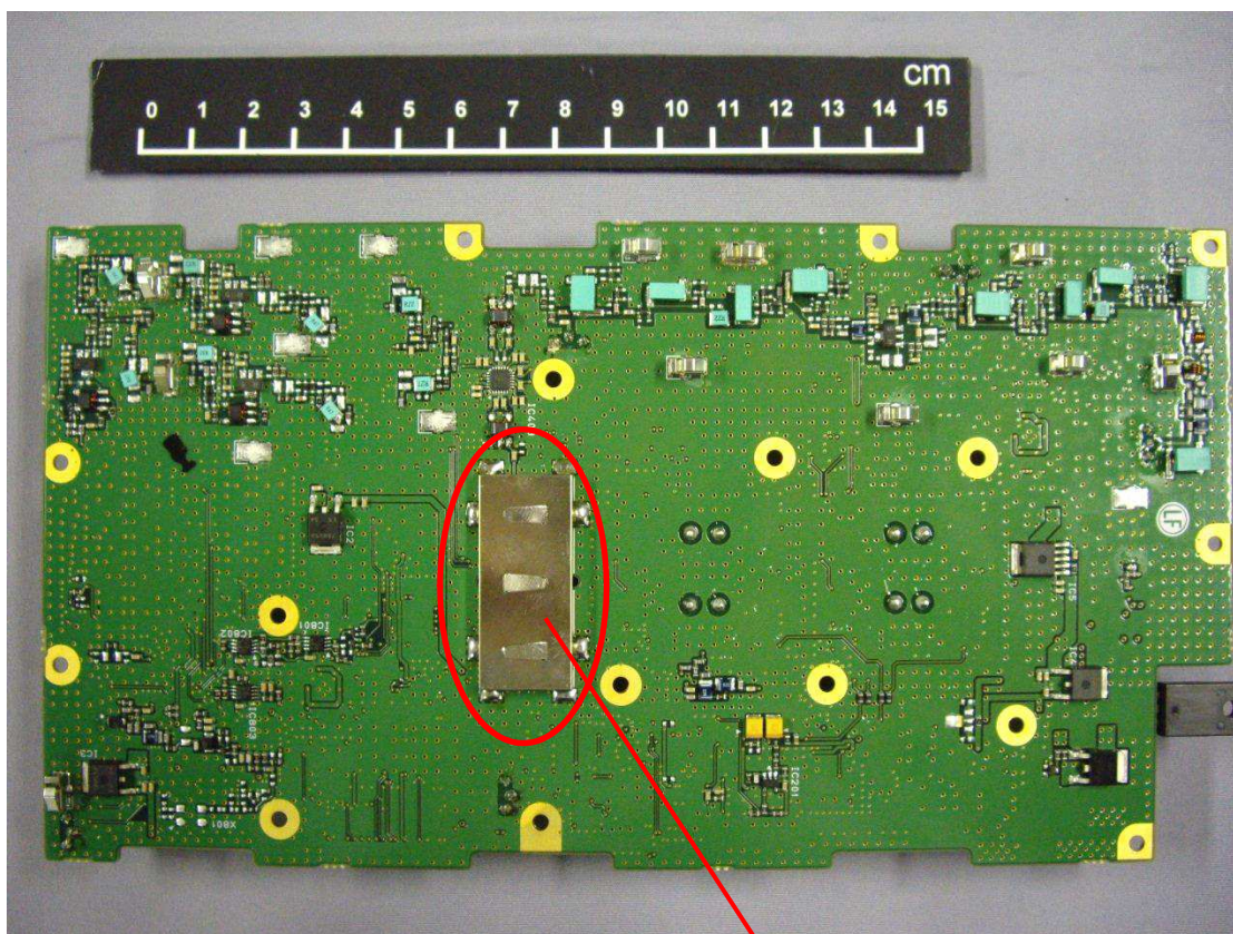
RX Bottom Side View with Shield
