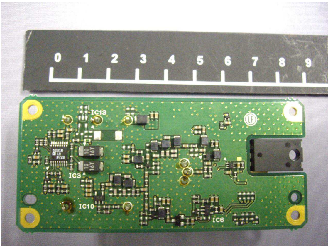
KXK-3 OCXO UNIT Bottom Side View
