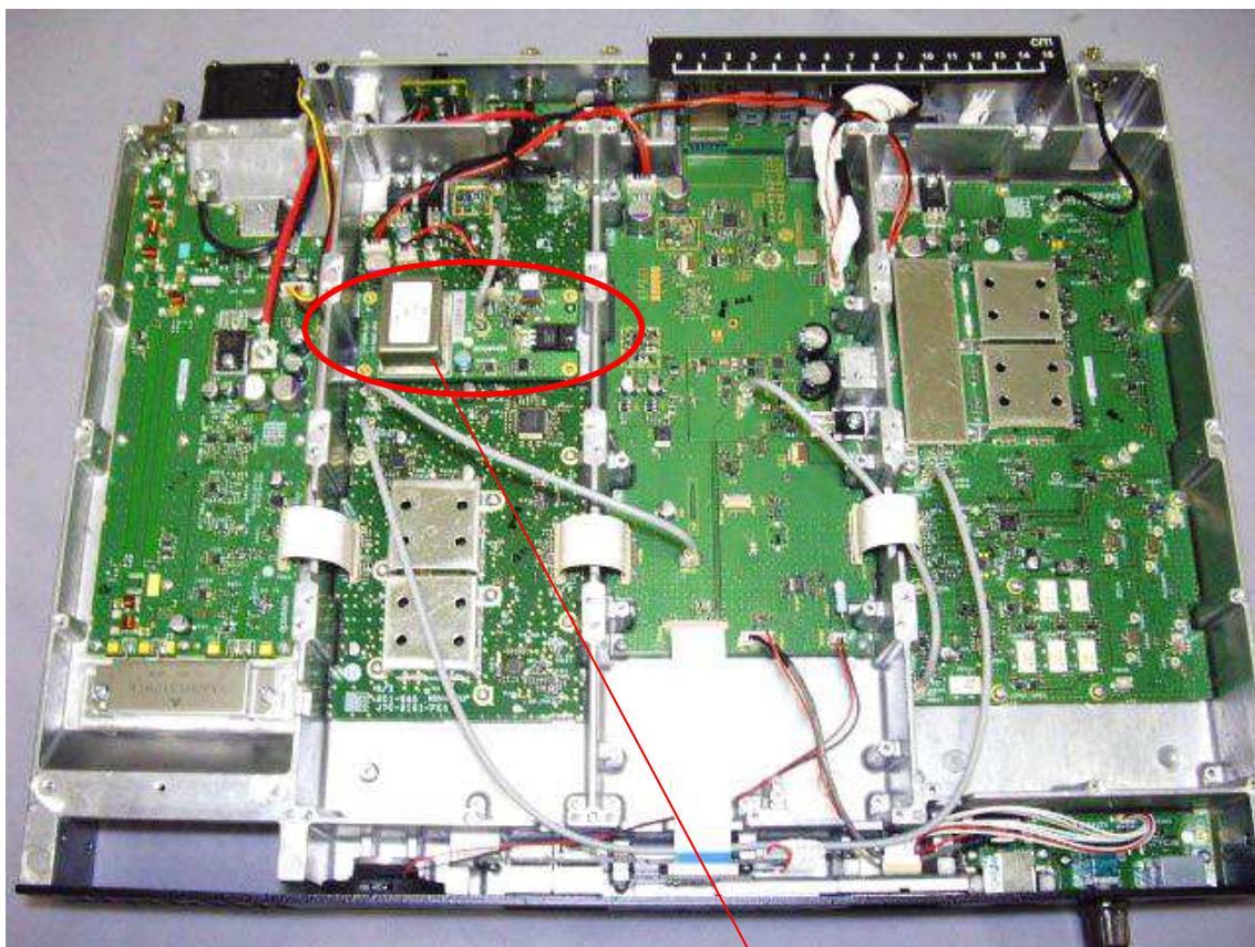
Upper Side View with OCXO Unit
