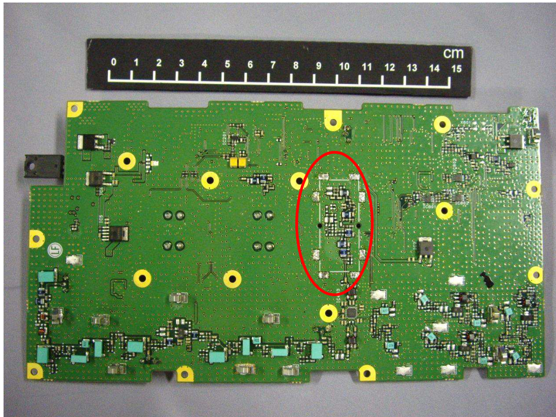
RX Bottom Side View without Shield
