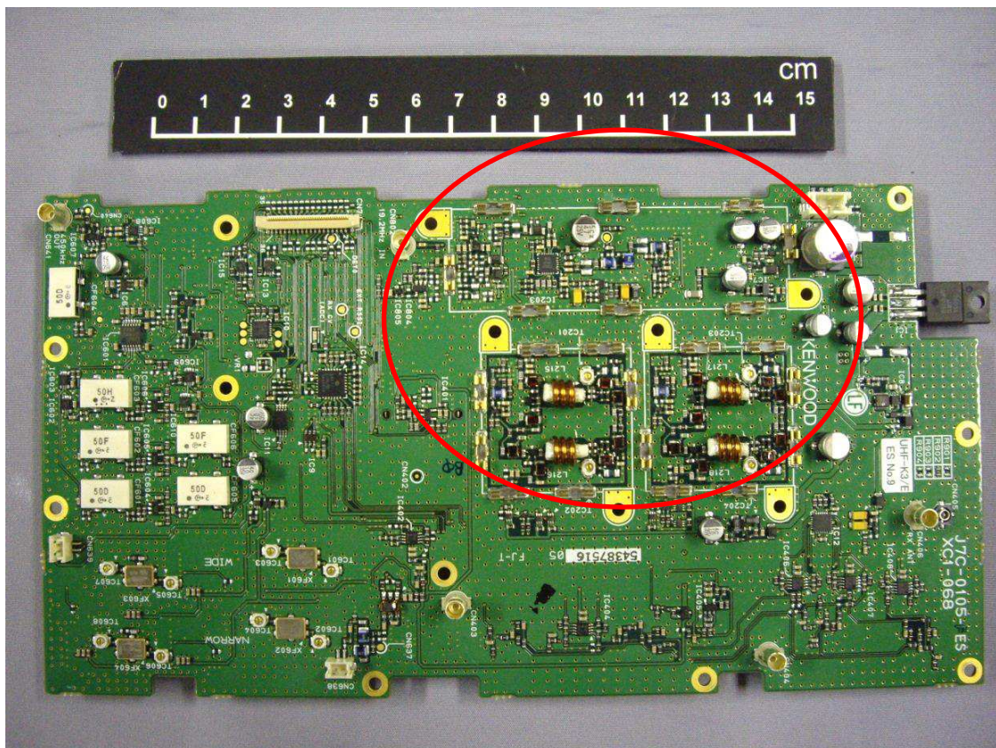
RX Upper Side View without Shield
