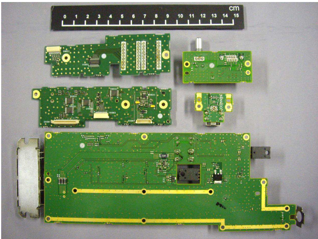
Final 1-5 Bottom Side View
