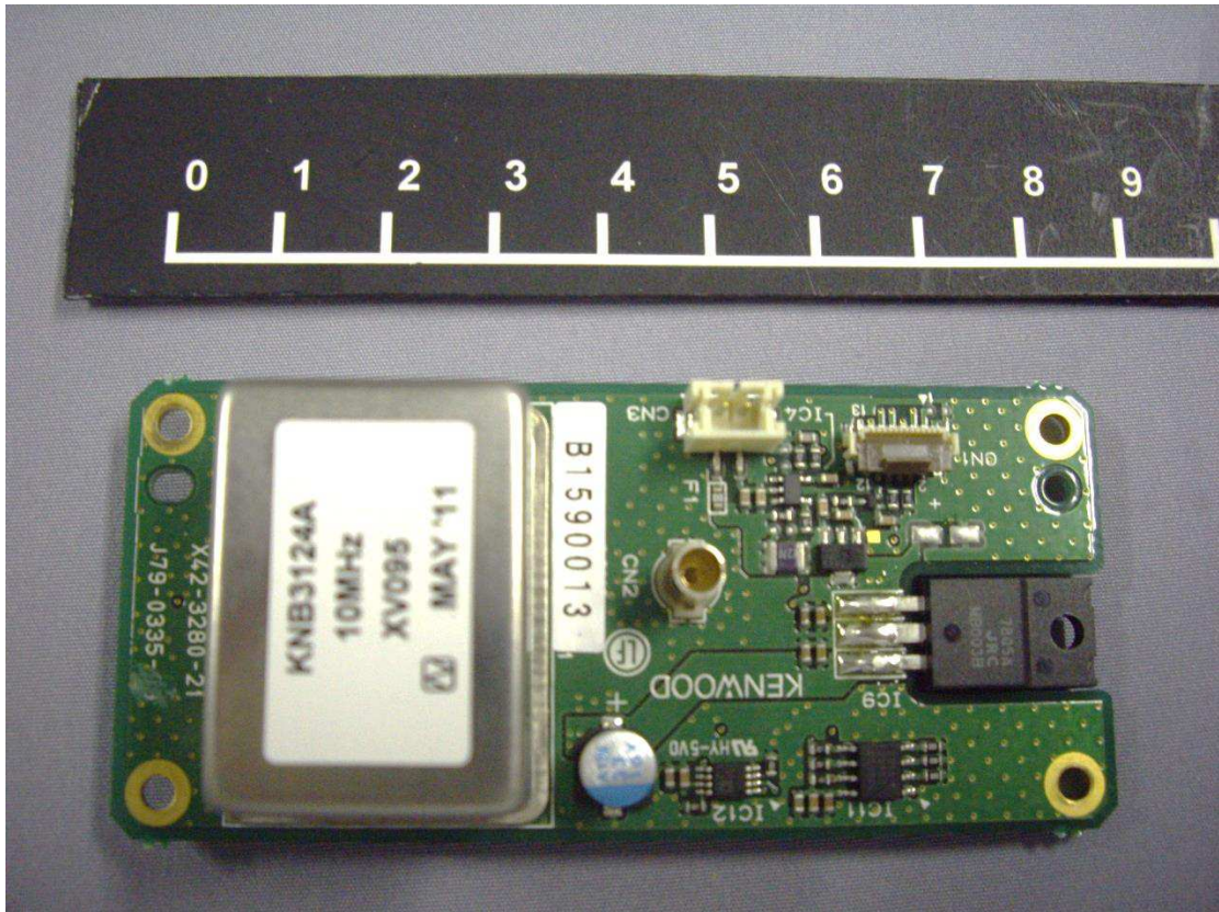
KXK-3 OCXO UNIT Upper Side View
