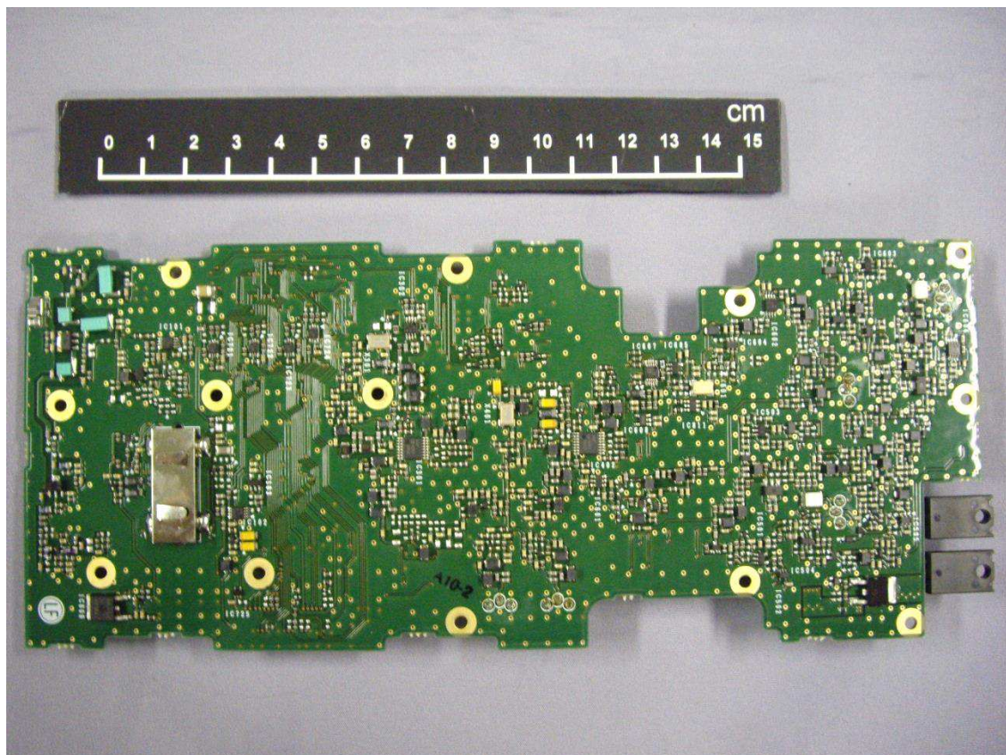
TX1 Bottom Side View
