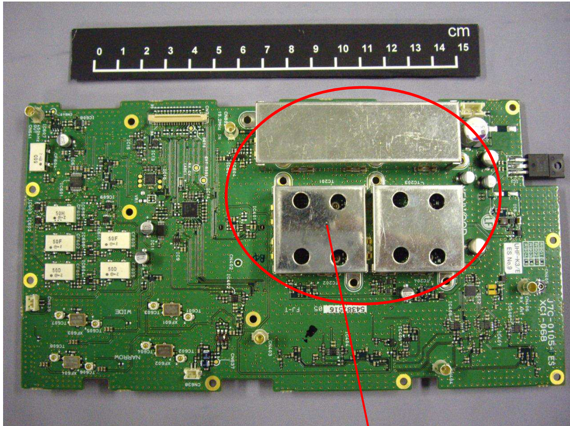
RX Upper Side View with Shield
