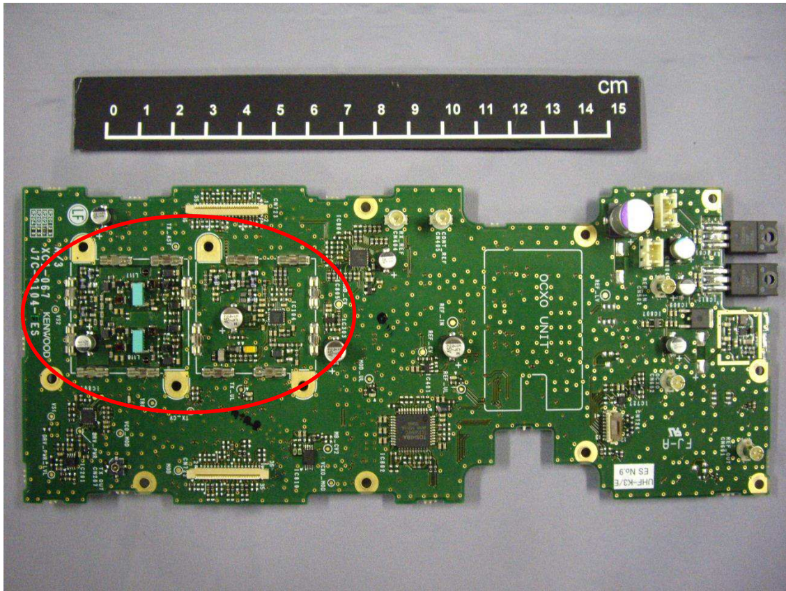
TX1 Upper Side View without Shield
