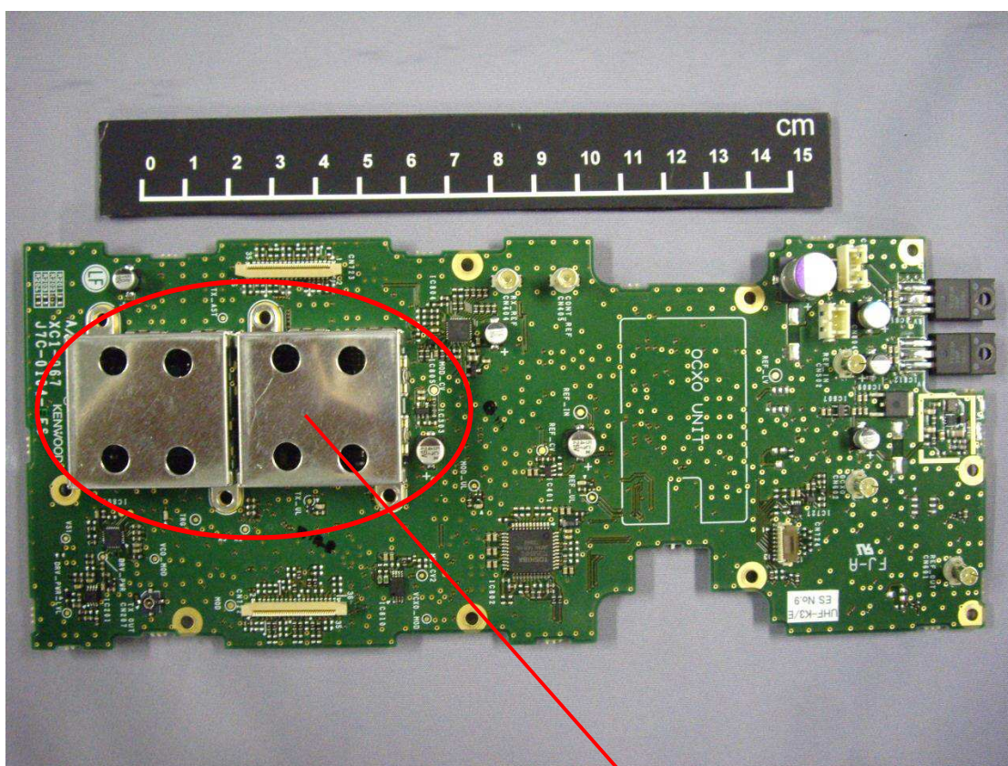
TX1 Upper Side View with Shield
