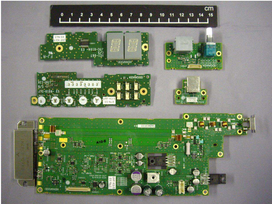
Final 1-5 Upper Side View
