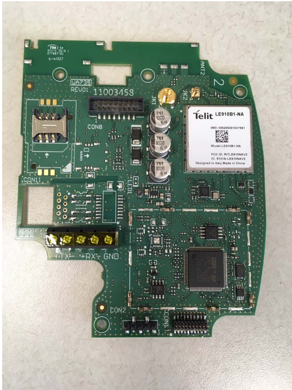
LE2077 (UA735 Rev. 01) PCB top side view (no shield)
