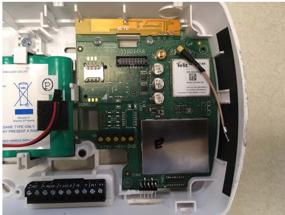
LE2077 (UA735 Rev. 01) PCB top side view (with shield)
