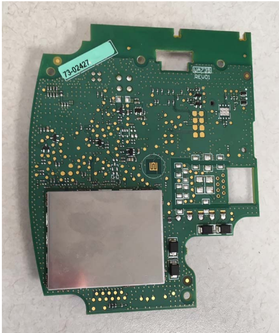
LE2077 (UA735 Rev. 01) PCB top side view (with shield)
