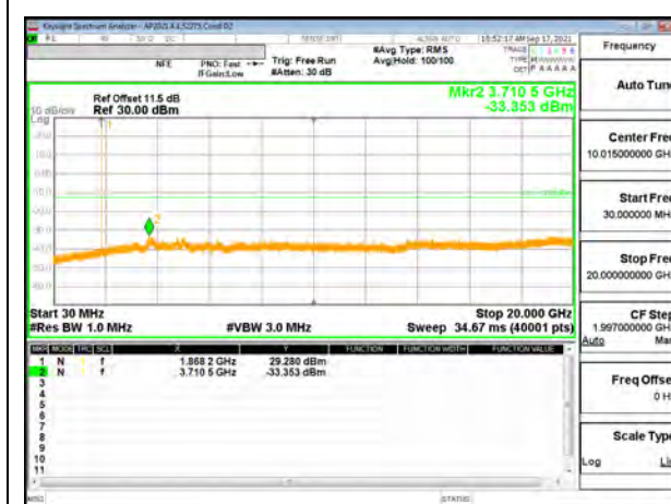
5G NR n25 30MHz BPSK Middle Channel RB1-1
