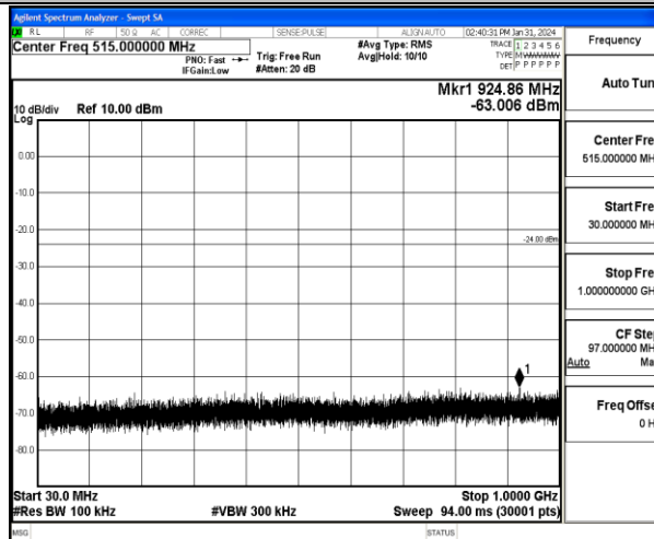
11N20MIMO-Ant1-2462-30~1000-PASS
