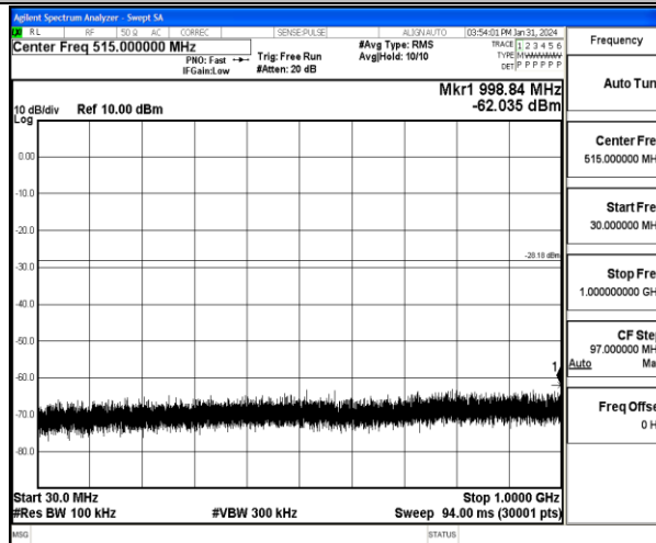
11N40MIMO-Ant1-2452-30~1000-PASS
