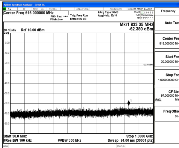
11G-Ant2-2437-30~1000-PASS
