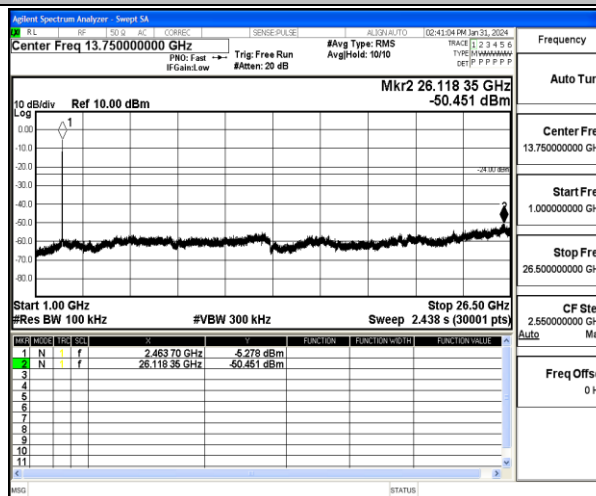
11N20MIMO-Ant1-2462-1000~26500-PASS
