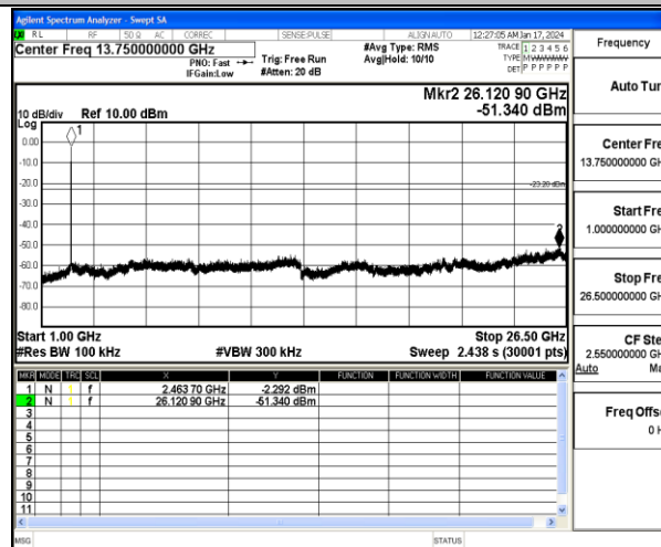
11G-Ant2-2462-1000~26500-PASS
