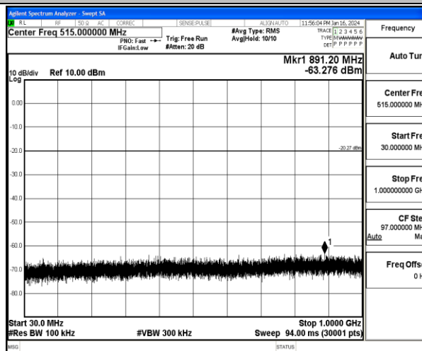
11G-Ant2-2412-30~1000-PASS
