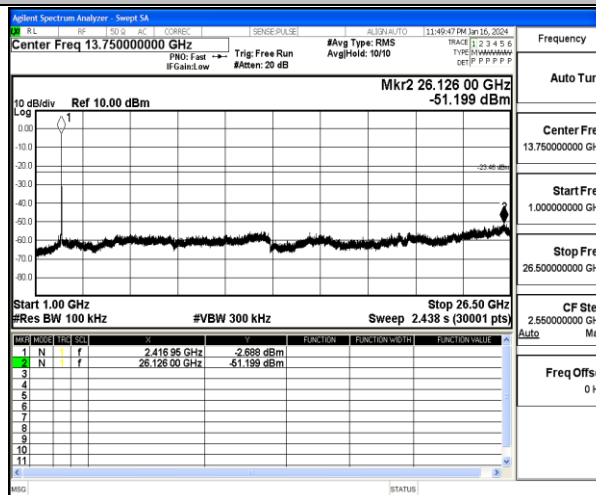
11G-Ant1-2412-1000~26500-PASS
