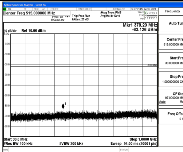
11N20MIMO-Ant2-2462-30~1000-PASS
