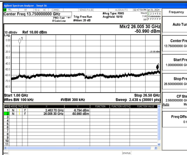
11N20MIMO-Ant2-2462-1000~26500-PASS
