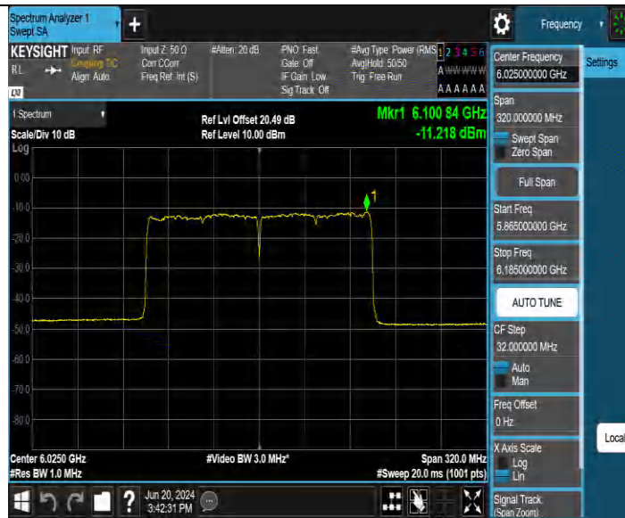
11AX160MIMO Ant3 6025
