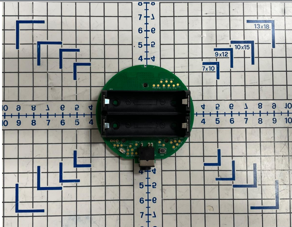
Mainboard View 2
