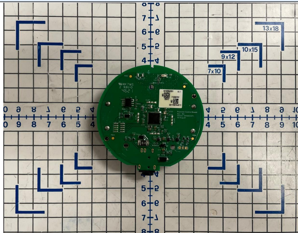
Mainboard View 2
