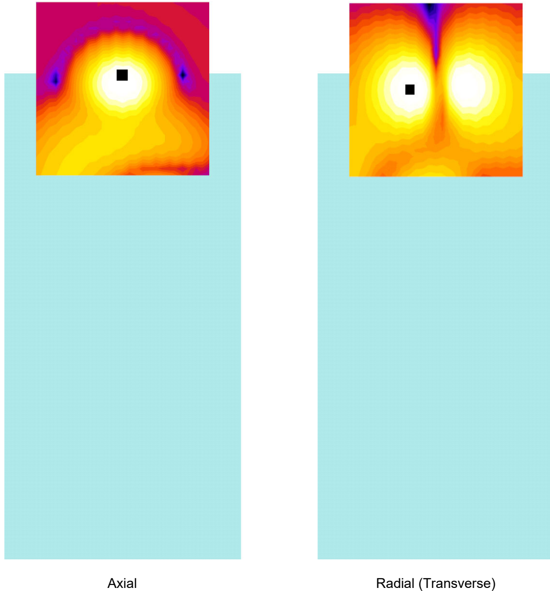
Figure 9-1 T-Coil Scan Overlay Magnetic Field Distributions
